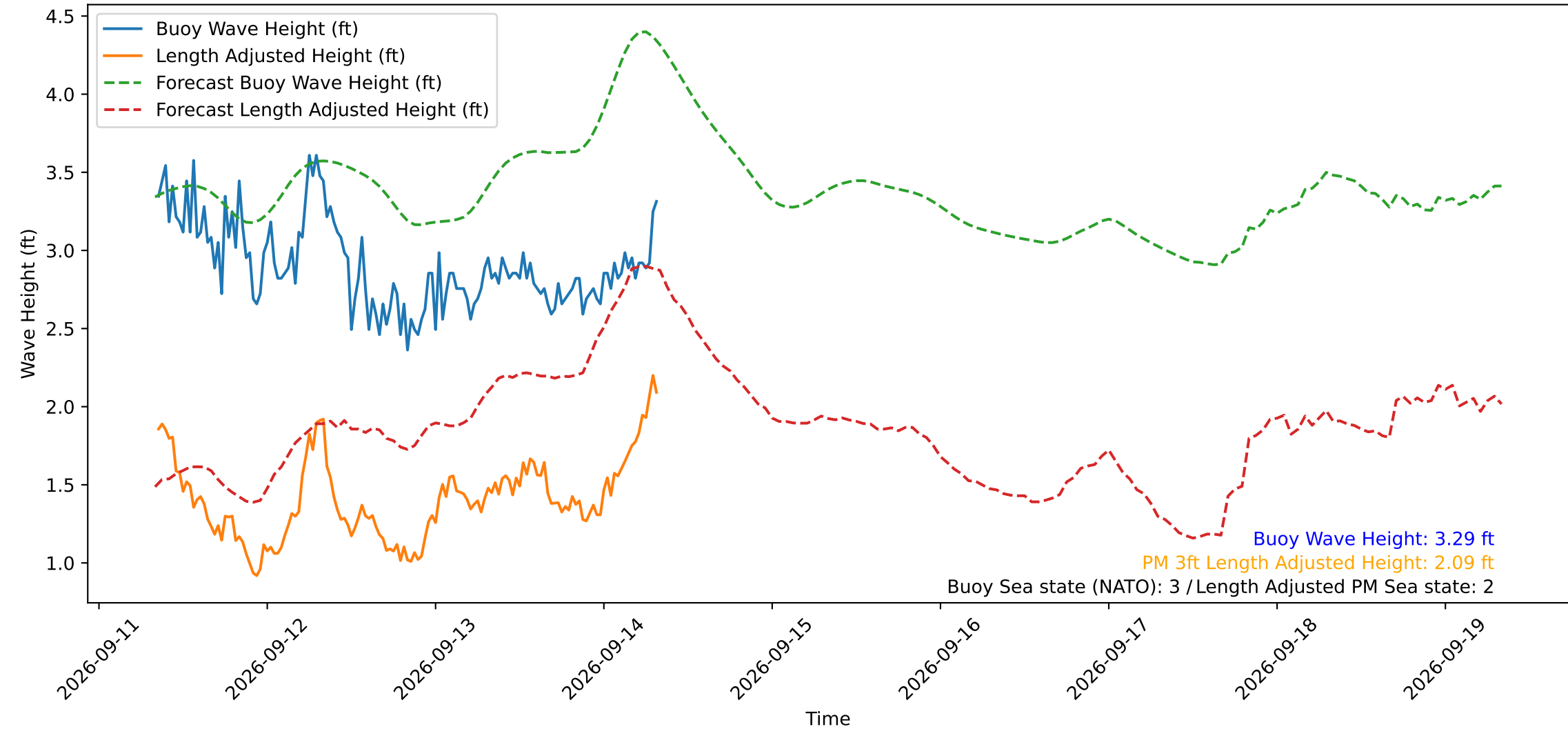
Wave Heights over Time for Green Beach at 2026-09-14 08:11:12
