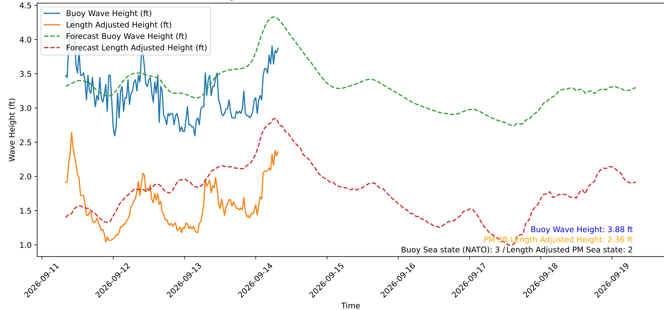
Wave Heights over Time for Oceanside Harbor at 2026-09-14 08:10:29
