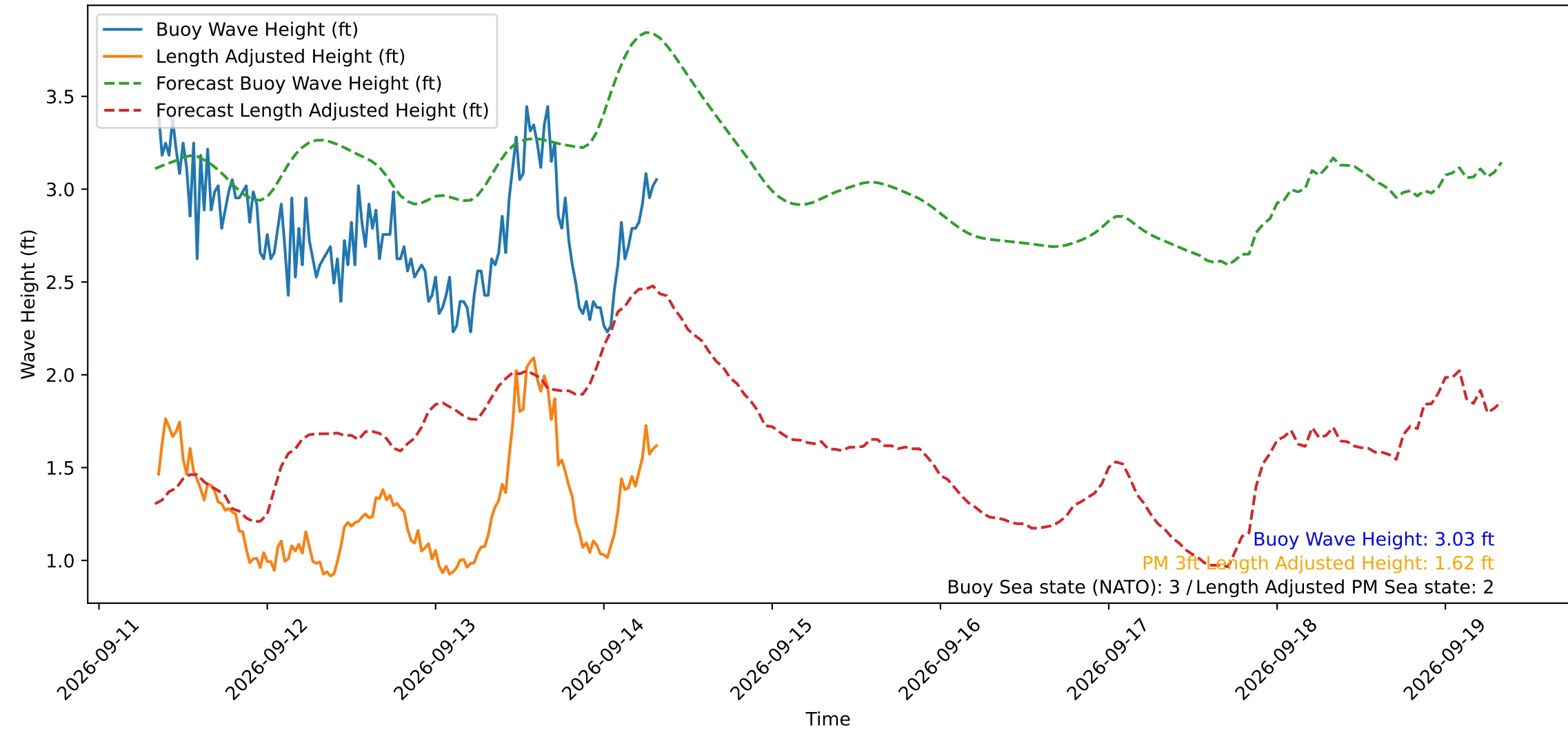
Wave Heights over Time for Red Beach at 2026-09-14 08:10:49
