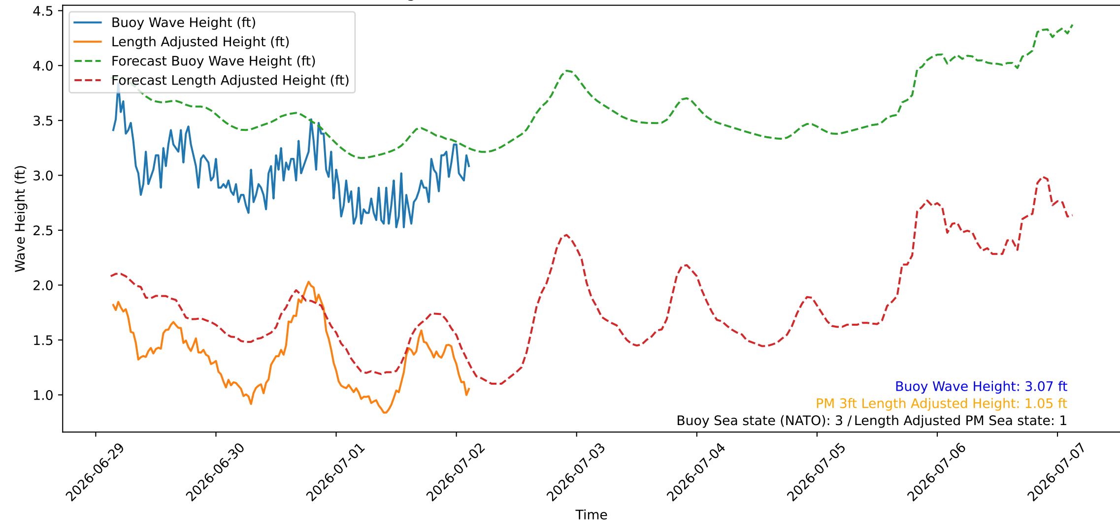
Wave Heights over Time for Green Beach at 2026-07-02 03:21:09
