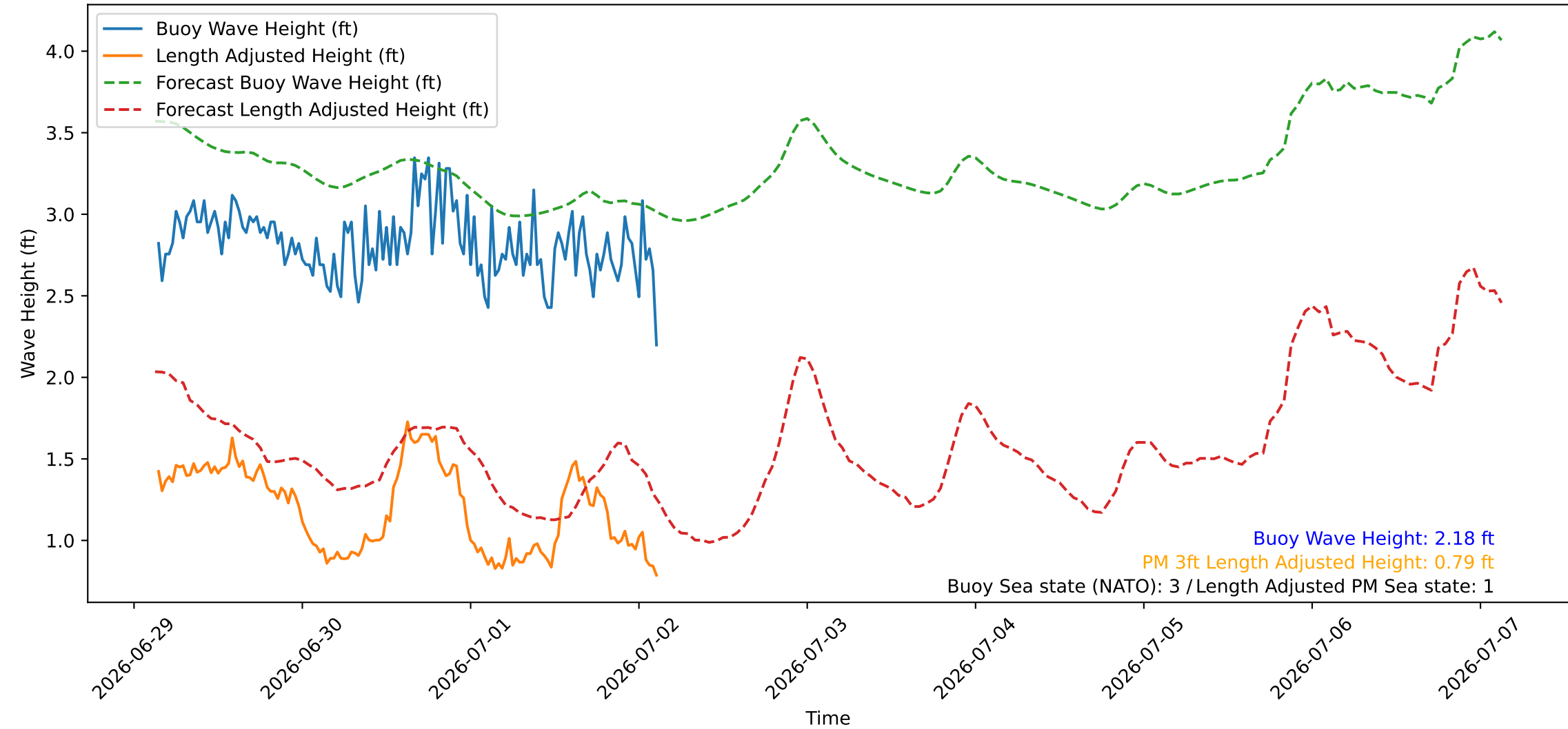
Wave Heights over Time for Red Beach at 2026-07-02 03:20:47
