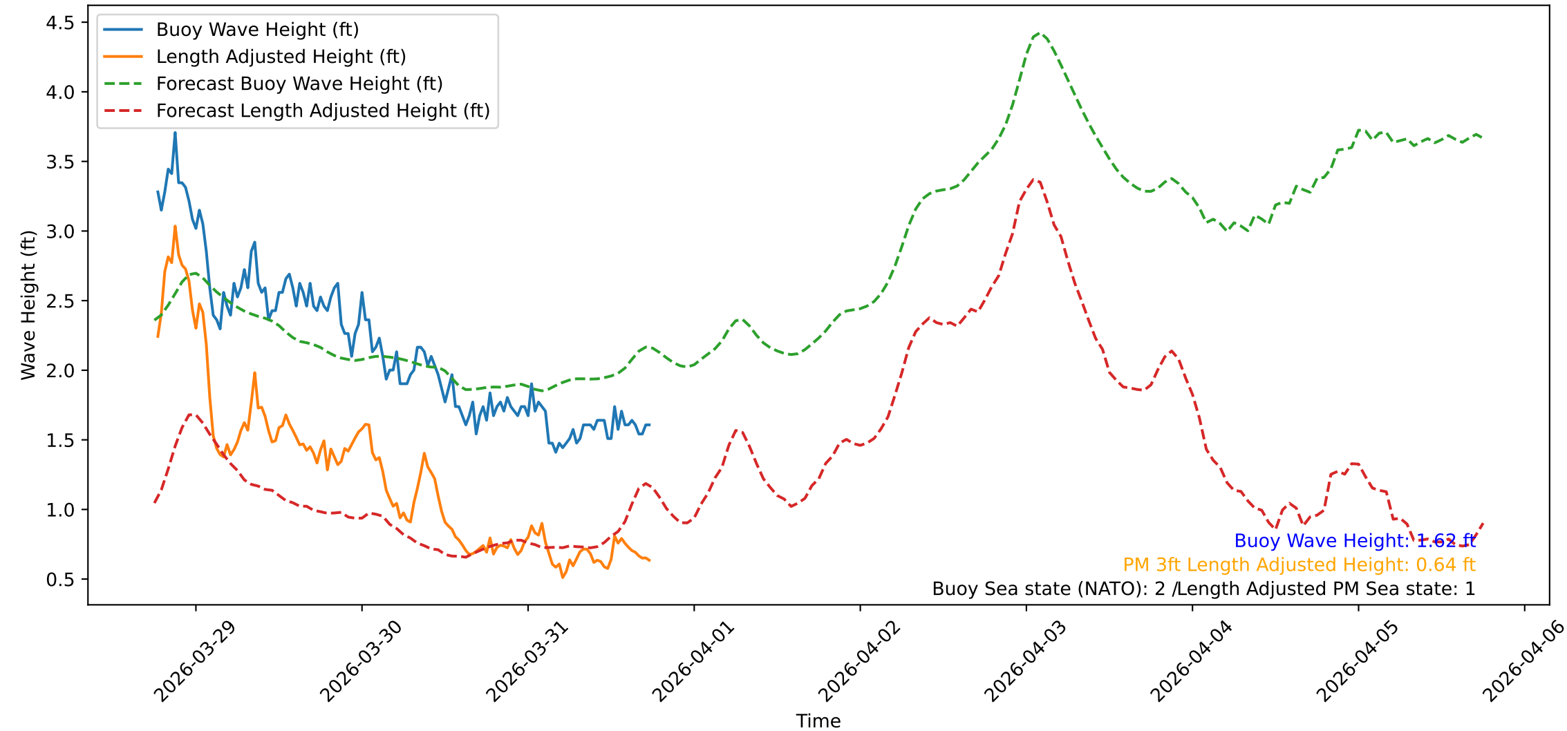
Wave Heights over Time for Green Beach at 2026-03-31 18:21:11
