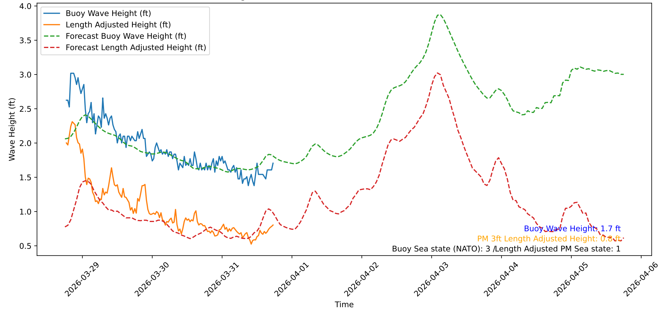
Wave Heights over Time for Red Beach at 2026-03-31 18:20:49
