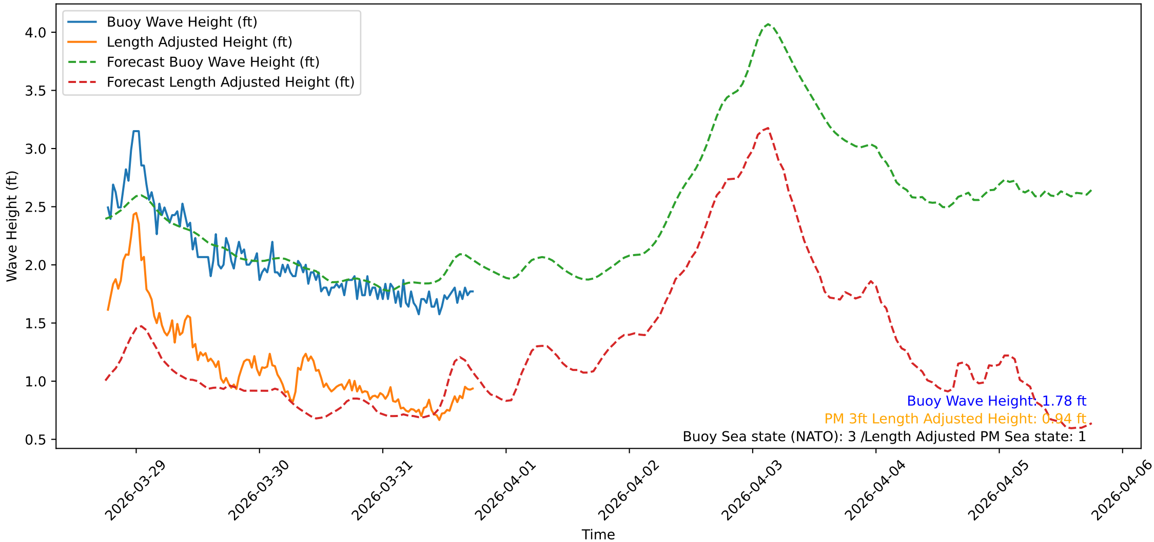
Wave Heights over Time for Oceanside Harbor at 2026-03-31 18:20:32
