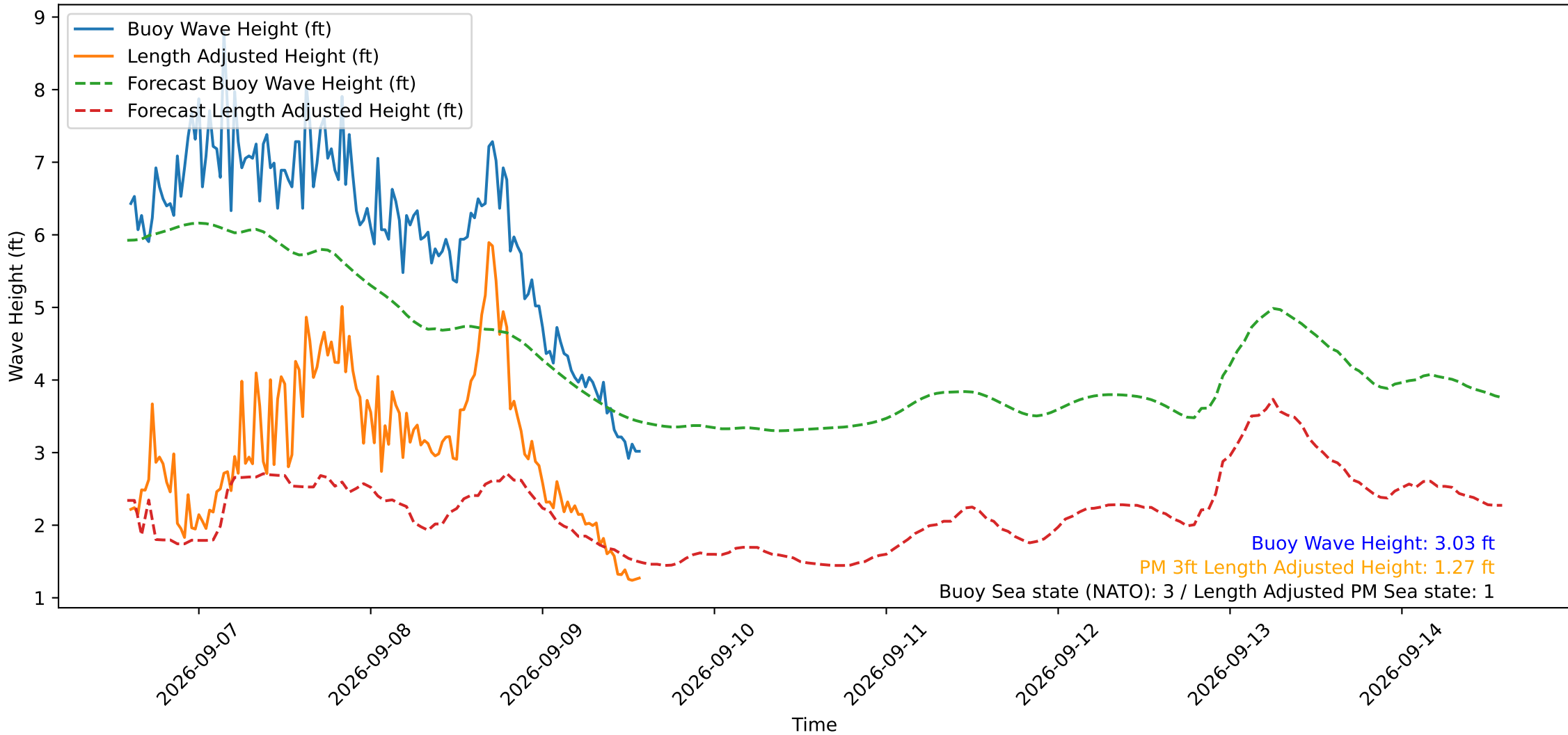
Wave Heights over Time for Green Beach at 2026-09-09 14:11:11
