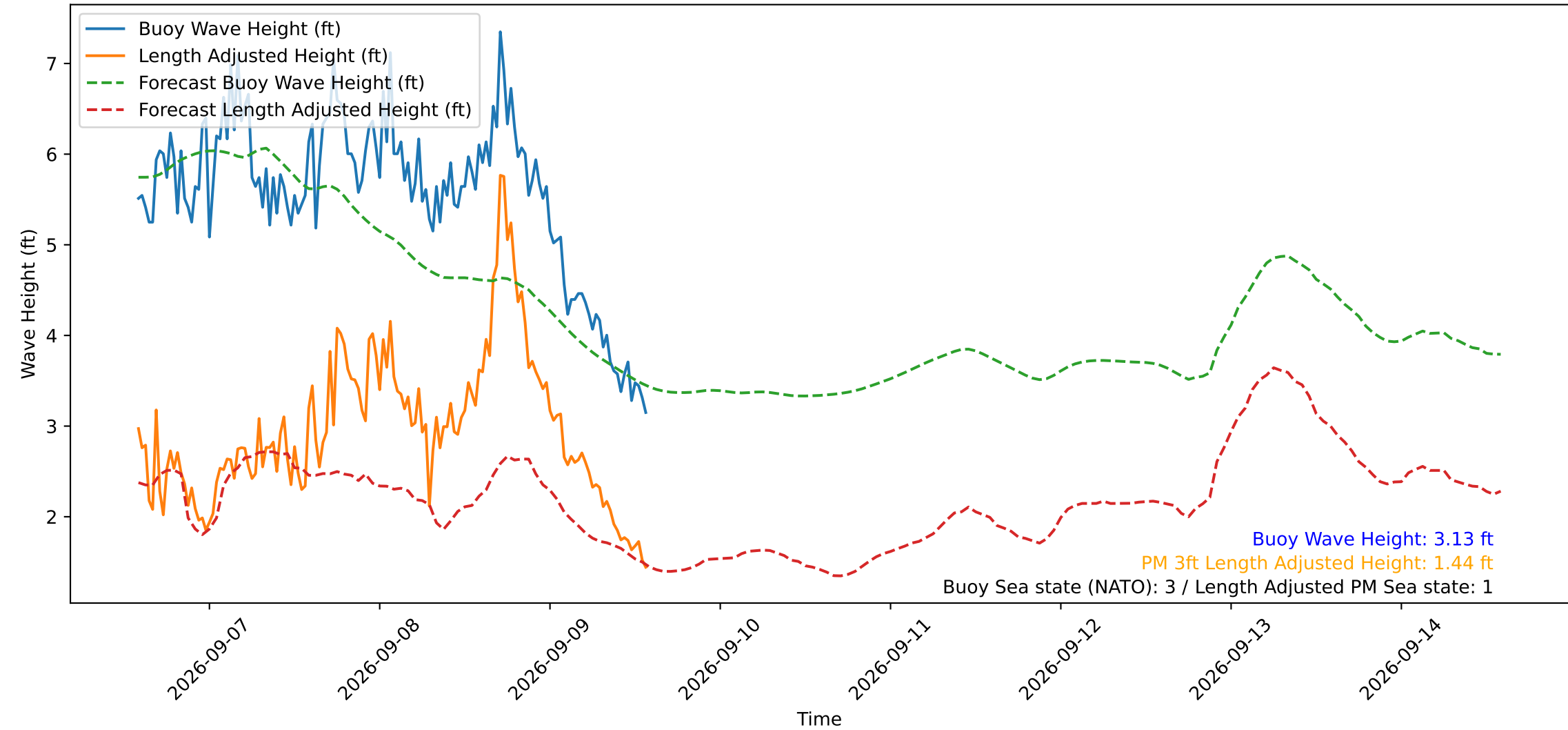
Wave Heights over Time for Oceanside Harbor at 2026-09-09 14:10:29
