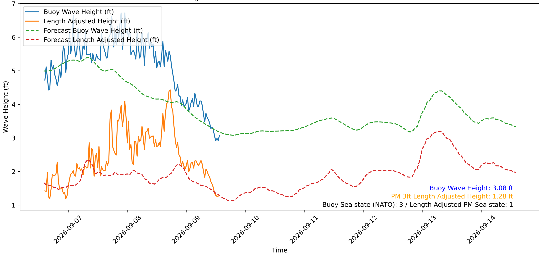
Wave Heights over Time for Red Beach at 2026-09-09 14:10:48
