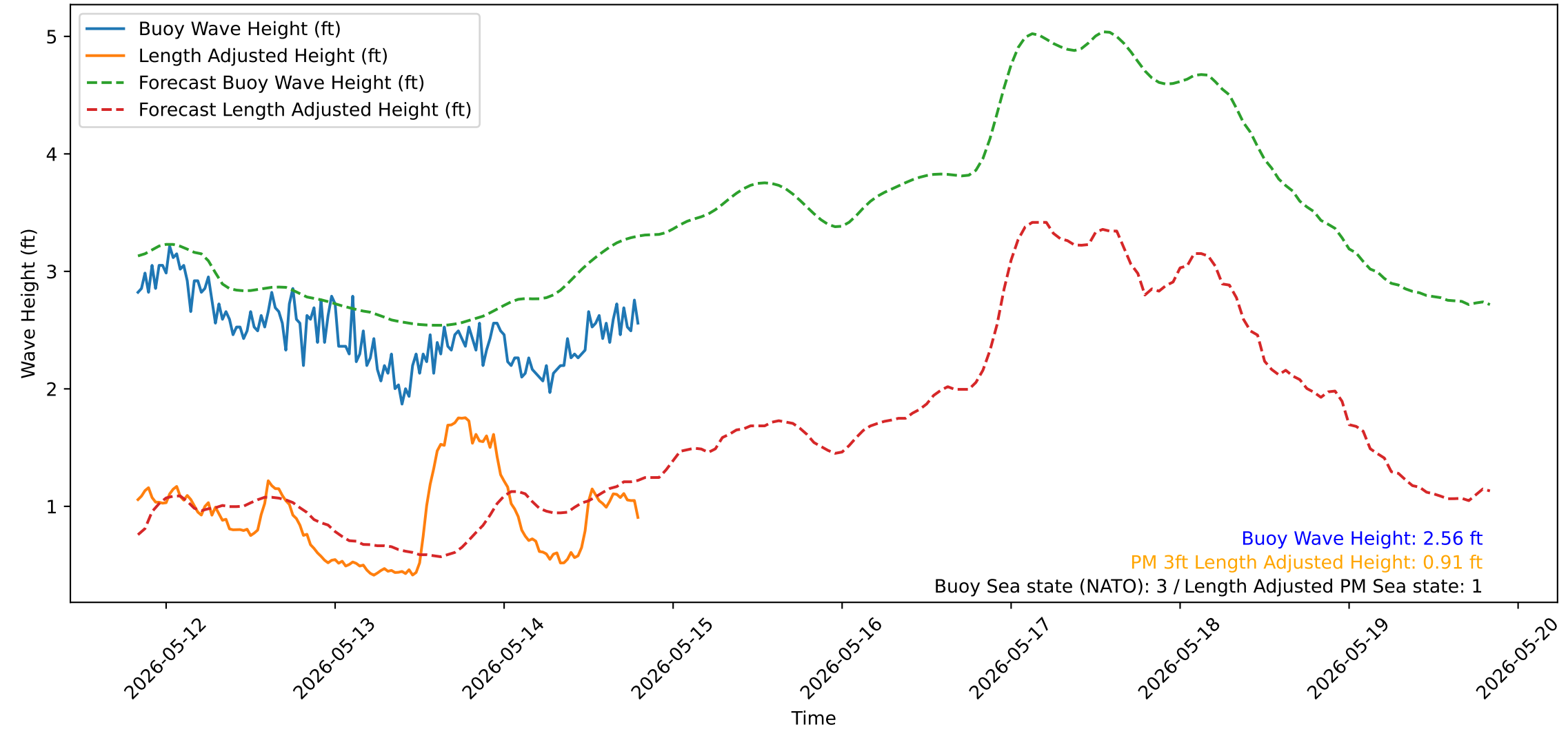
Wave Heights over Time for Red Beach at 2026-05-14 19:40:51
