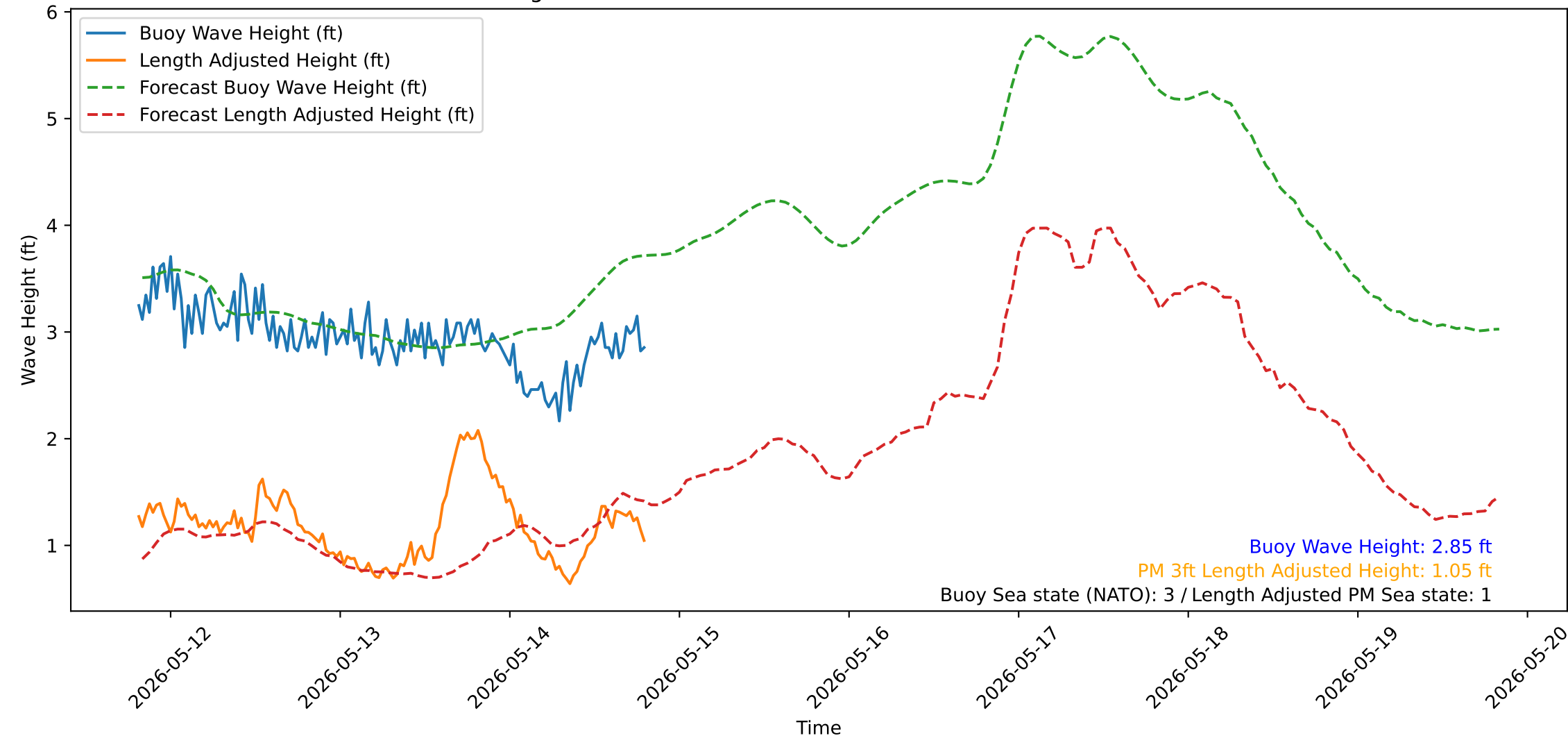
Wave Heights over Time for Oceanside Harbor at 2026-05-14 19:40:32
