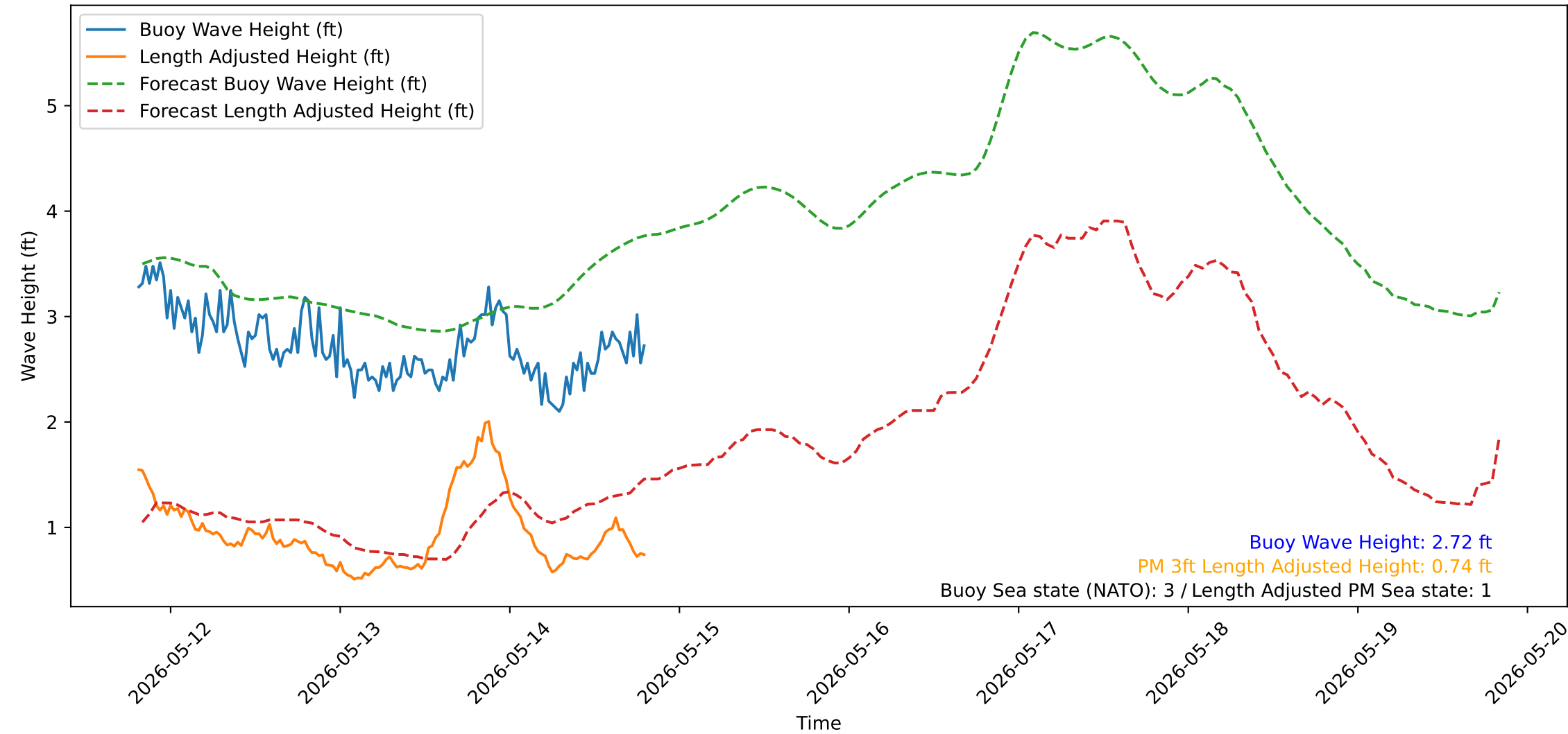
Wave Heights over Time for Green Beach at 2026-05-14 19:41:14
