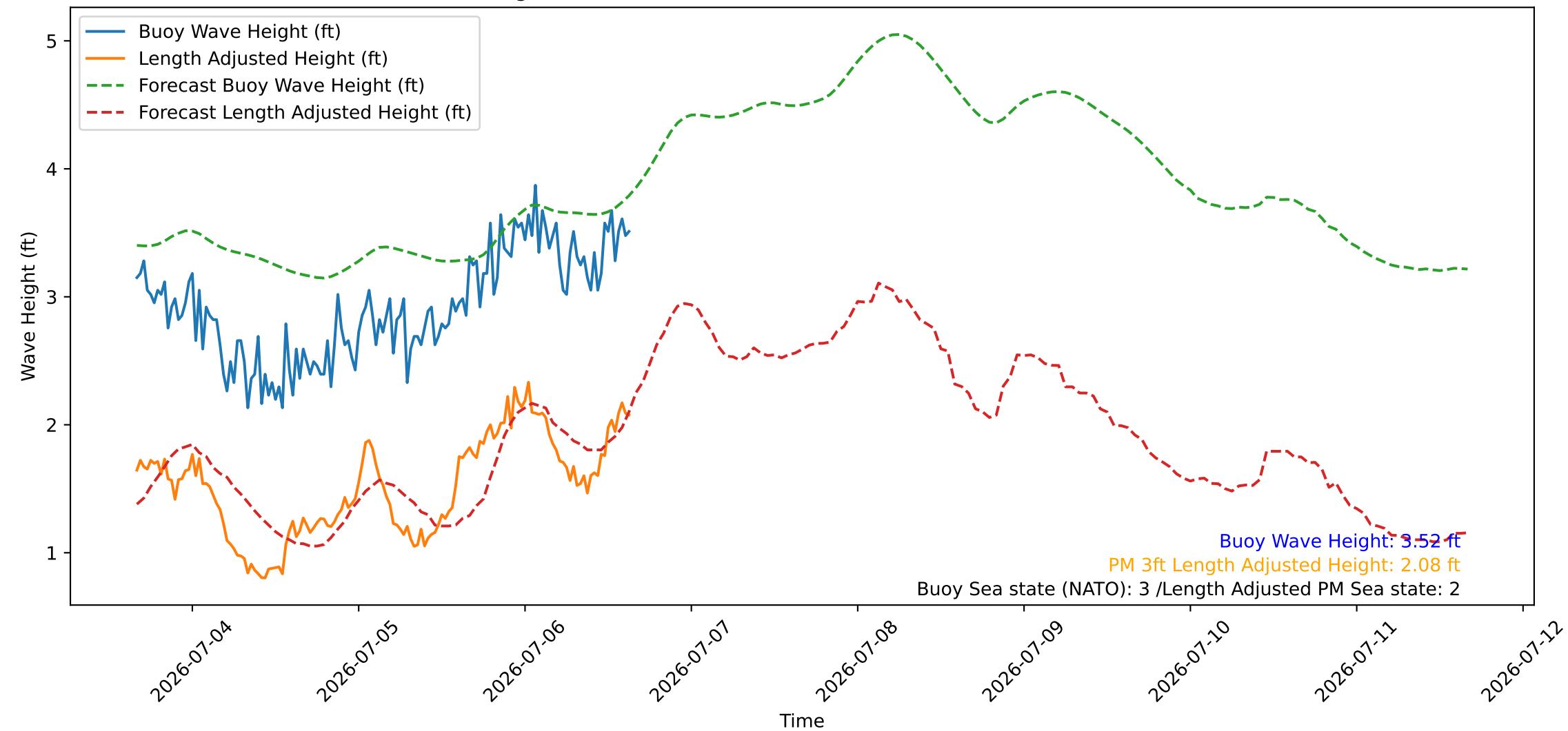
Wave Heights over Time for Oceanside Harbor at 2026-07-06 16:00:26
