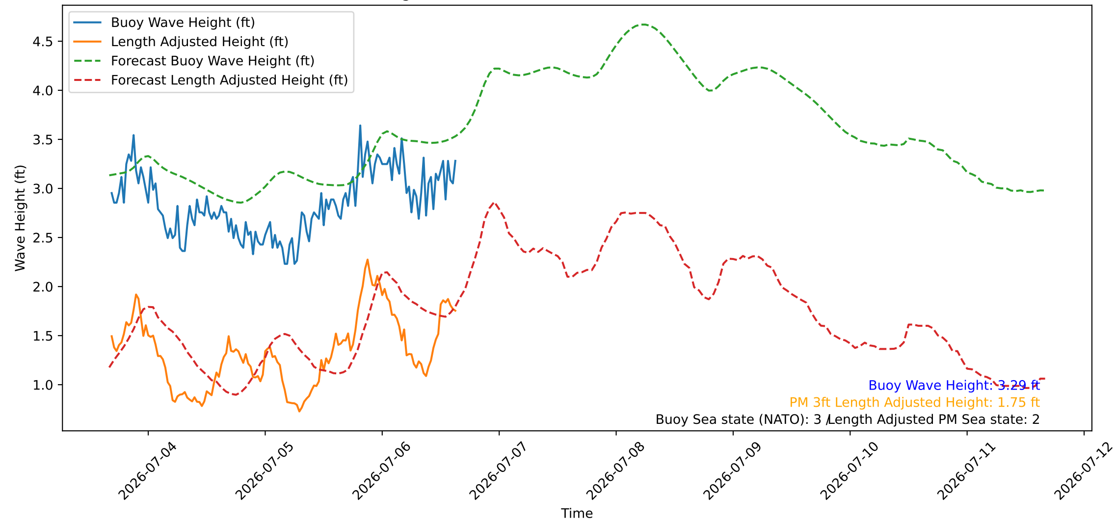
Wave Heights over Time for Red Beach at 2026-07-06 16:00:46
