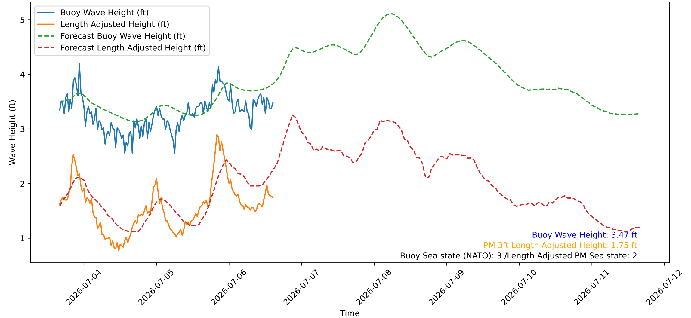
Wave Heights over Time for Green Beach at 2026-07-06 16:01:08
