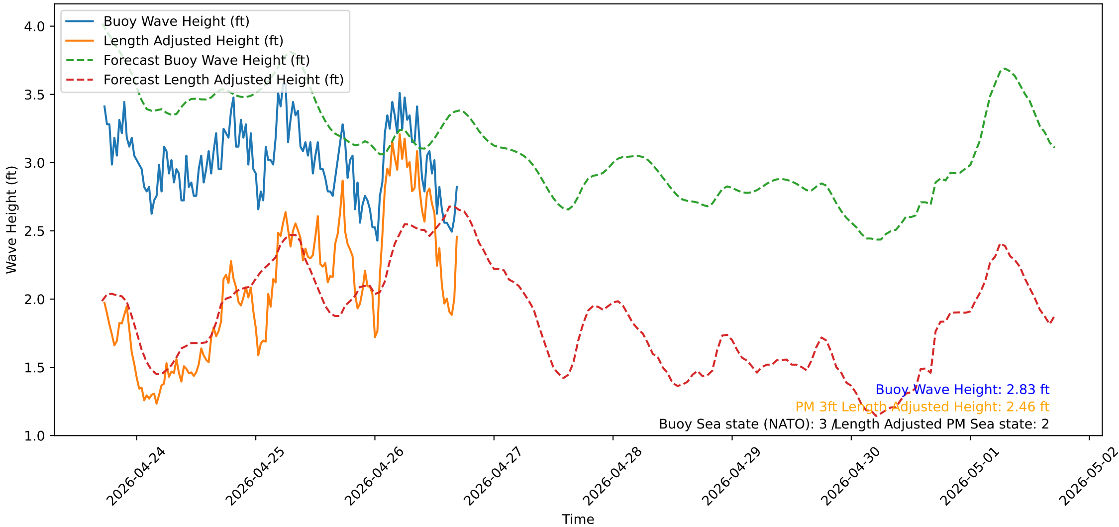
Wave Heights over Time for Green Beach at 2026-04-26 17:21:13
