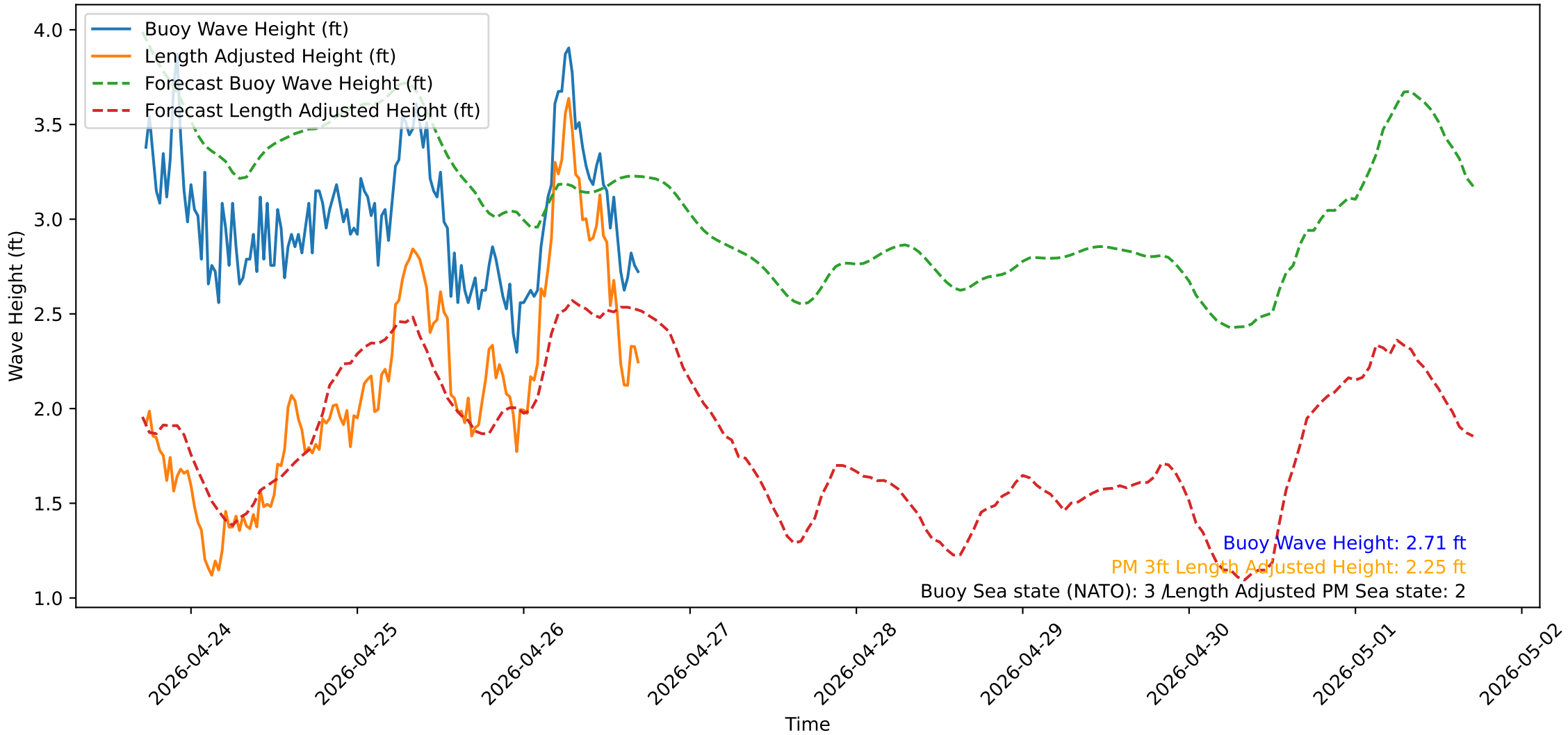
Wave Heights over Time for Oceanside Harbor at 2026-04-26 17:20:31
