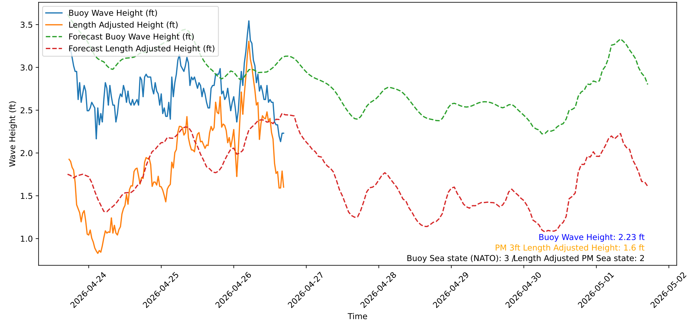
Wave Heights over Time for Red Beach at 2026-04-26 17:20:51
