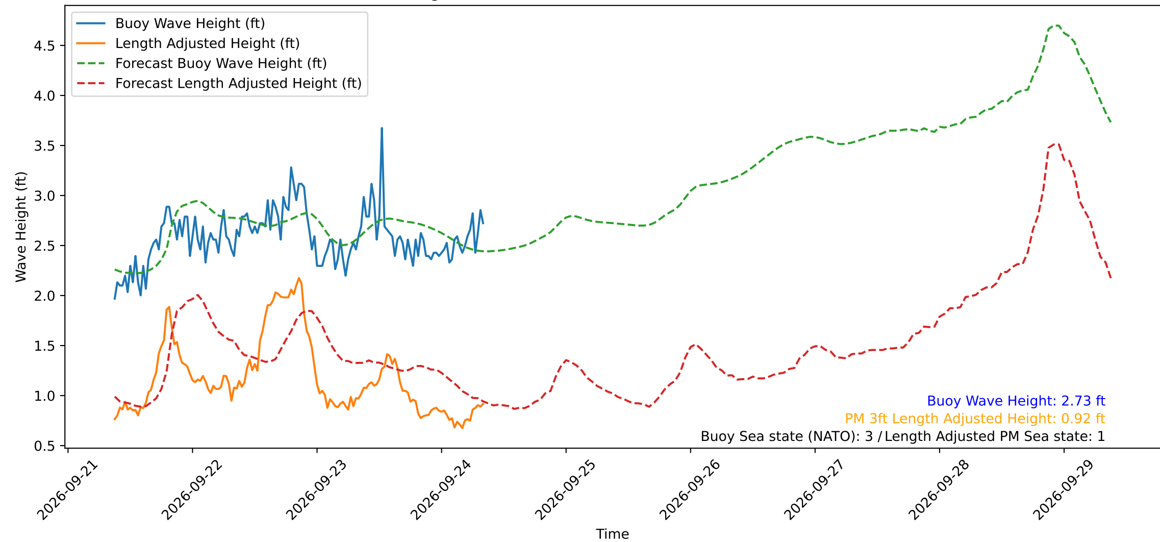
Wave Heights over Time for Red Beach at 2026-09-24 08:50:51
