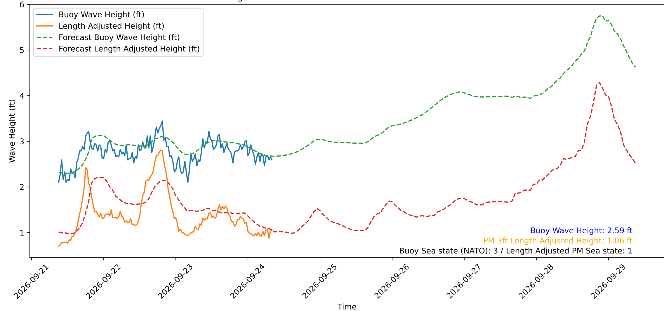
Wave Heights over Time for Green Beach at 2026-09-24 08:51:15
