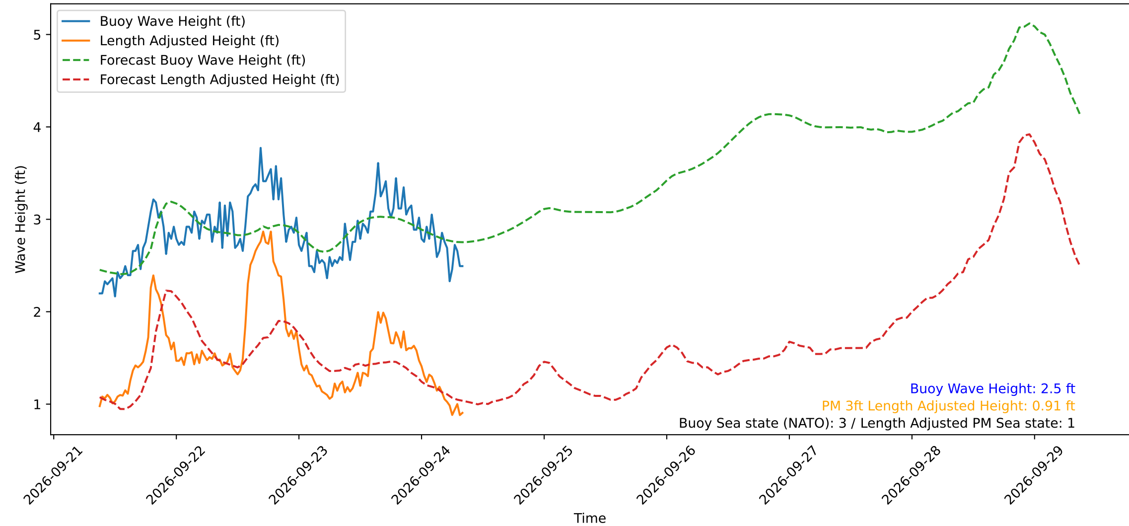
Wave Heights over Time for Oceanside Harbor at 2026-09-24 08:50:30
