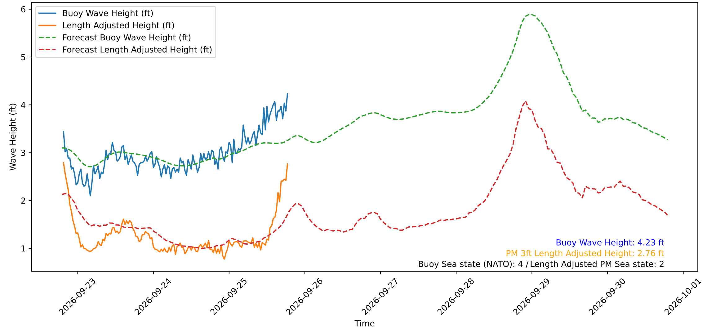
Wave Heights over Time for Green Beach at 2026-09-25 19:11:12
