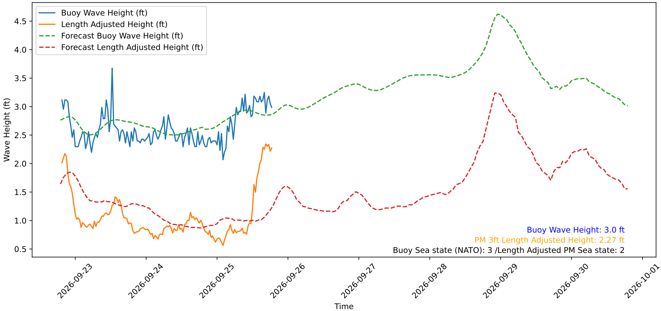
Wave Heights over Time for Red Beach at 2026-09-25 19:10:49
