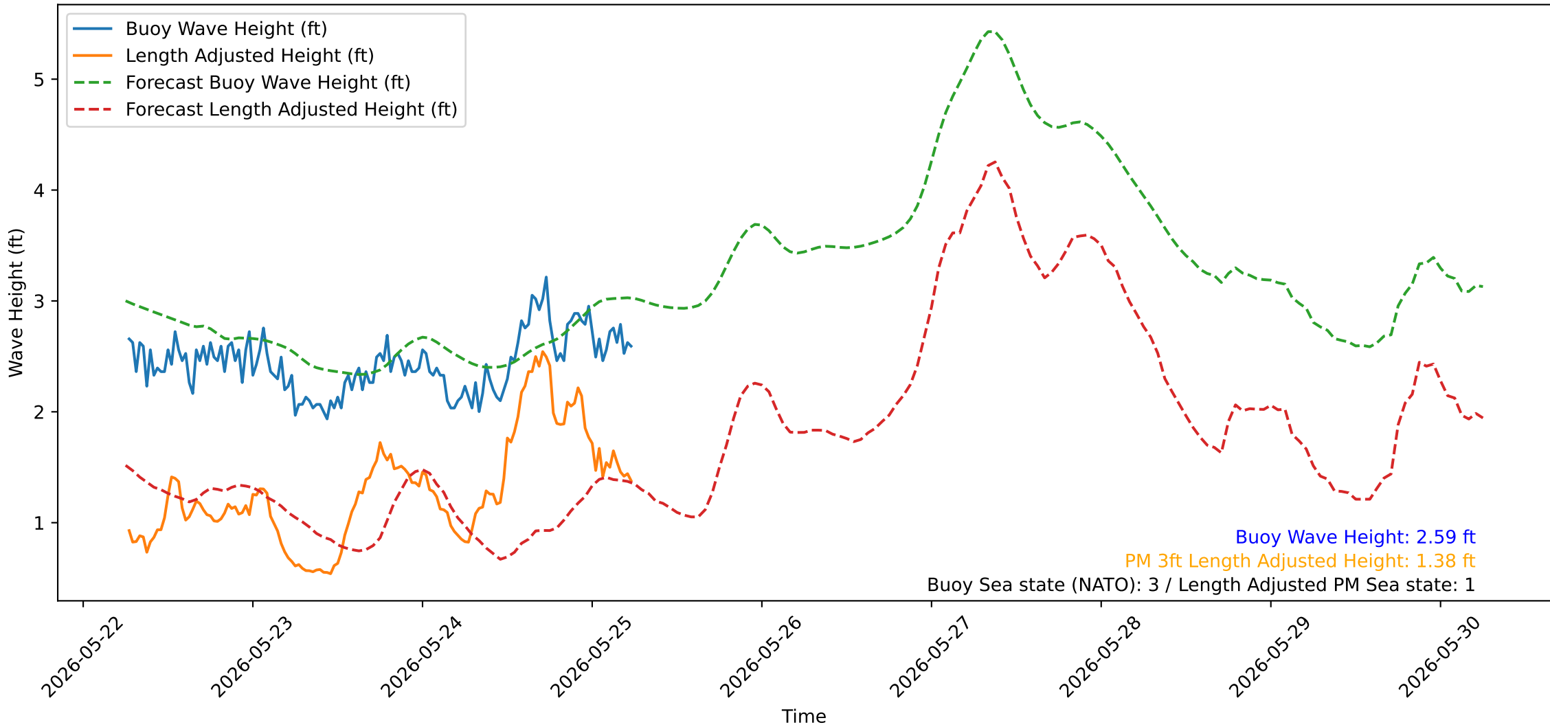
Wave Heights over Time for Red Beach at 2026-05-25 06:20:52
