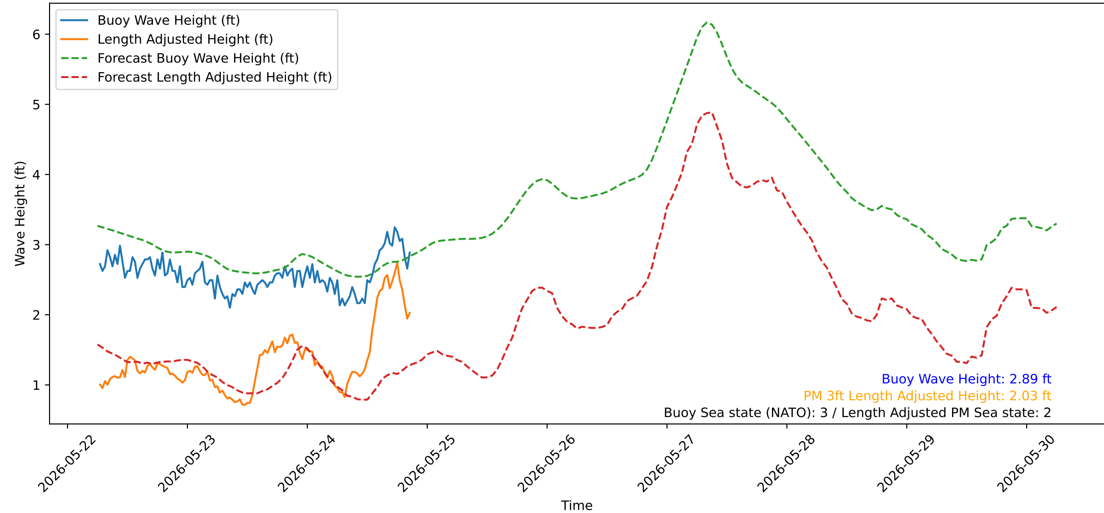
Wave Heights over Time for Oceanside Harbor at 2026-05-25 06:20:31
