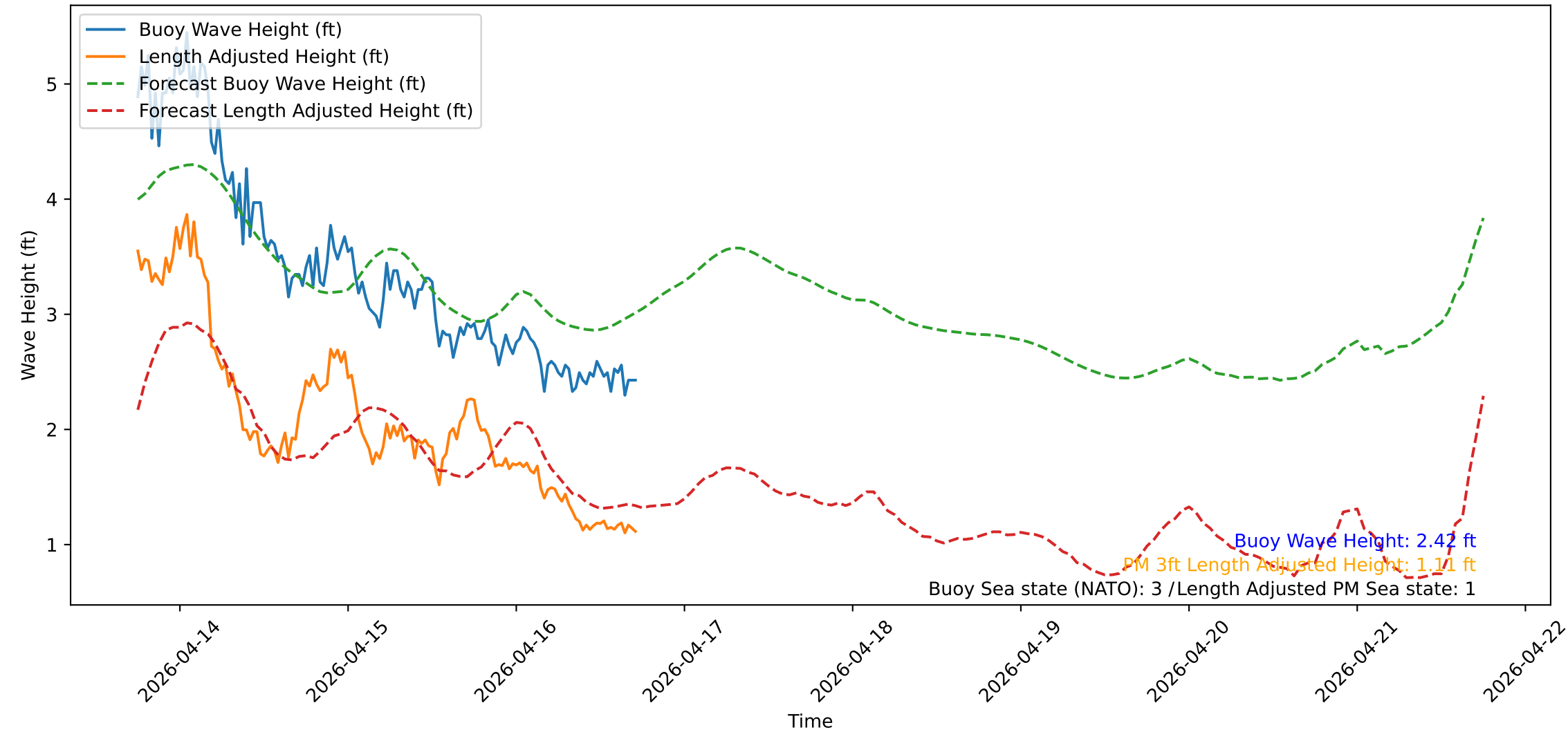
Wave Heights over Time for Oceanside Harbor at 2026-04-16 18:00:32
