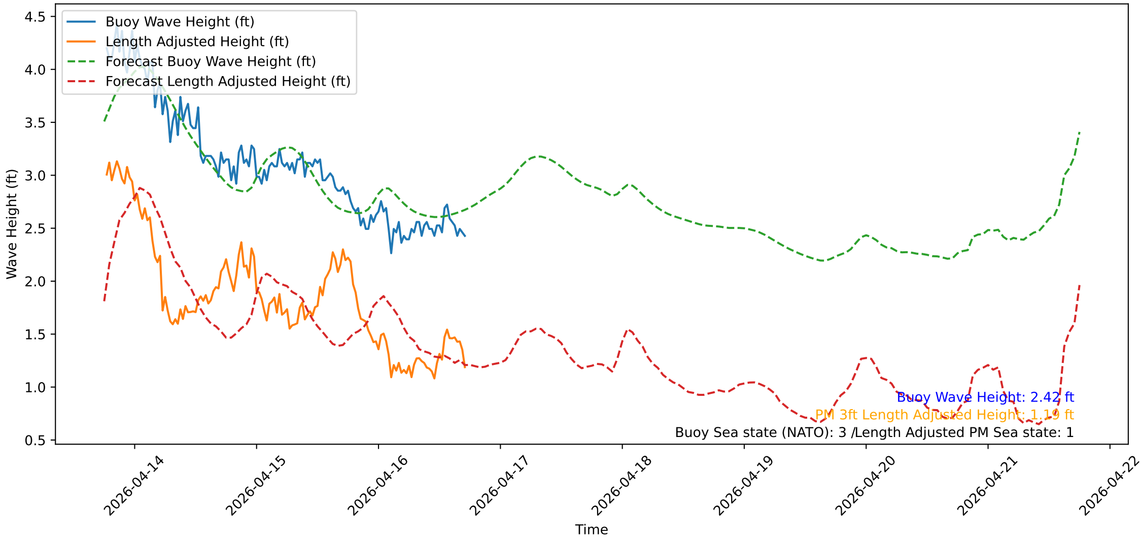
Wave Heights over Time for Red Beach at 2026-04-16 18:00:51
