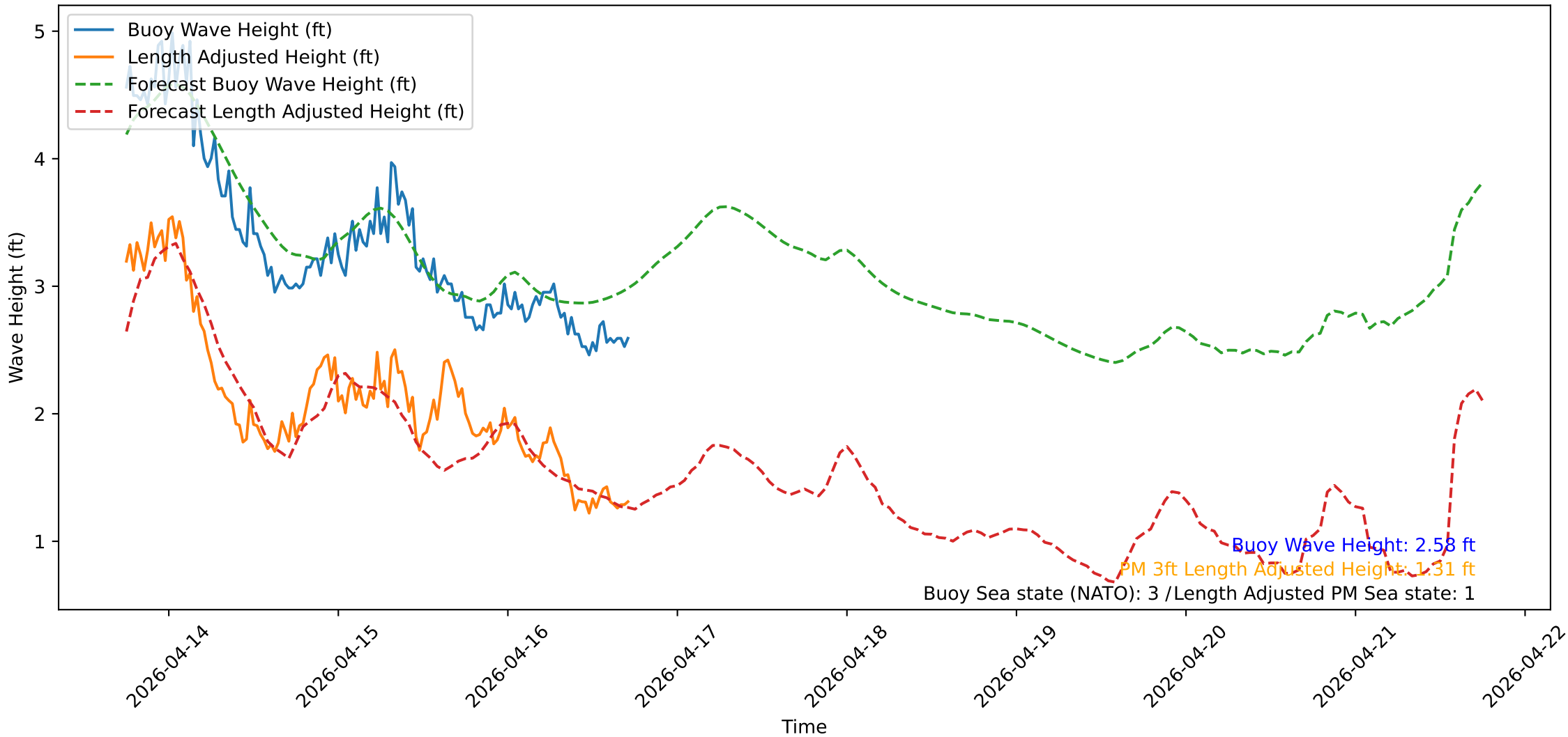
Wave Heights over Time for Green Beach at 2026-04-16 18:01:13
