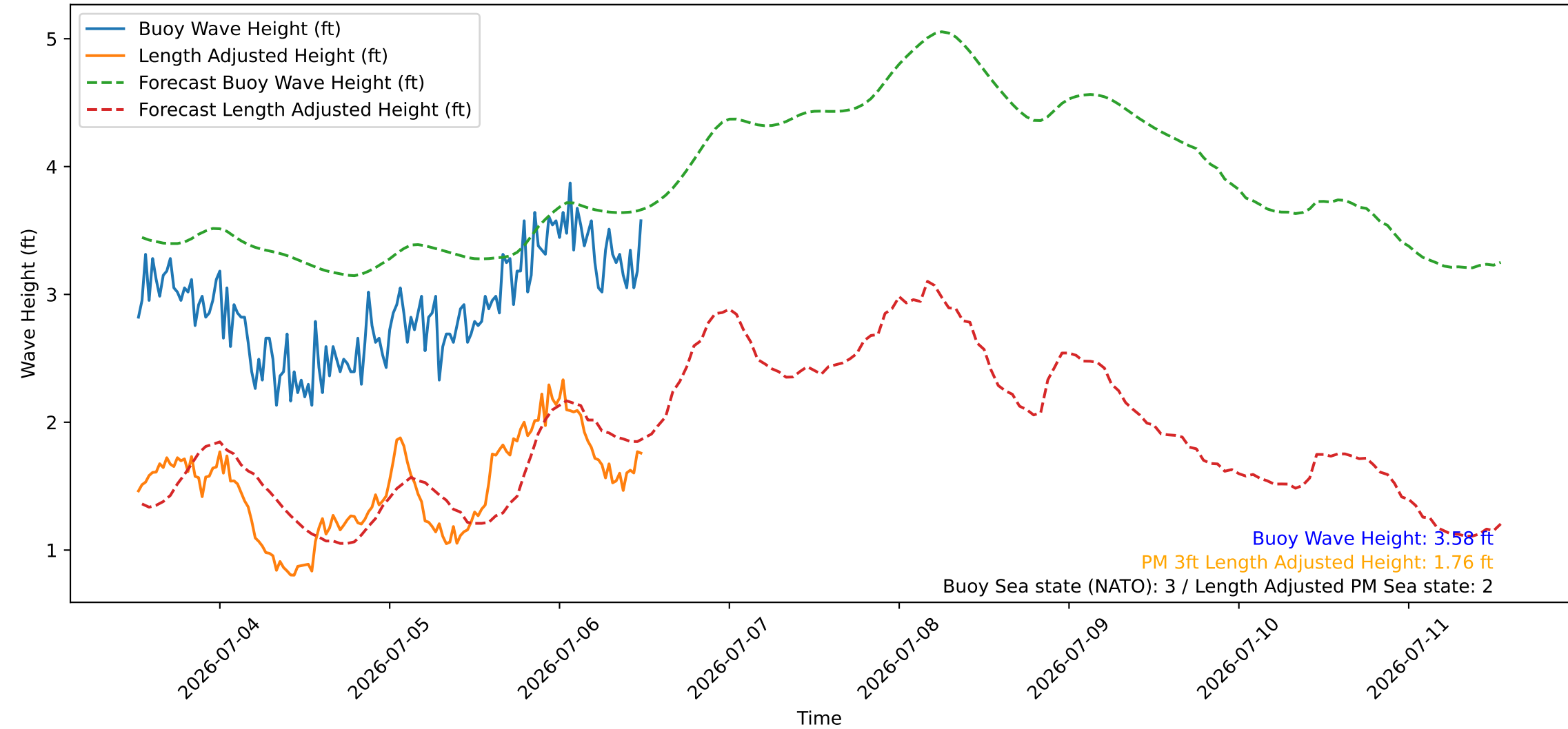
Wave Heights over Time for Oceanside Harbor at 2026-07-06 12:30:26
