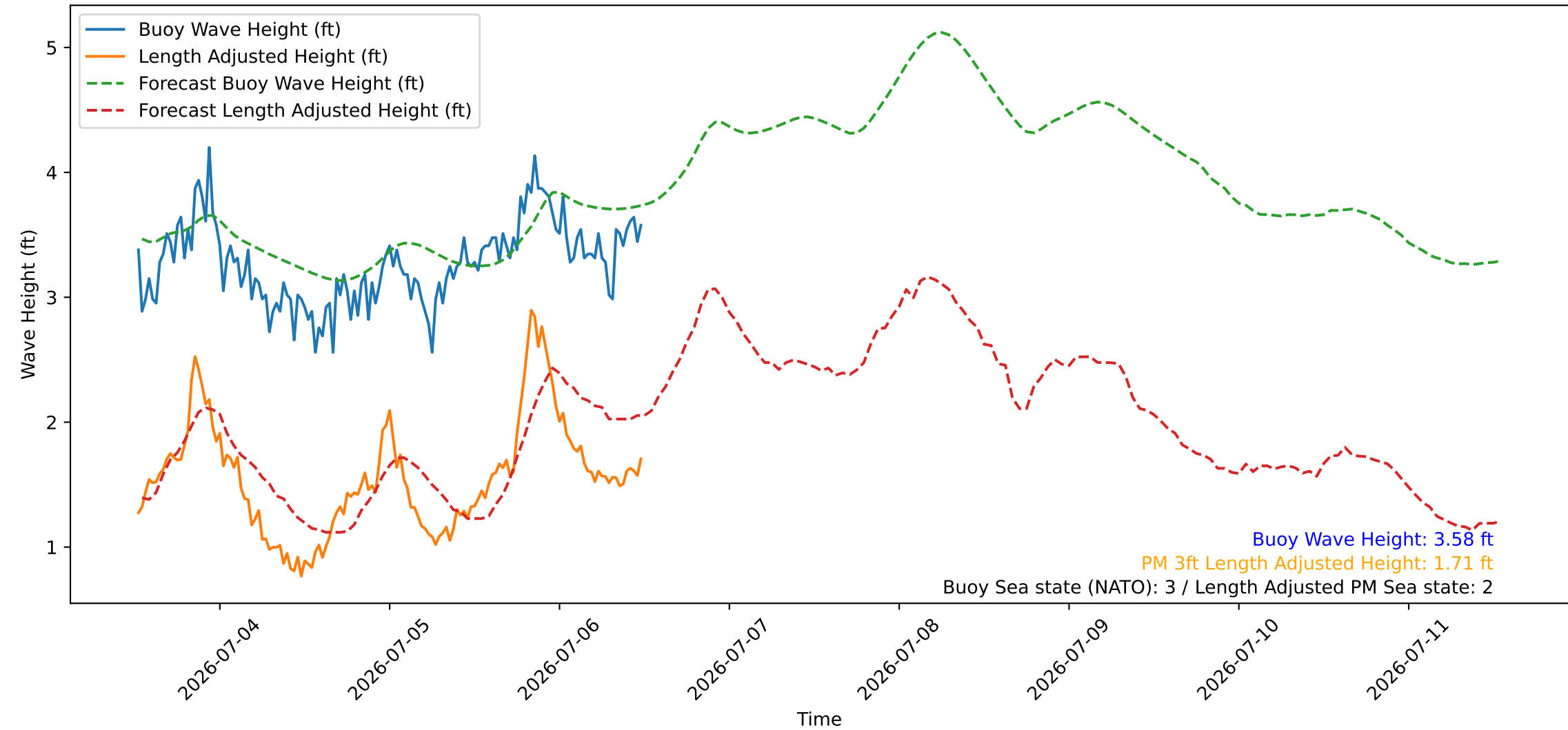
Wave Heights over Time for Green Beach at 2026-07-06 12:31:08
