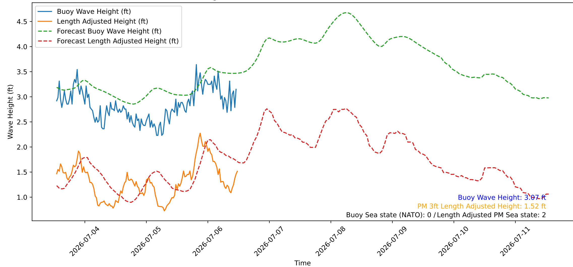
Wave Heights over Time for Red Beach at 2026-07-06 12:30:45
