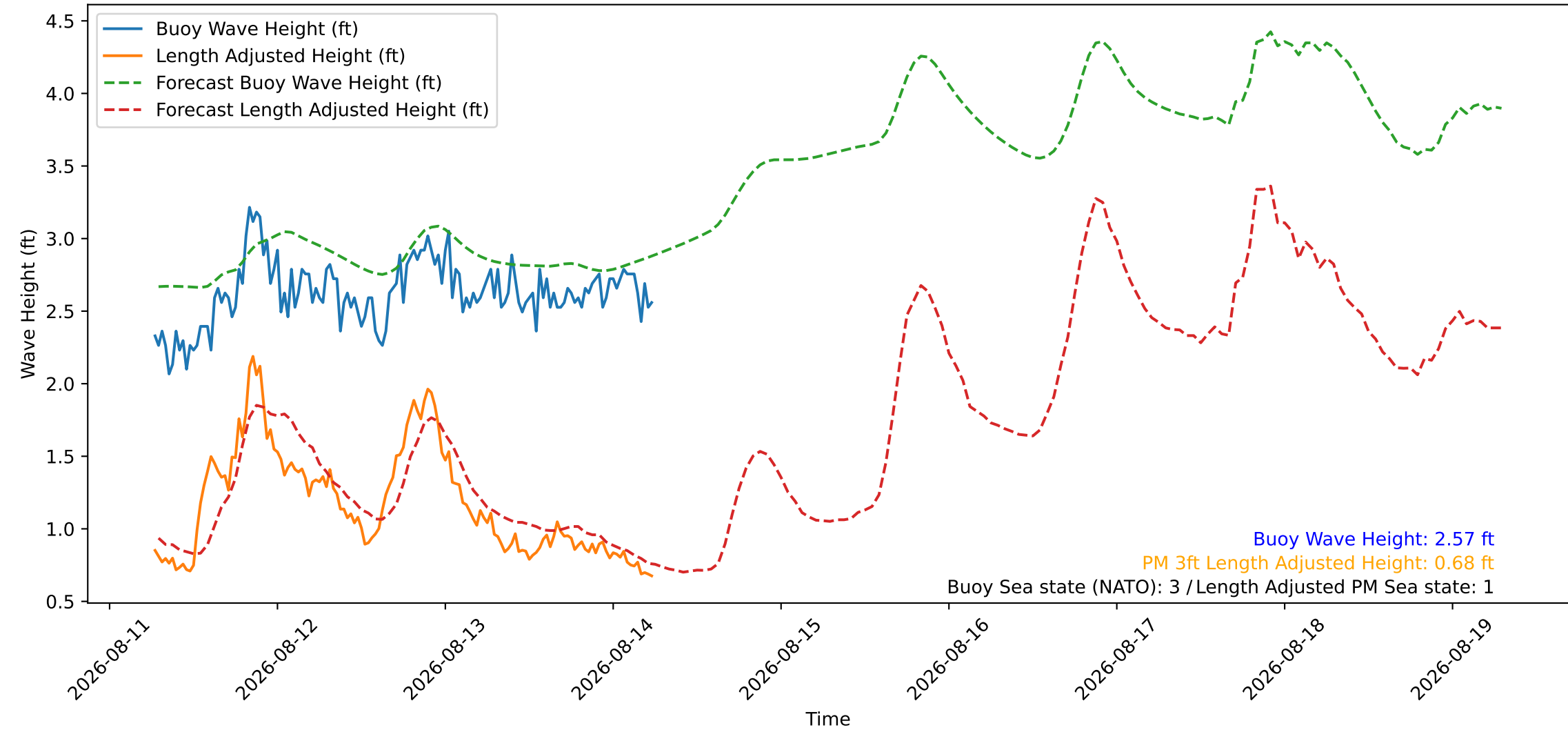
Wave Heights over Time for Green Beach at 2026-08-14 06:31:07
