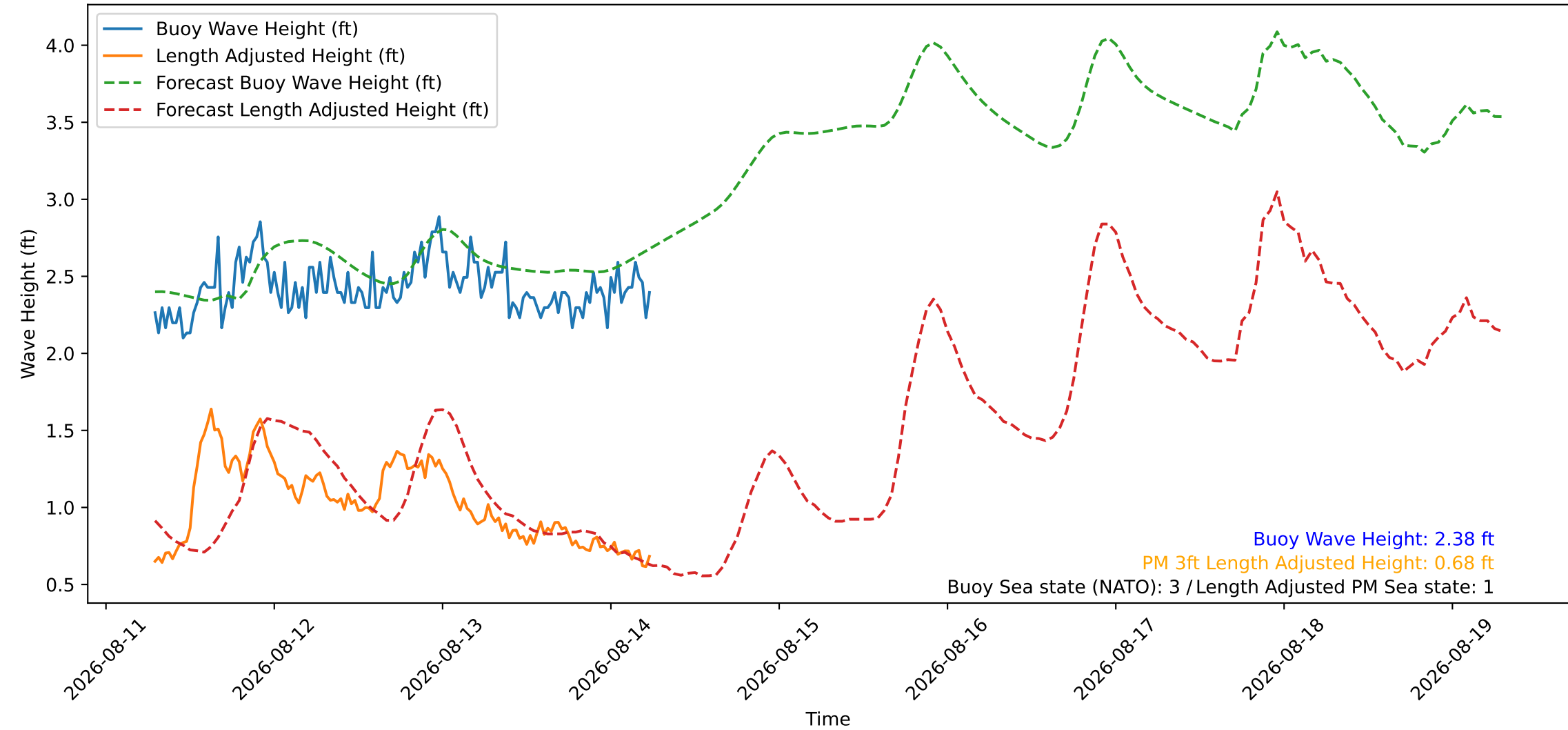
Wave Heights over Time for Red Beach at 2026-08-14 06:30:45
