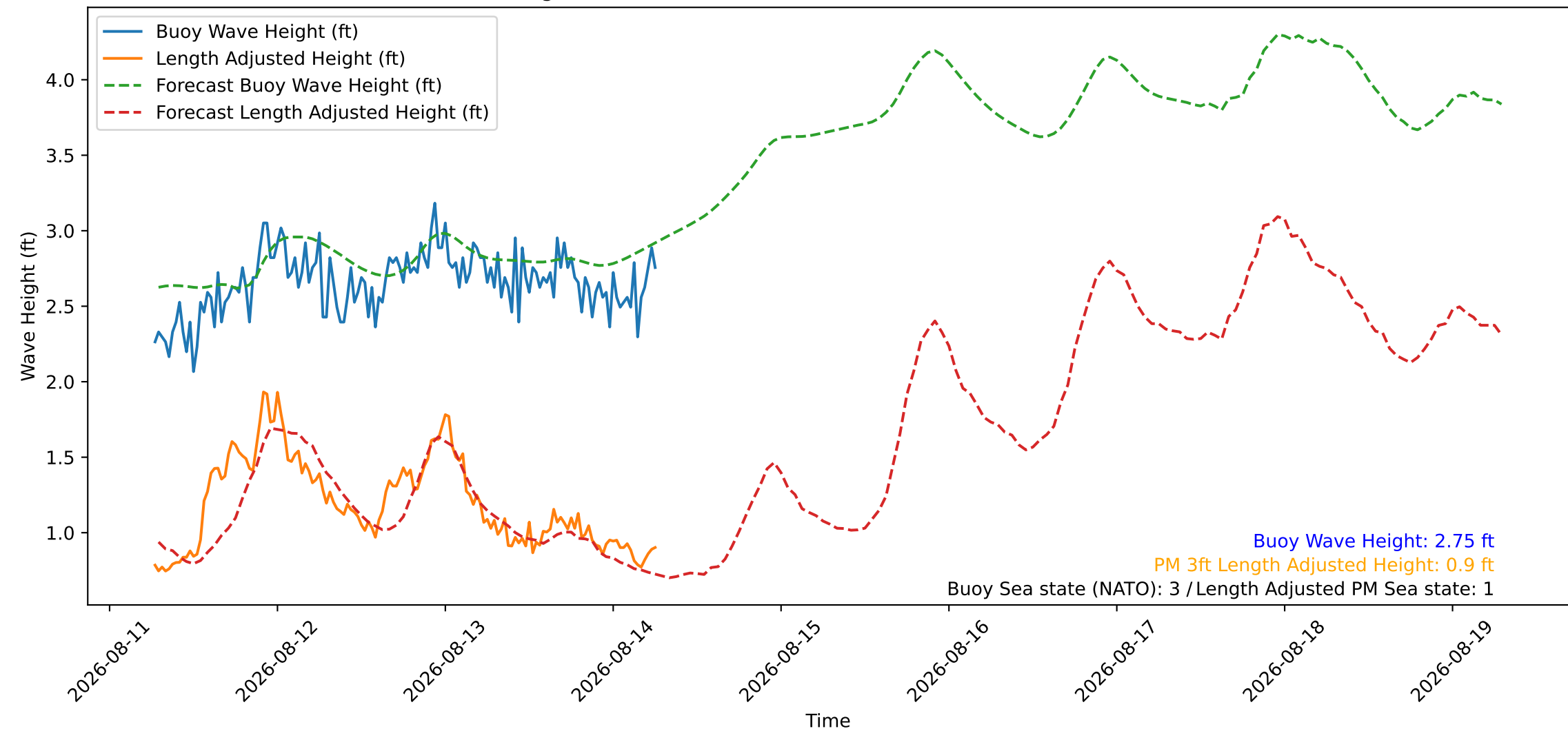
Wave Heights over Time for Oceanside Harbor at 2026-08-14 06:30:26
