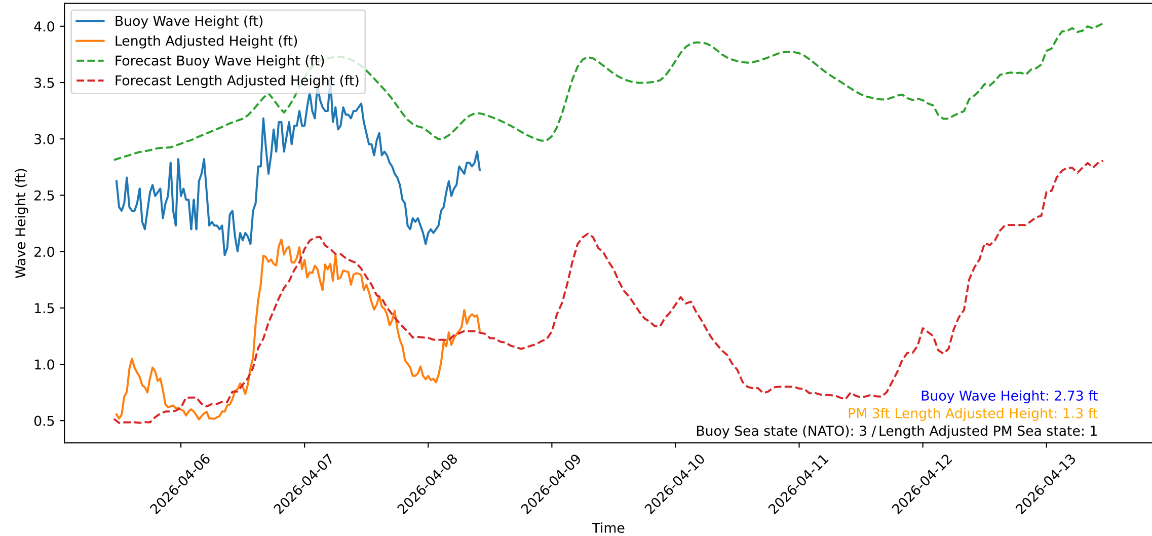
Wave Heights over Time for Red Beach at 2026-04-08 11:00:49
