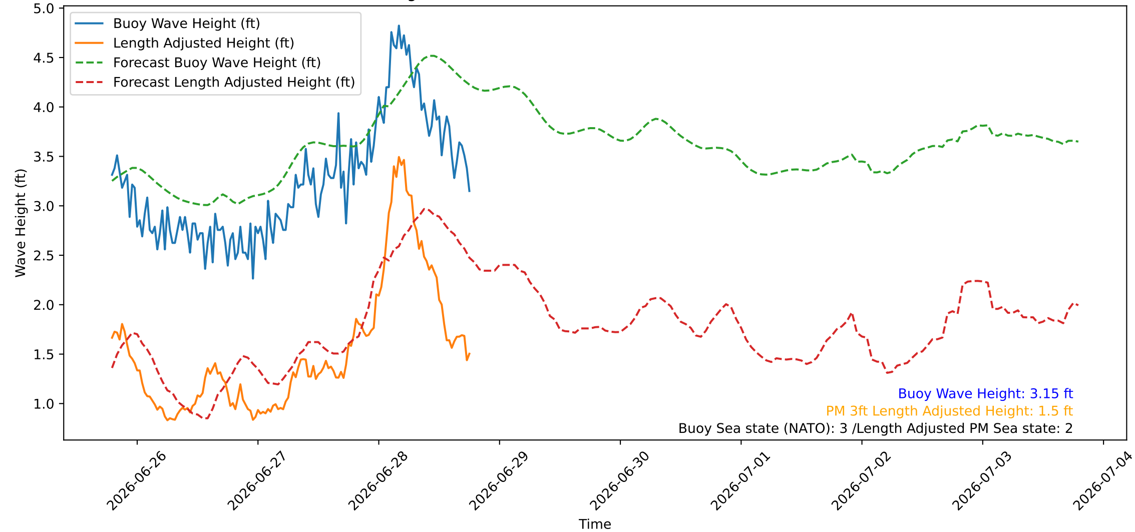
Wave Heights over Time for Green Beach at 2026-06-28 18:51:09
