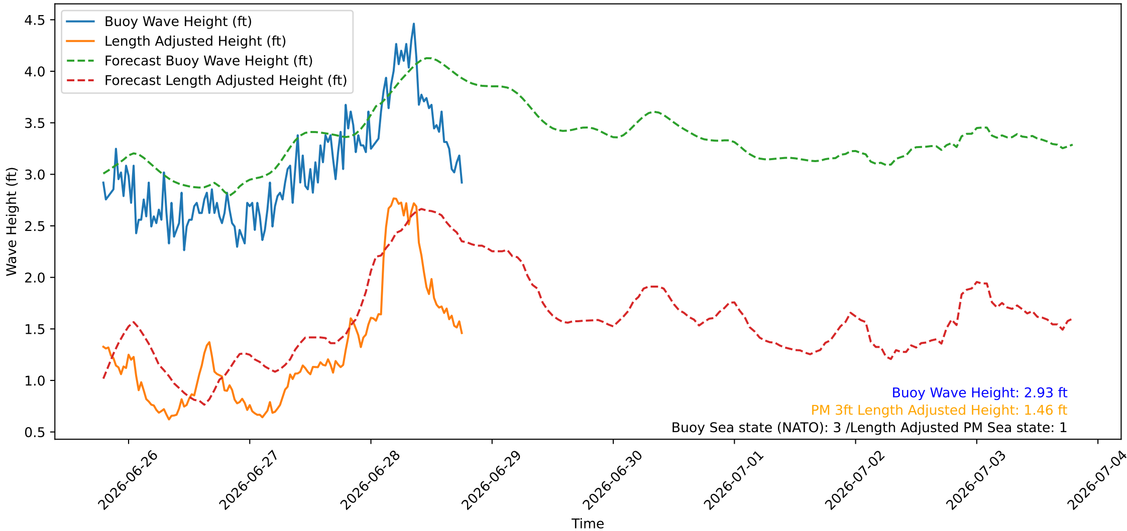
Wave Heights over Time for Red Beach at 2026-06-28 18:50:46
