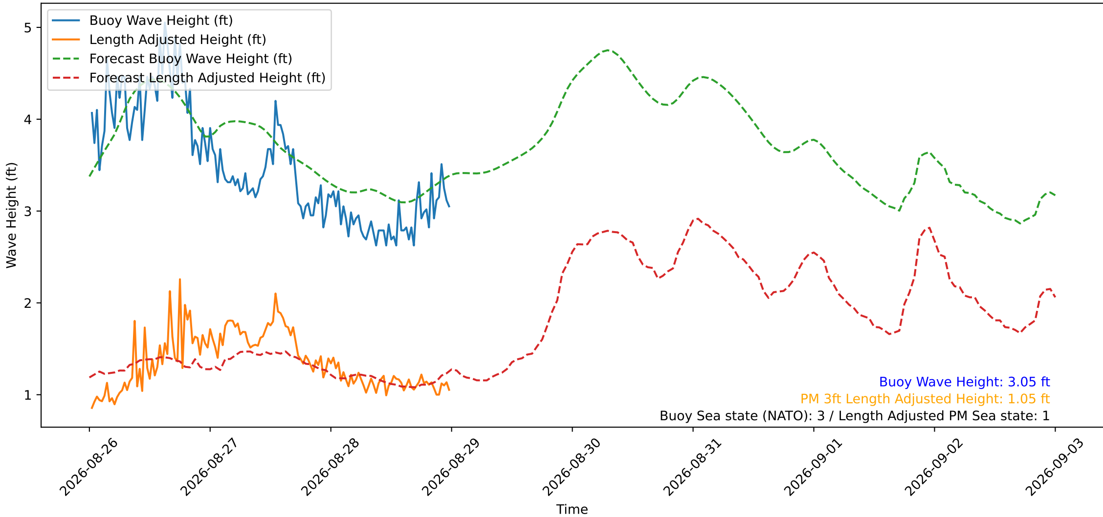
Wave Heights over Time for Red Beach at 2026-08-29 00:10:49
