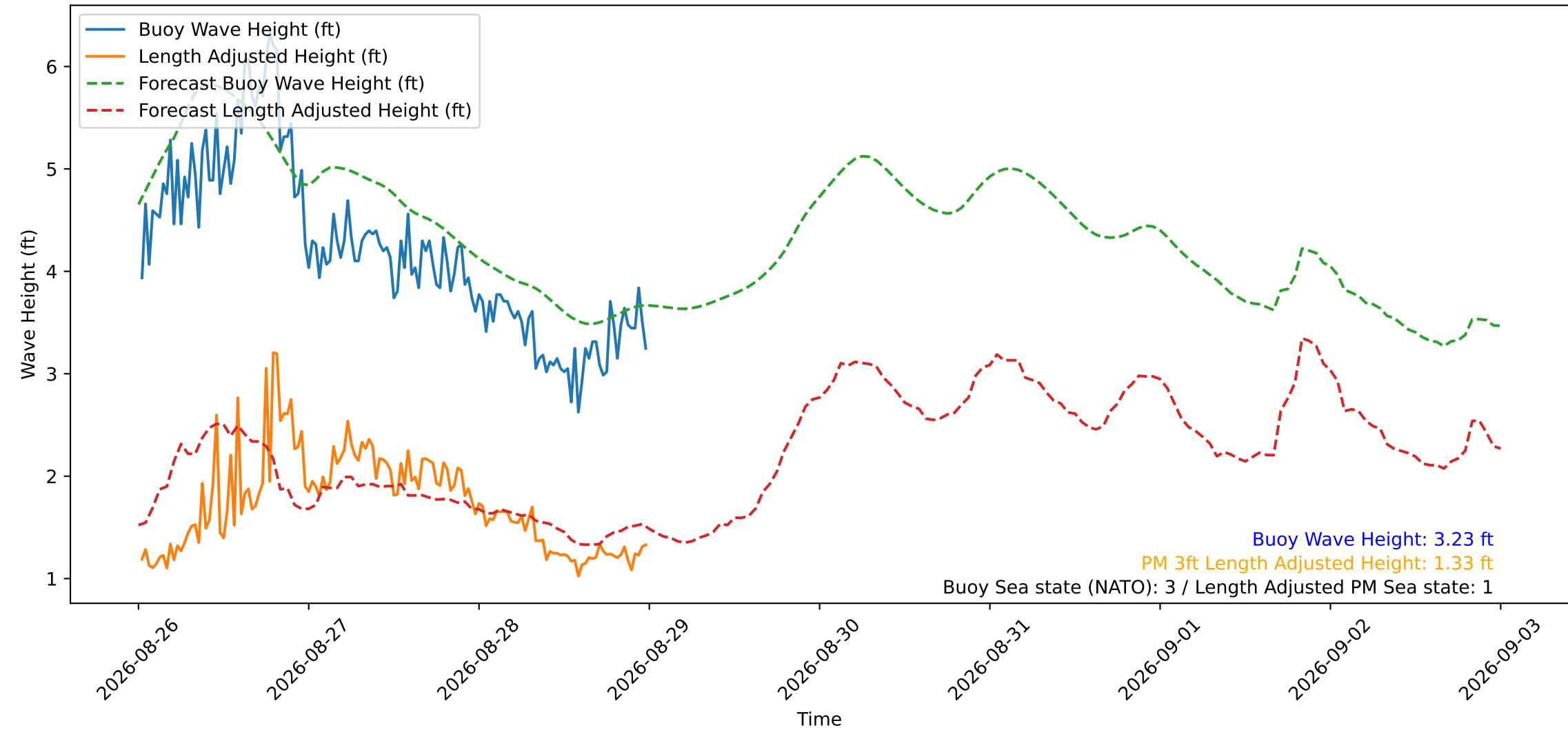
Wave Heights over Time for Green Beach at 2026-08-29 00:11:12
