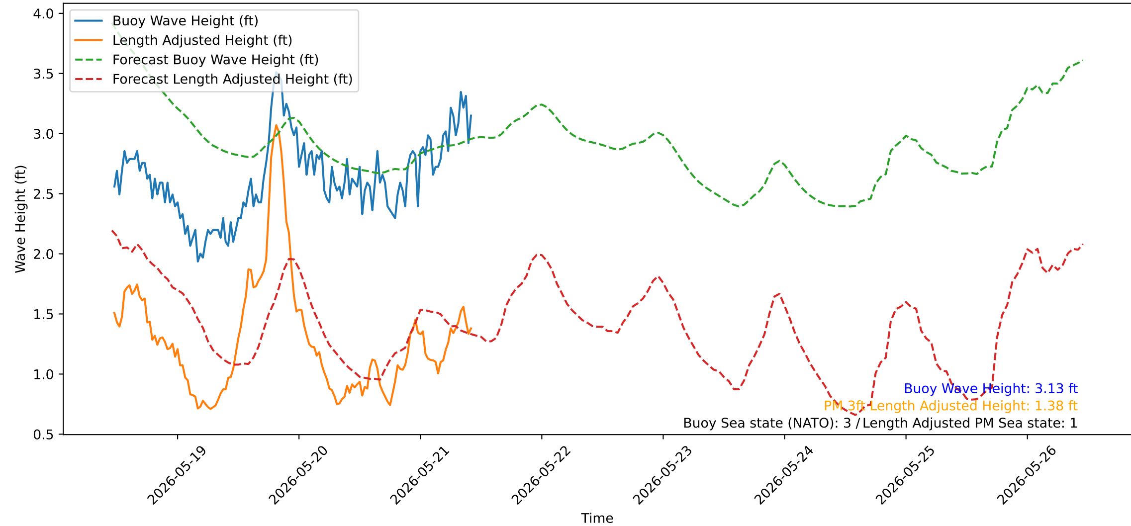
Wave Heights over Time for Red Beach at 2026-05-21 11:00:51
