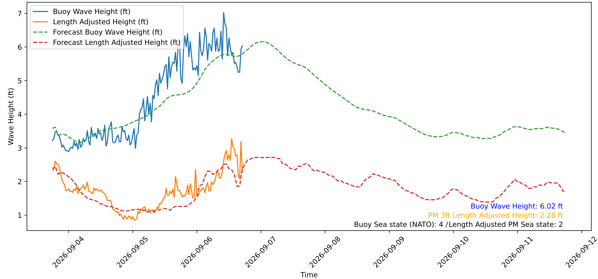
Wave Heights over Time for Oceanside Harbor at 2026-09-06 18:00:29
