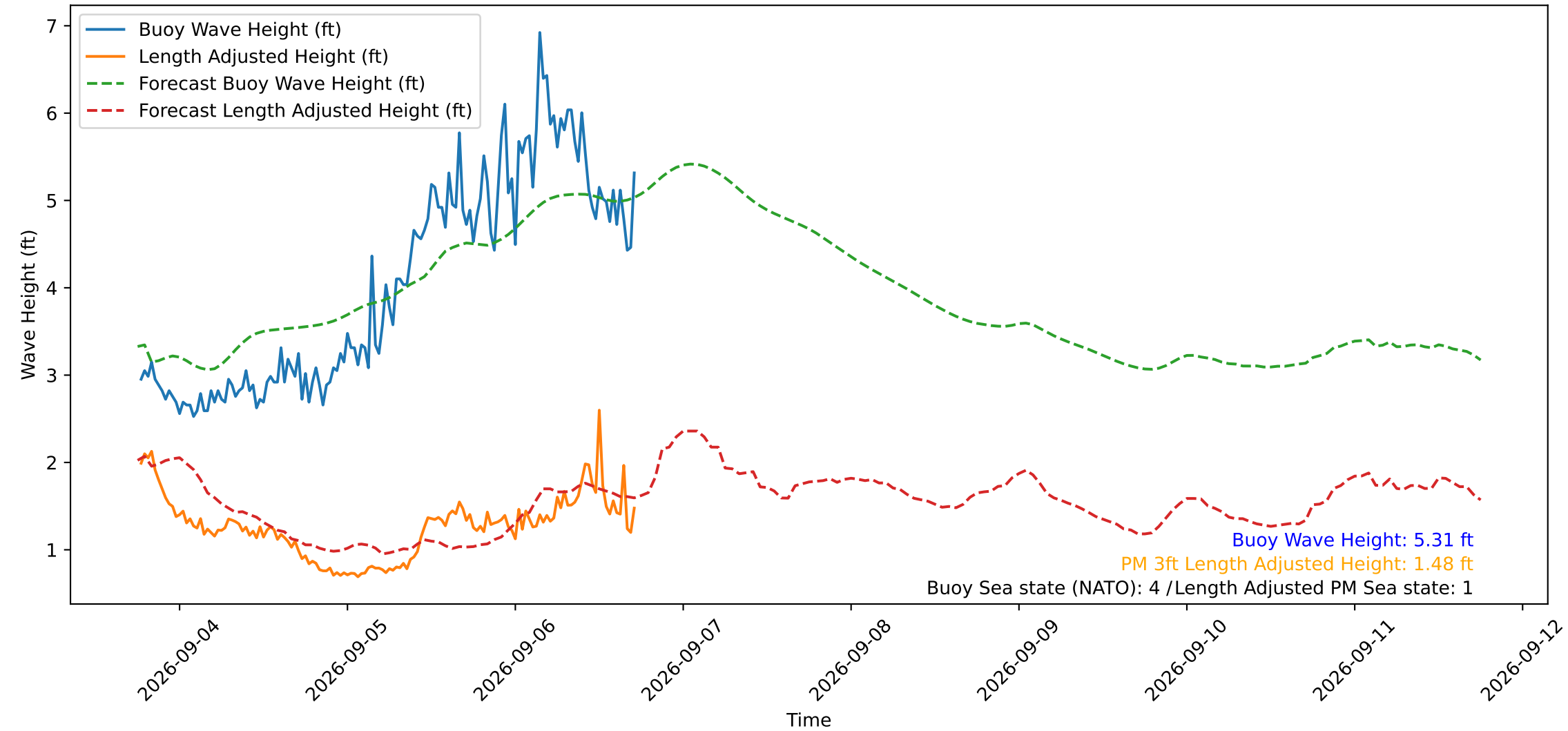
Wave Heights over Time for Red Beach at 2026-09-06 18:00:49
