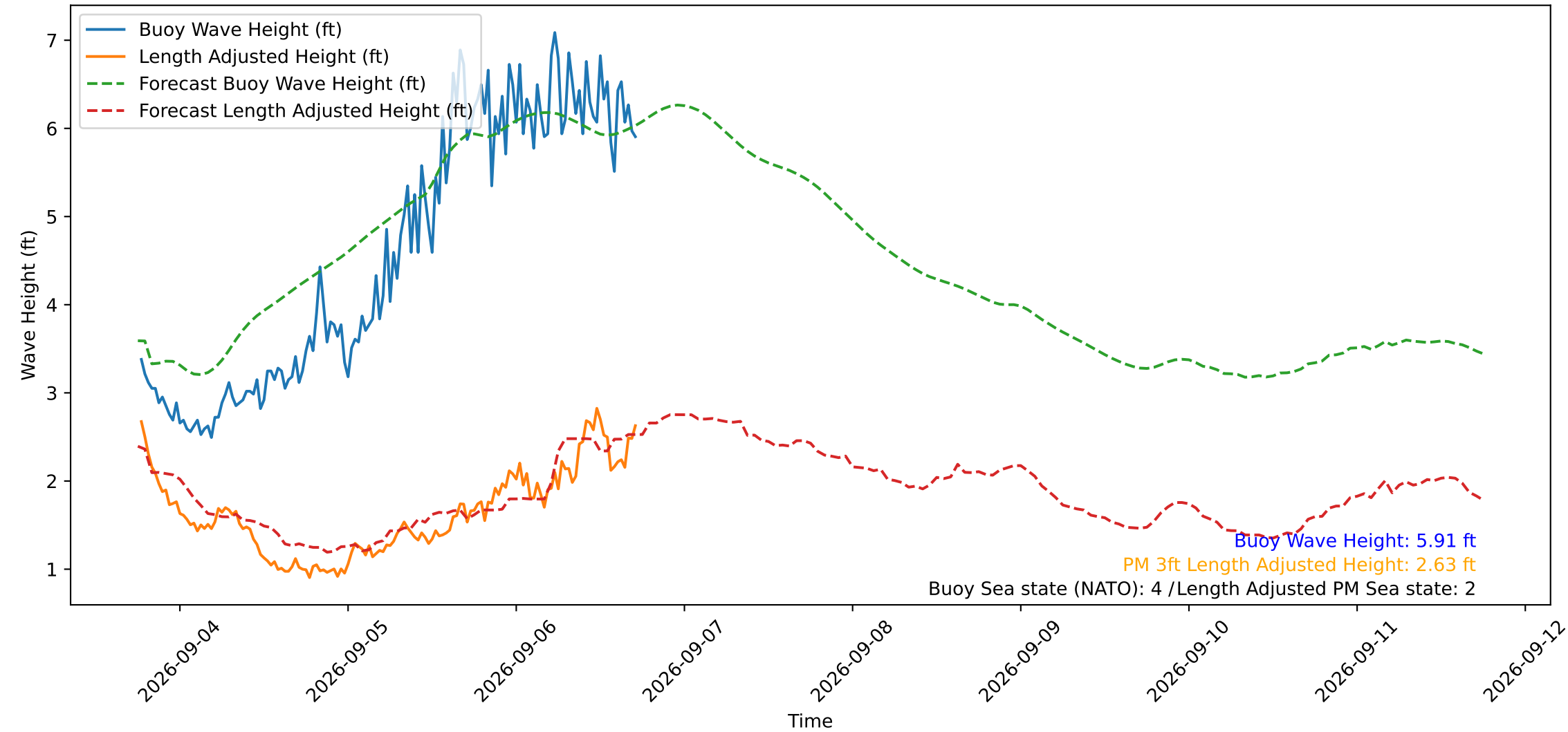
Wave Heights over Time for Green Beach at 2026-09-06 18:01:12
