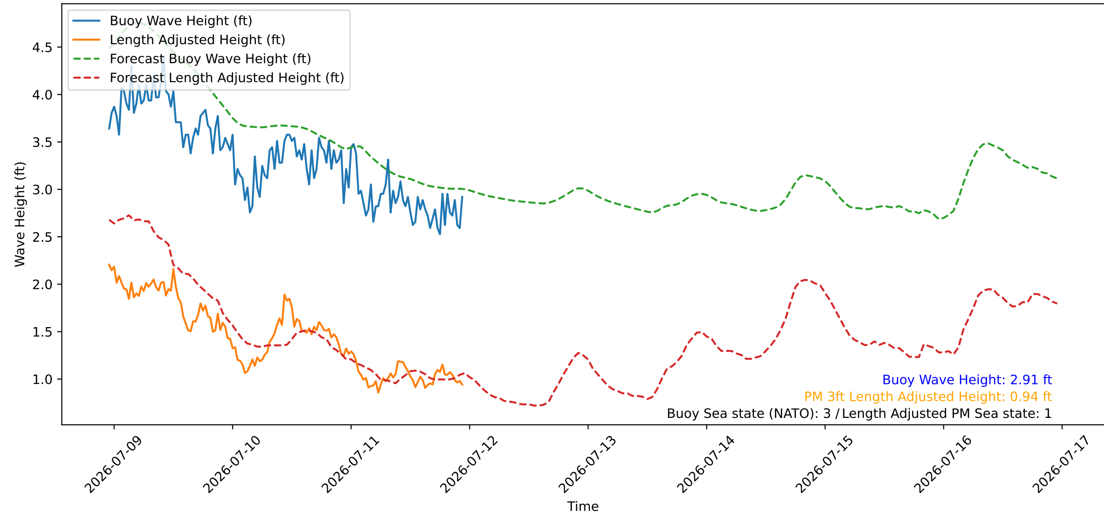
Wave Heights over Time for Green Beach at 2026-07-11 23:11:08
