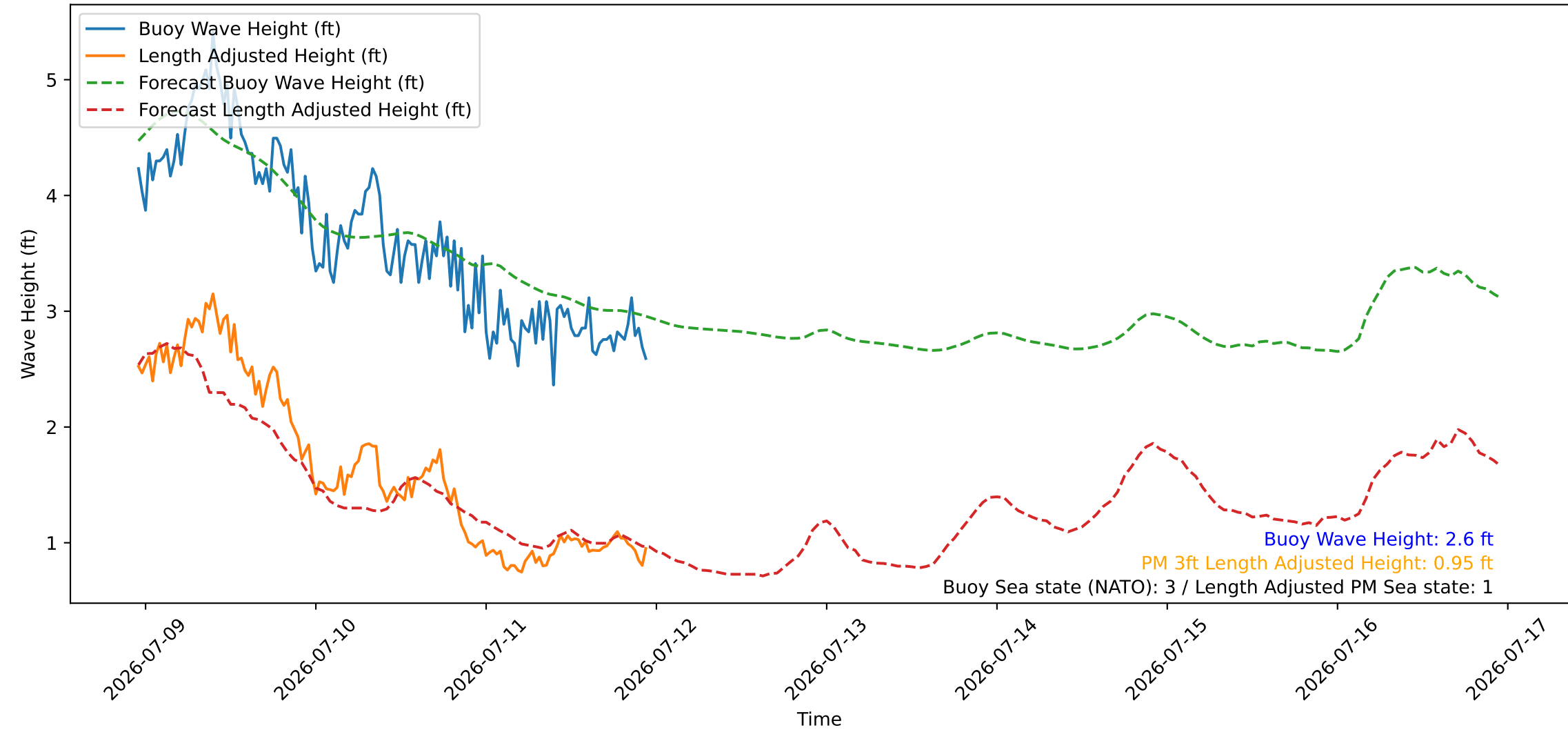
Wave Heights over Time for Oceanside Harbor at 2026-07-11 23:10:26
