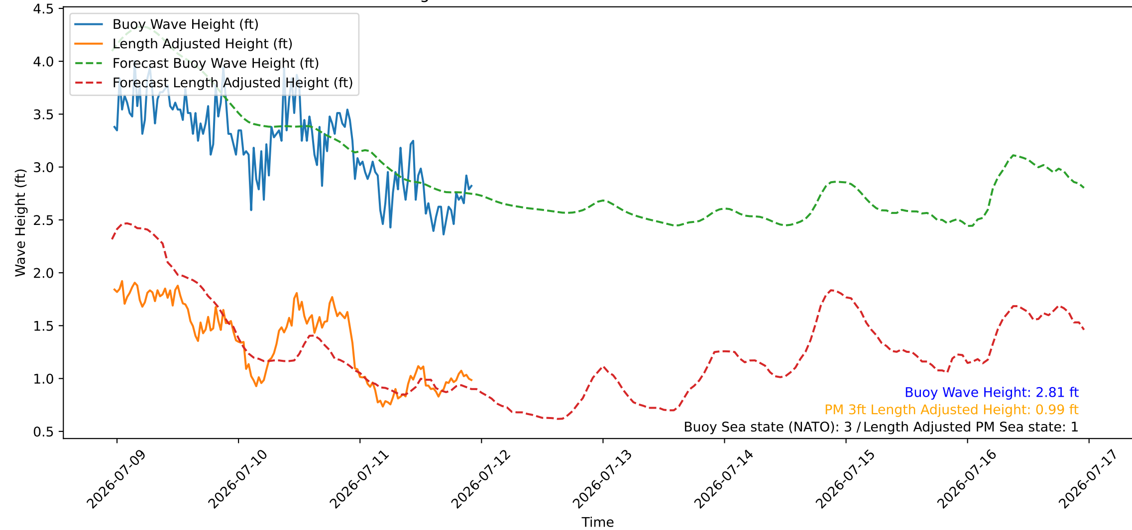
Wave Heights over Time for Red Beach at 2026-07-11 23:10:45
