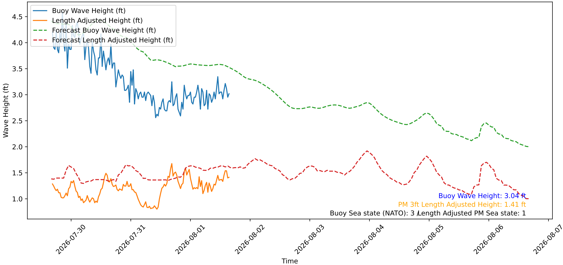
Wave Heights over Time for Red Beach at 2026-08-01 16:10:46
