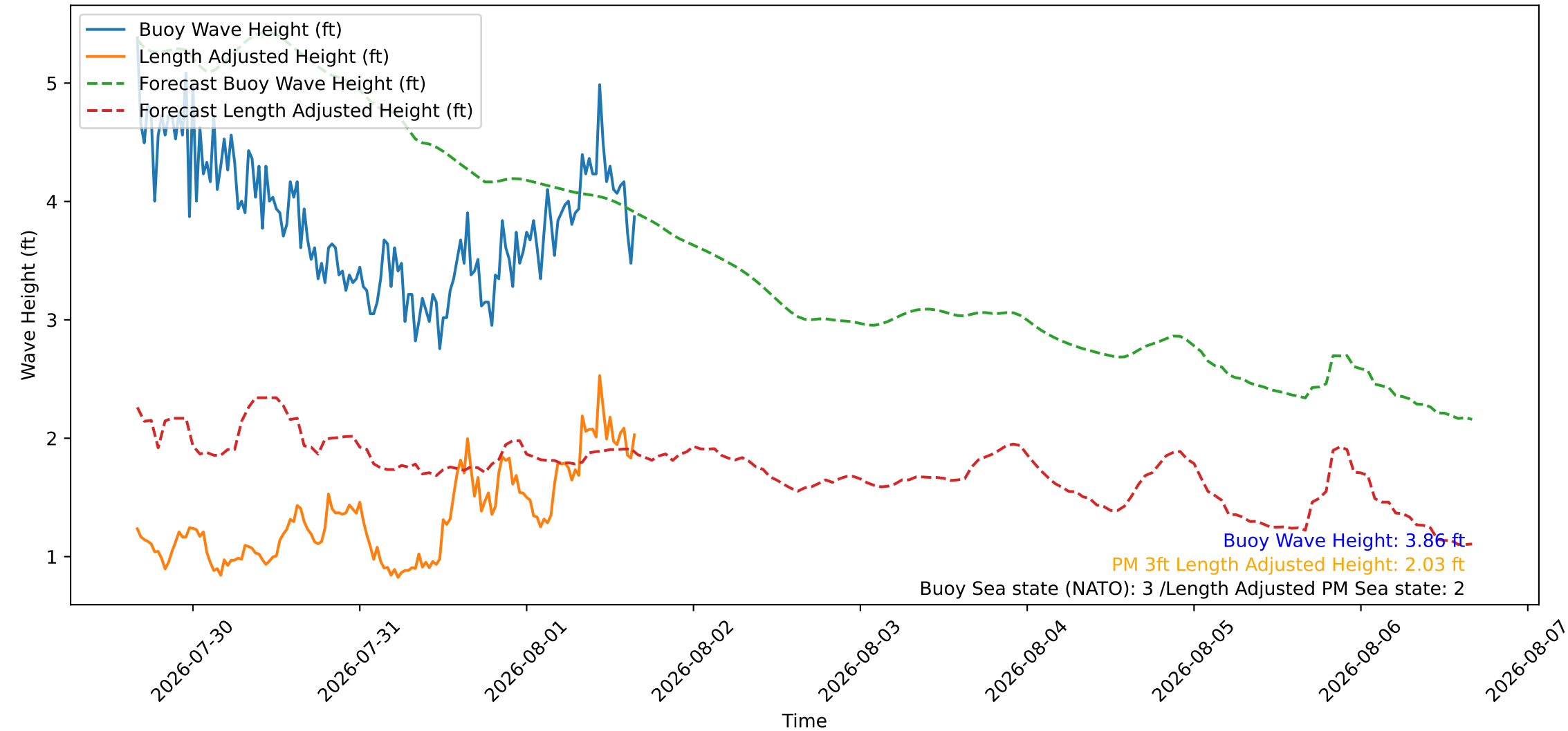
Wave Heights over Time for Green Beach at 2026-08-01 16:11:09
