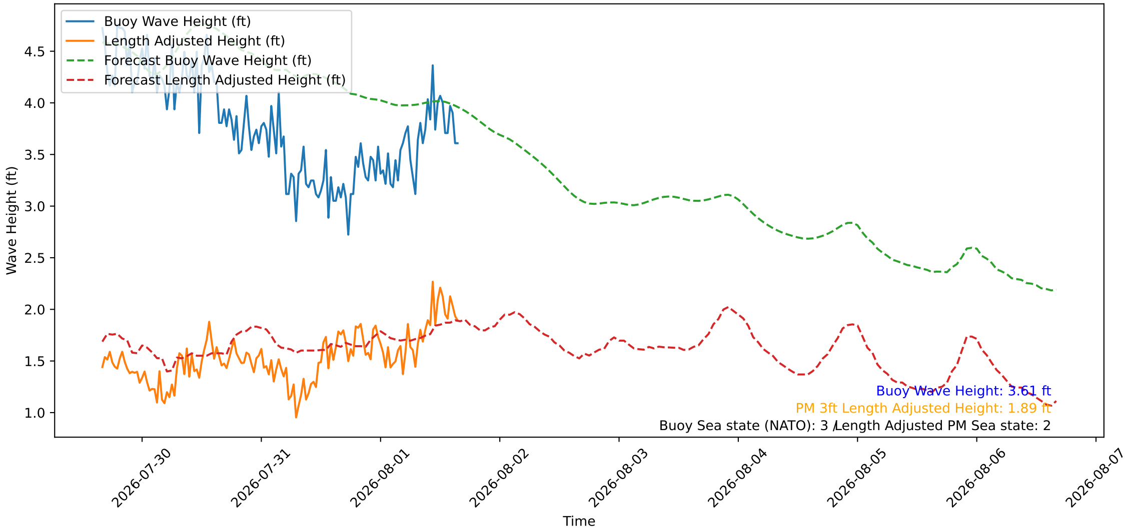
Wave Heights over Time for Oceanside Harbor at 2026-08-01 16:10:26
