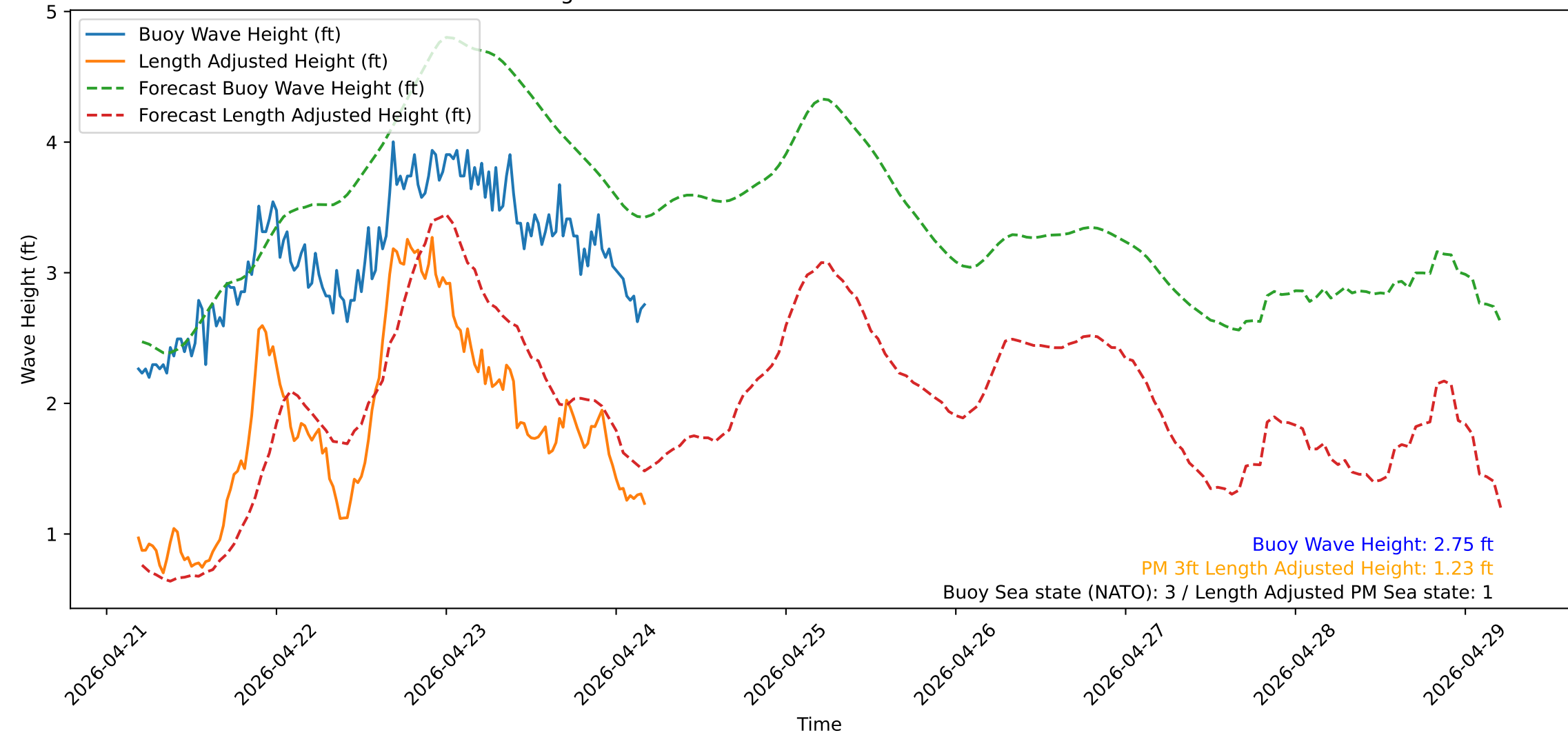
Wave Heights over Time for Green Beach at 2026-04-24 04:41:13
