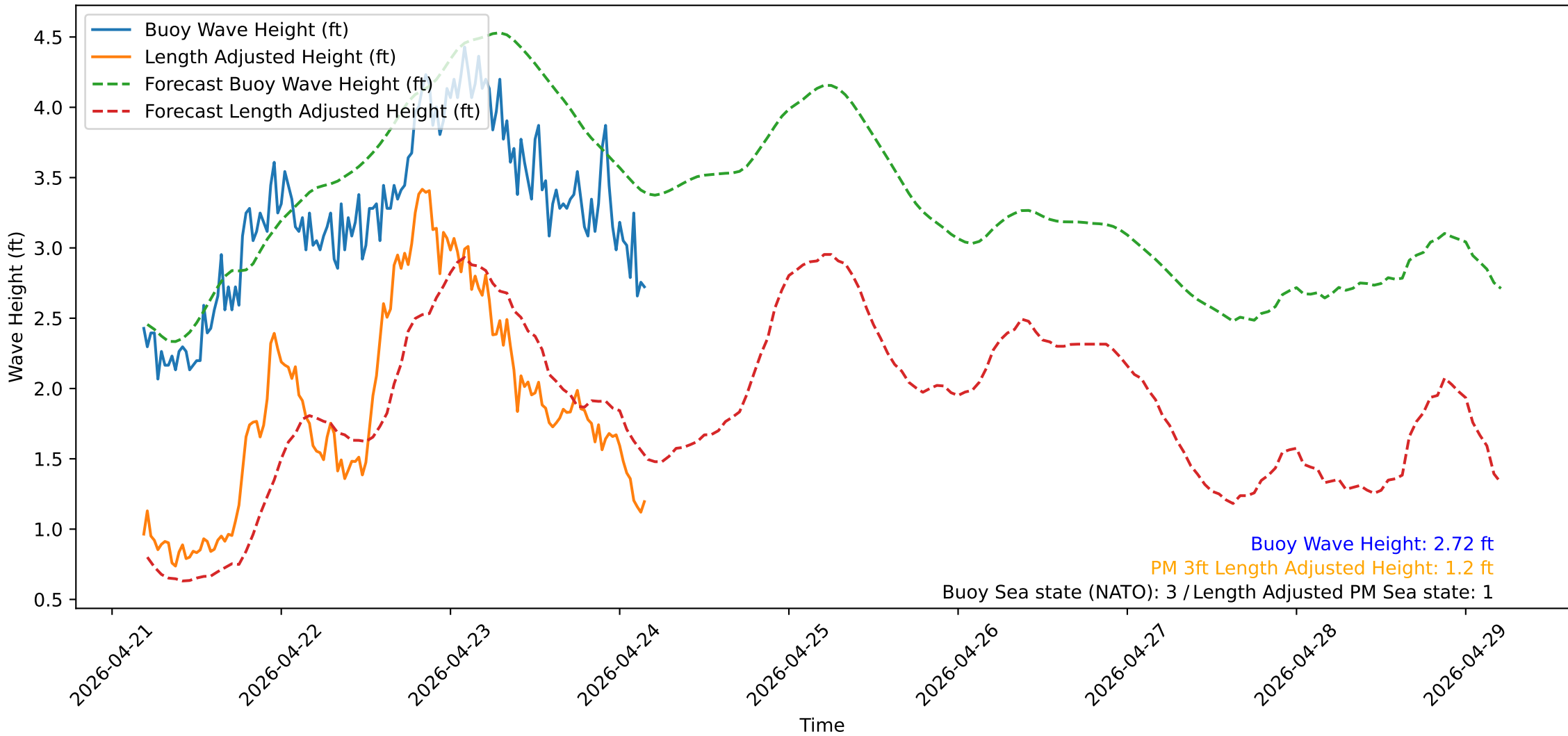
Wave Heights over Time for Oceanside Harbor at 2026-04-24 04:40:31
