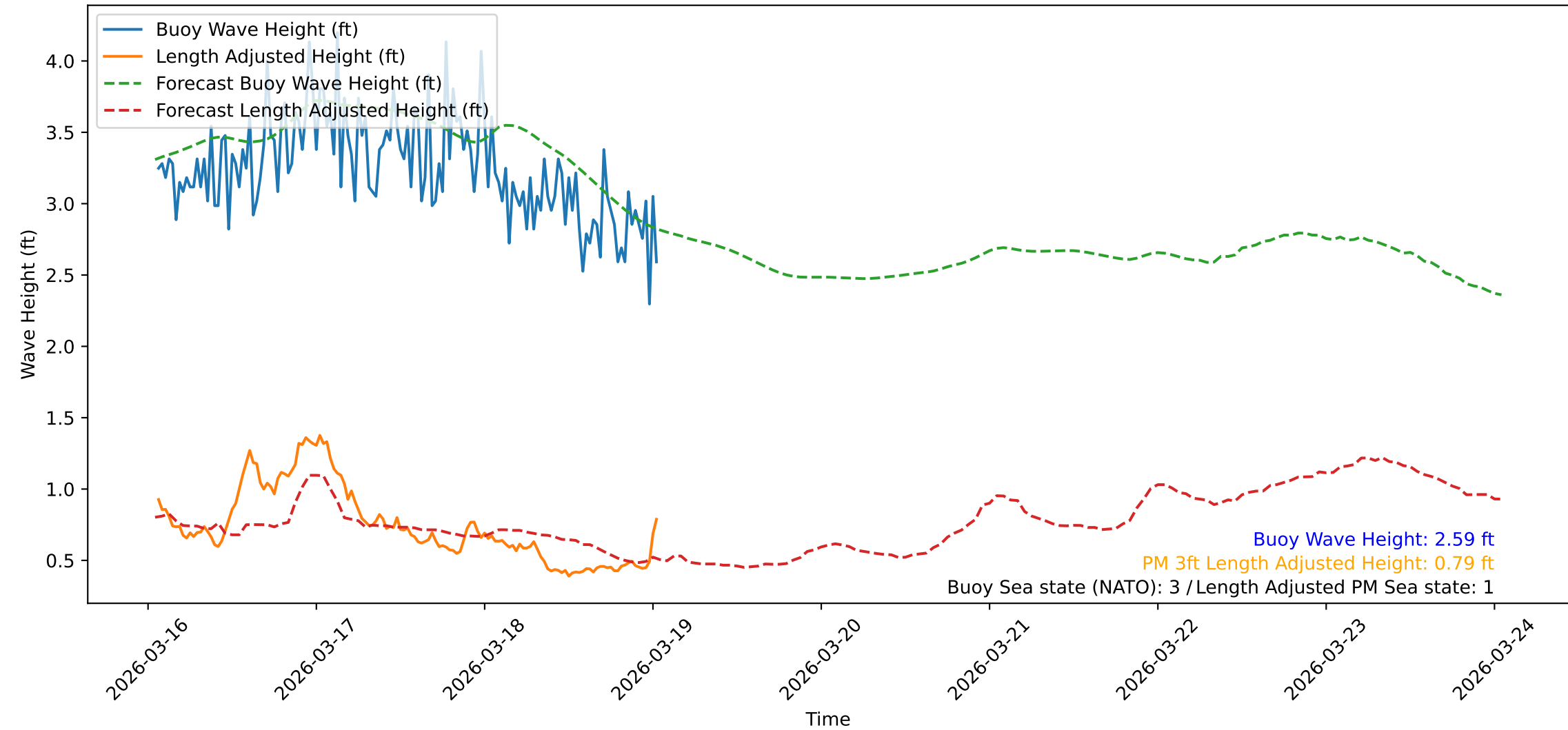
Wave Heights over Time for Green Beach at 2026-03-19 01:21:10
