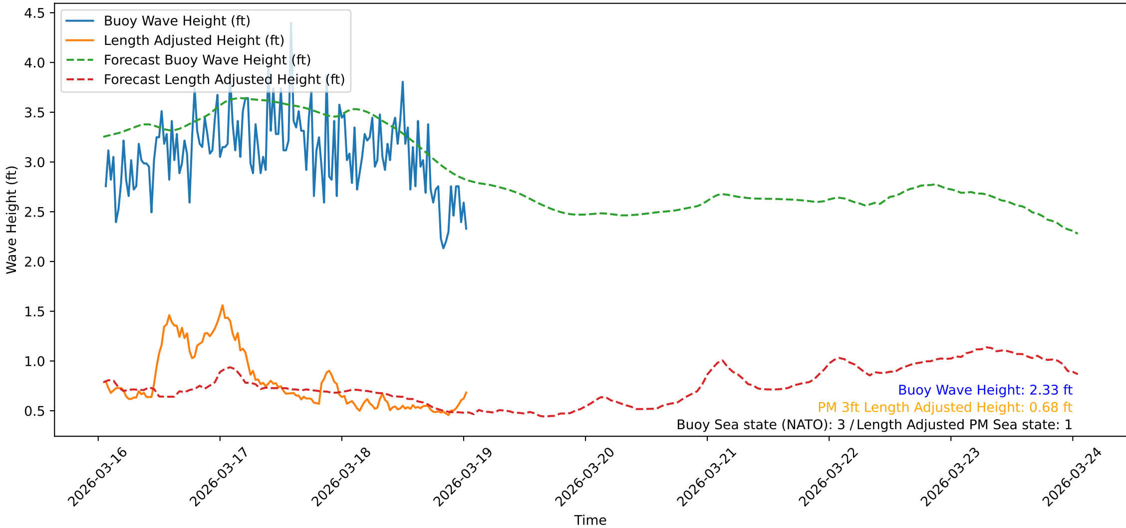
Wave Heights over Time for Oceanside Harbor at 2026-03-19 01:20:31
