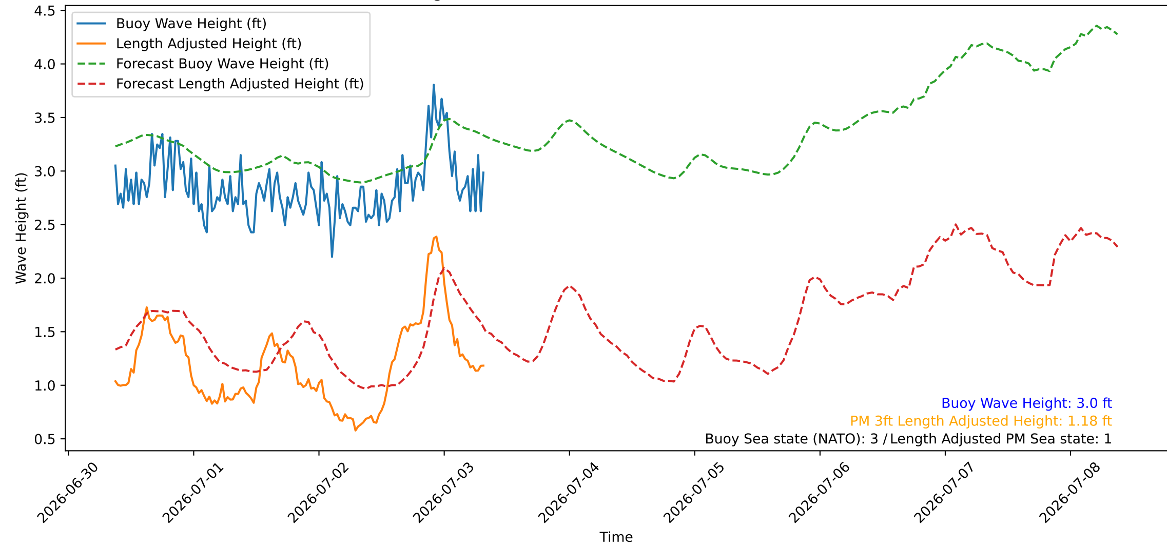
Wave Heights over Time for Red Beach at 2026-07-03 08:30:46
