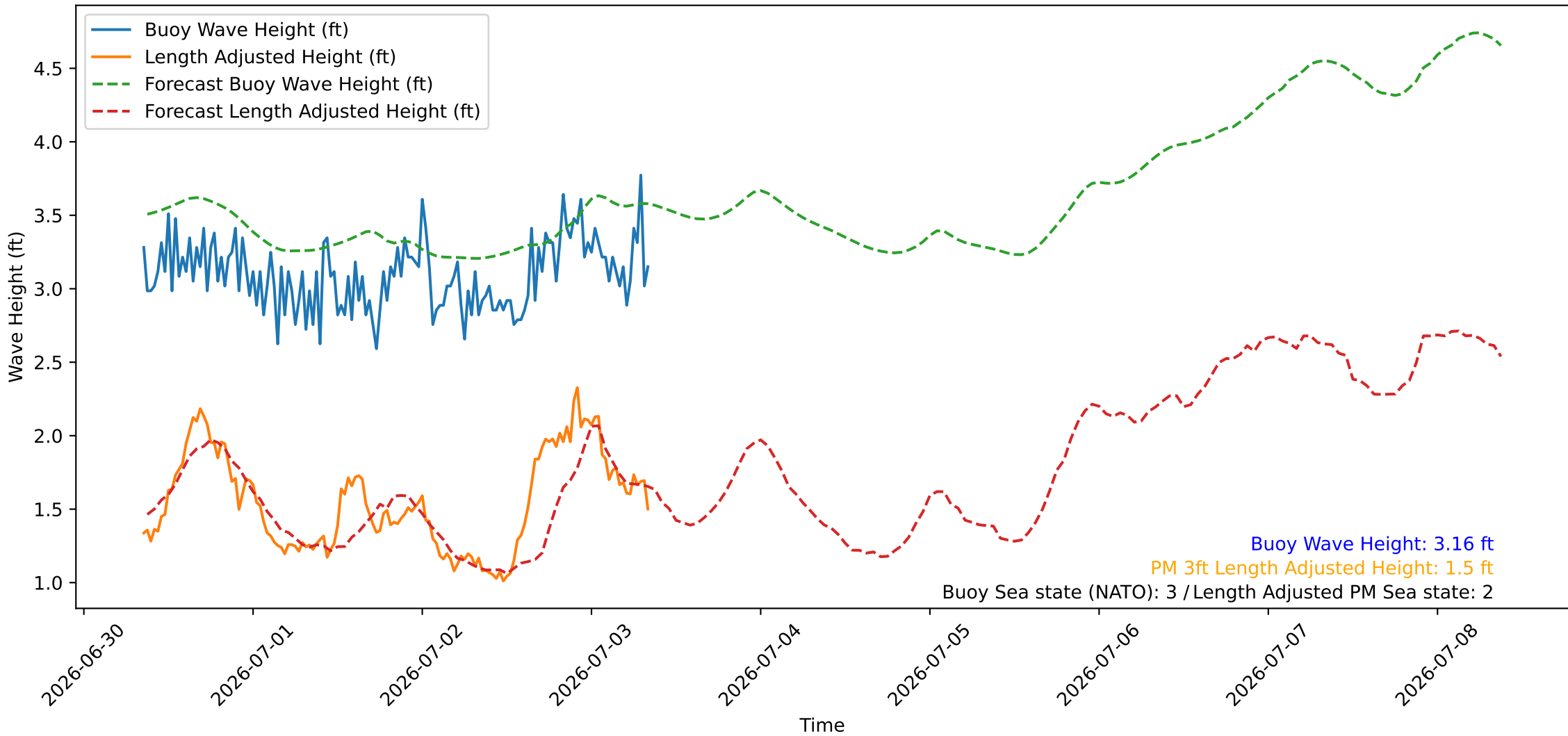
Wave Heights over Time for Oceanside Harbor at 2026-07-03 08:30:27
