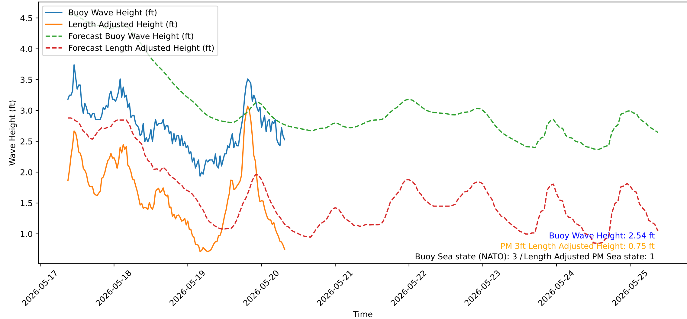
Wave Heights over Time for Red Beach at 2026-05-20 08:30:51
