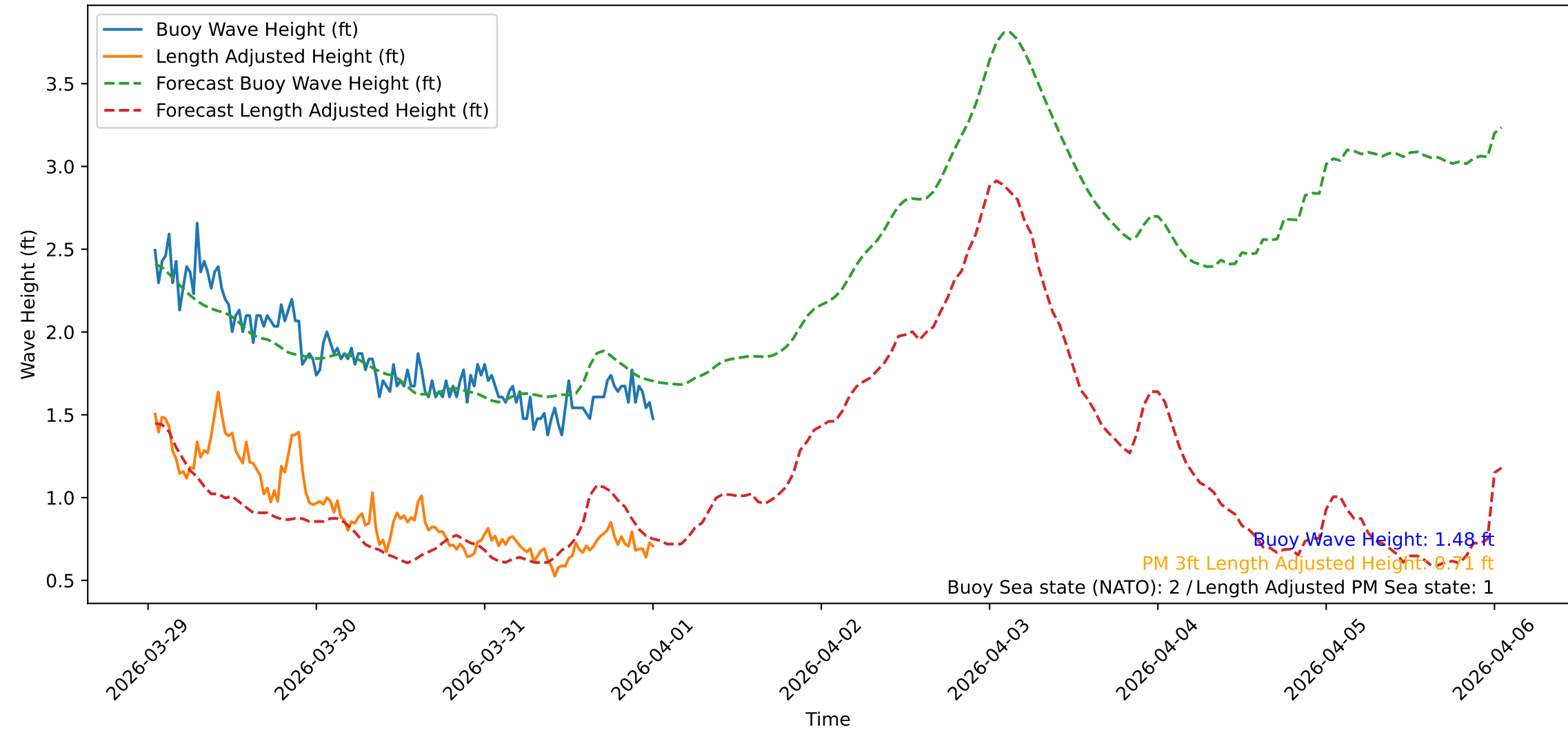
Wave Heights over Time for Red Beach at 2026-04-01 00:50:46
