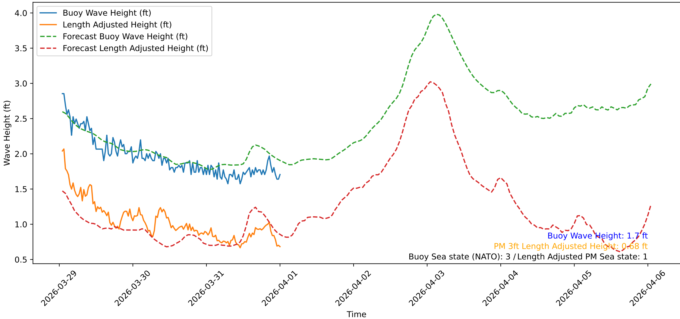
Wave Heights over Time for Oceanside Harbor at 2026-04-01 00:50:31
