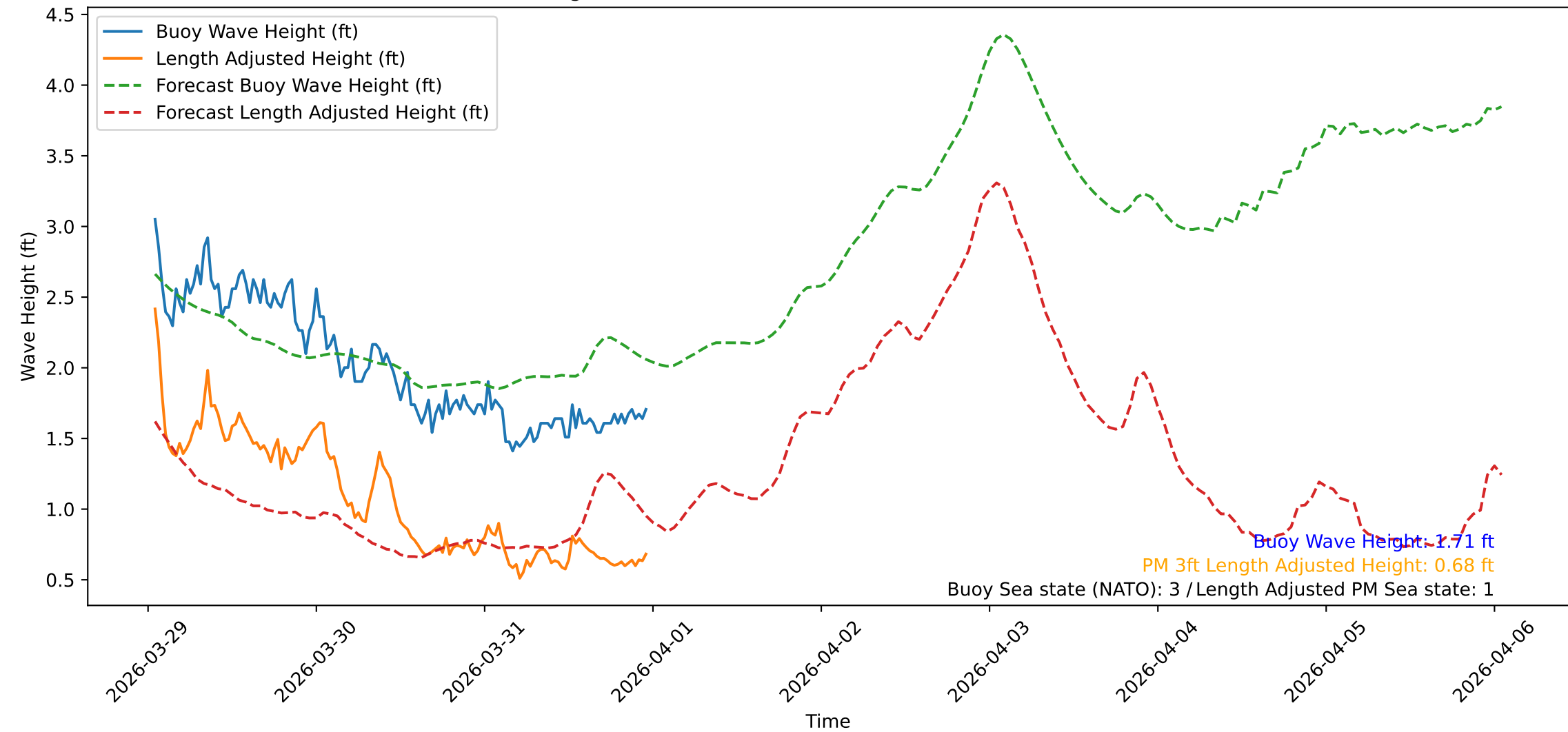
Wave Heights over Time for Green Beach at 2026-04-01 00:51:08
