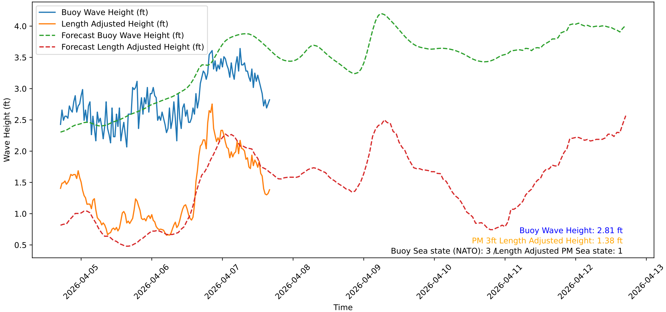
Wave Heights over Time for Oceanside Harbor at 2026-04-07 16:50:31
