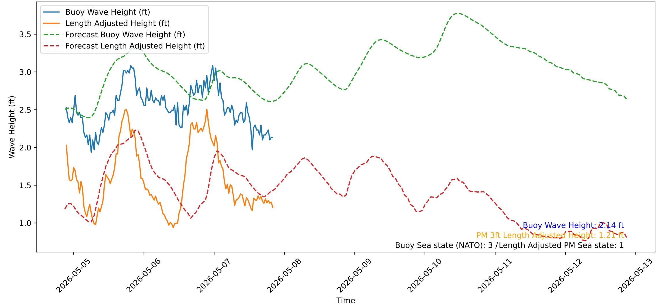
Wave Heights over Time for Red Beach at 2026-05-07 21:00:51
