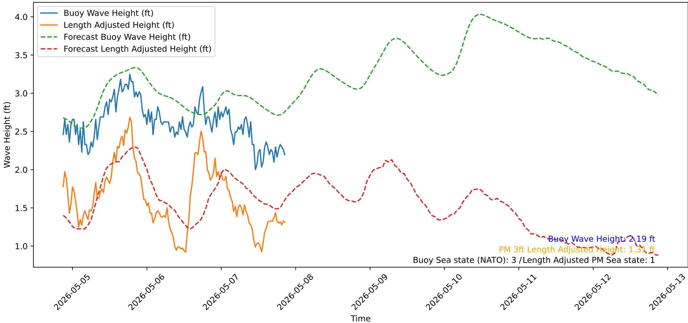
Wave Heights over Time for Oceanside Harbor at 2026-05-07 21:00:31
