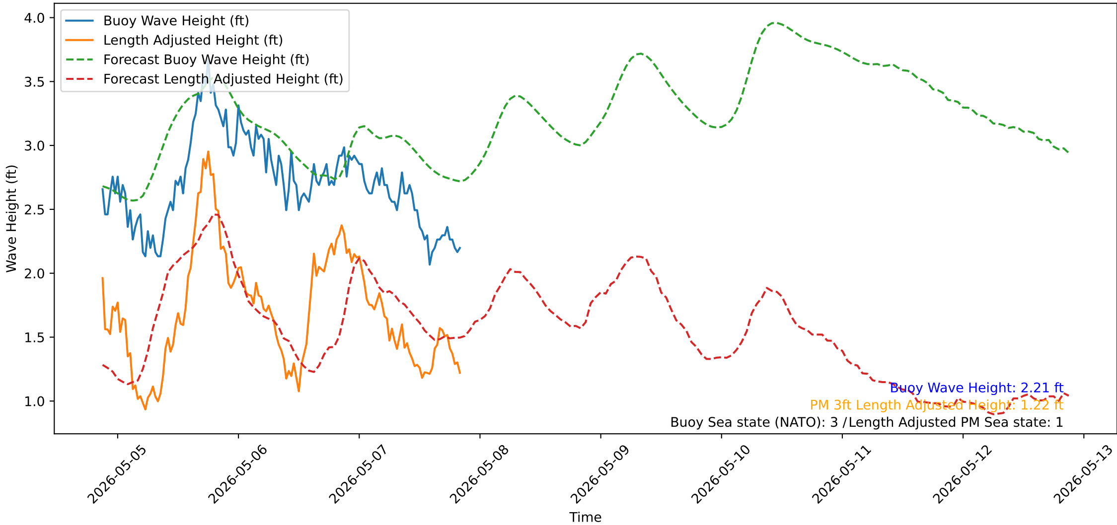
Wave Heights over Time for Green Beach at 2026-05-07 21:01:13
