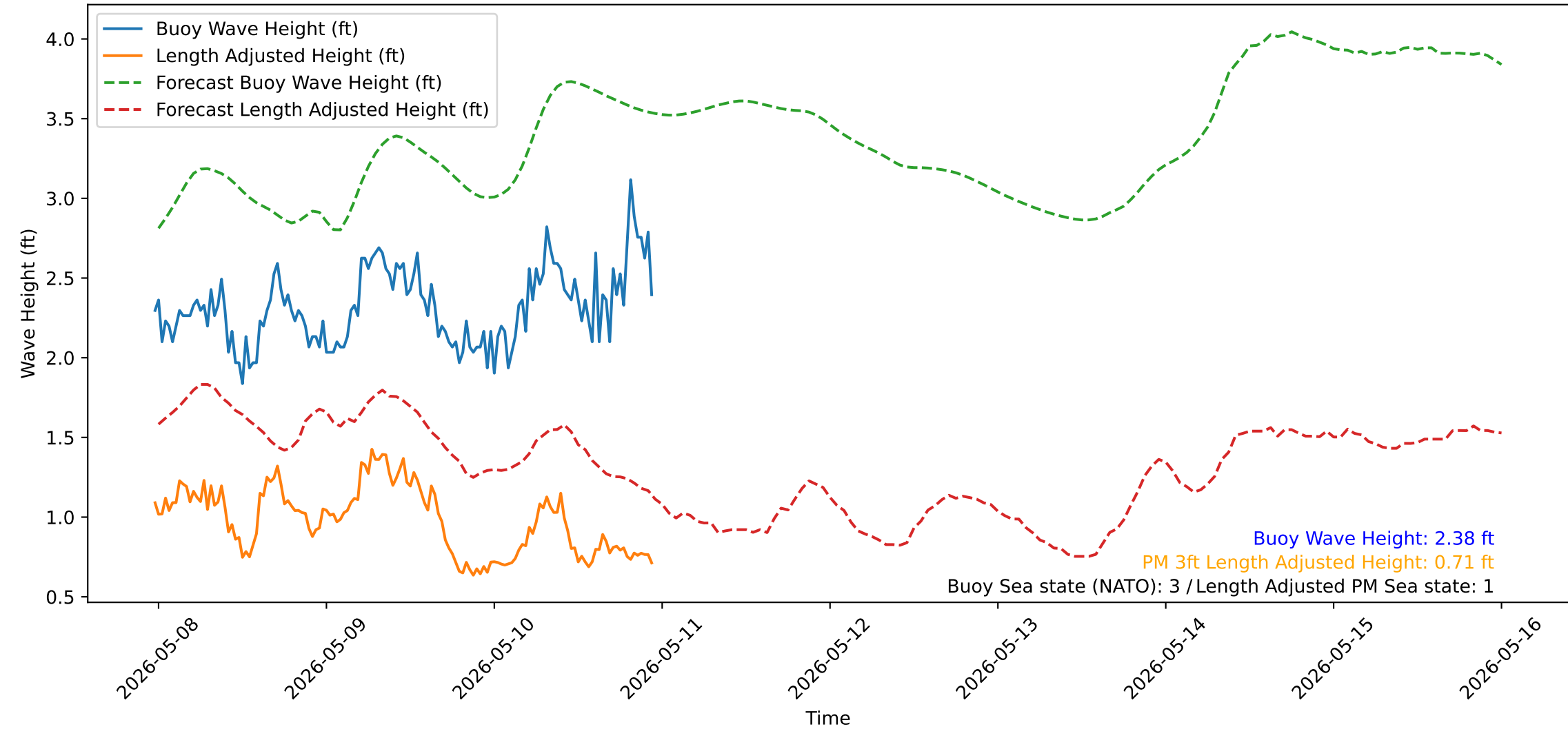
Wave Heights over Time for Green Beach at 2026-05-10 23:31:13
