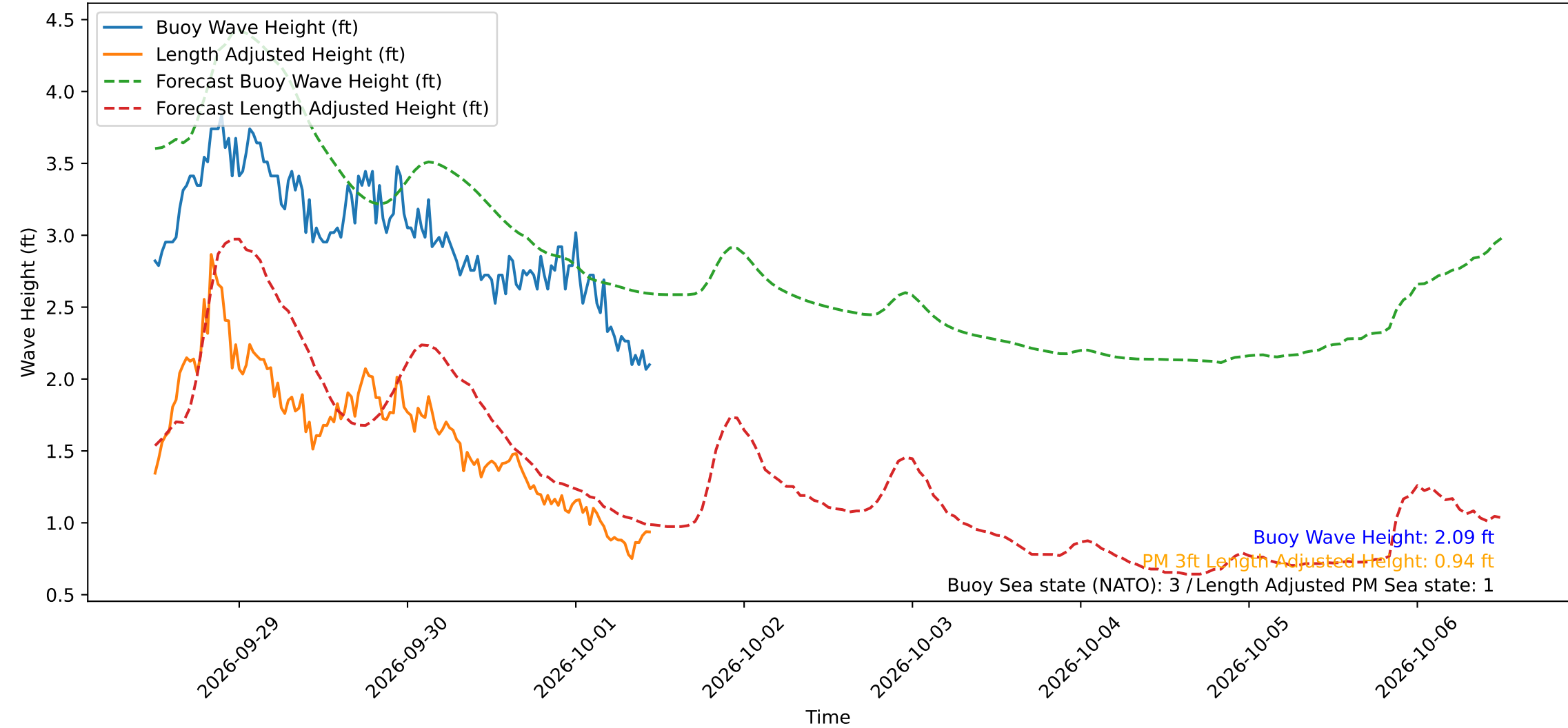
Wave Heights over Time for Red Beach at 2026-10-01 11:30:51
