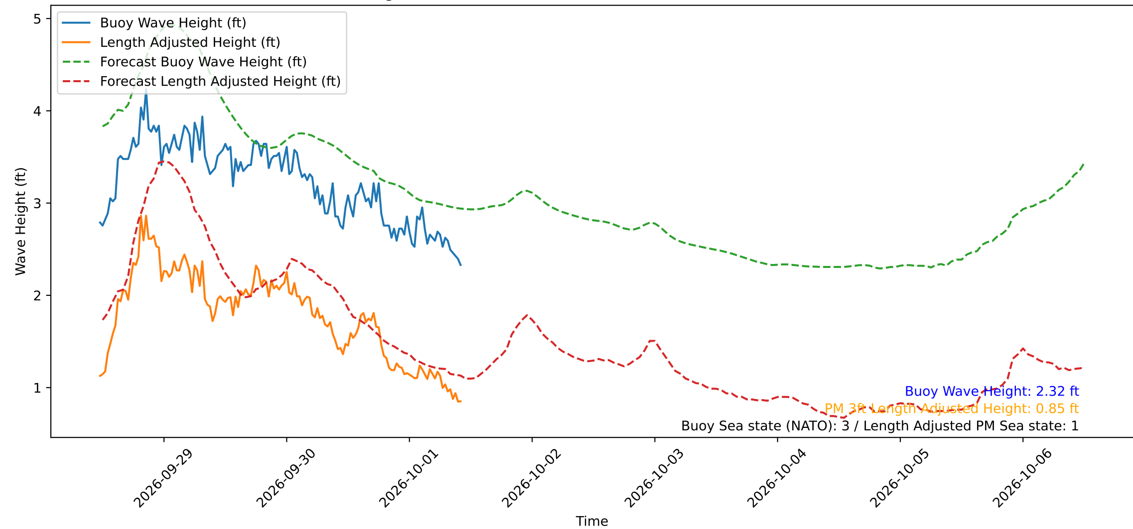
Wave Heights over Time for Oceanside Harbor at 2026-10-01 11:30:31
