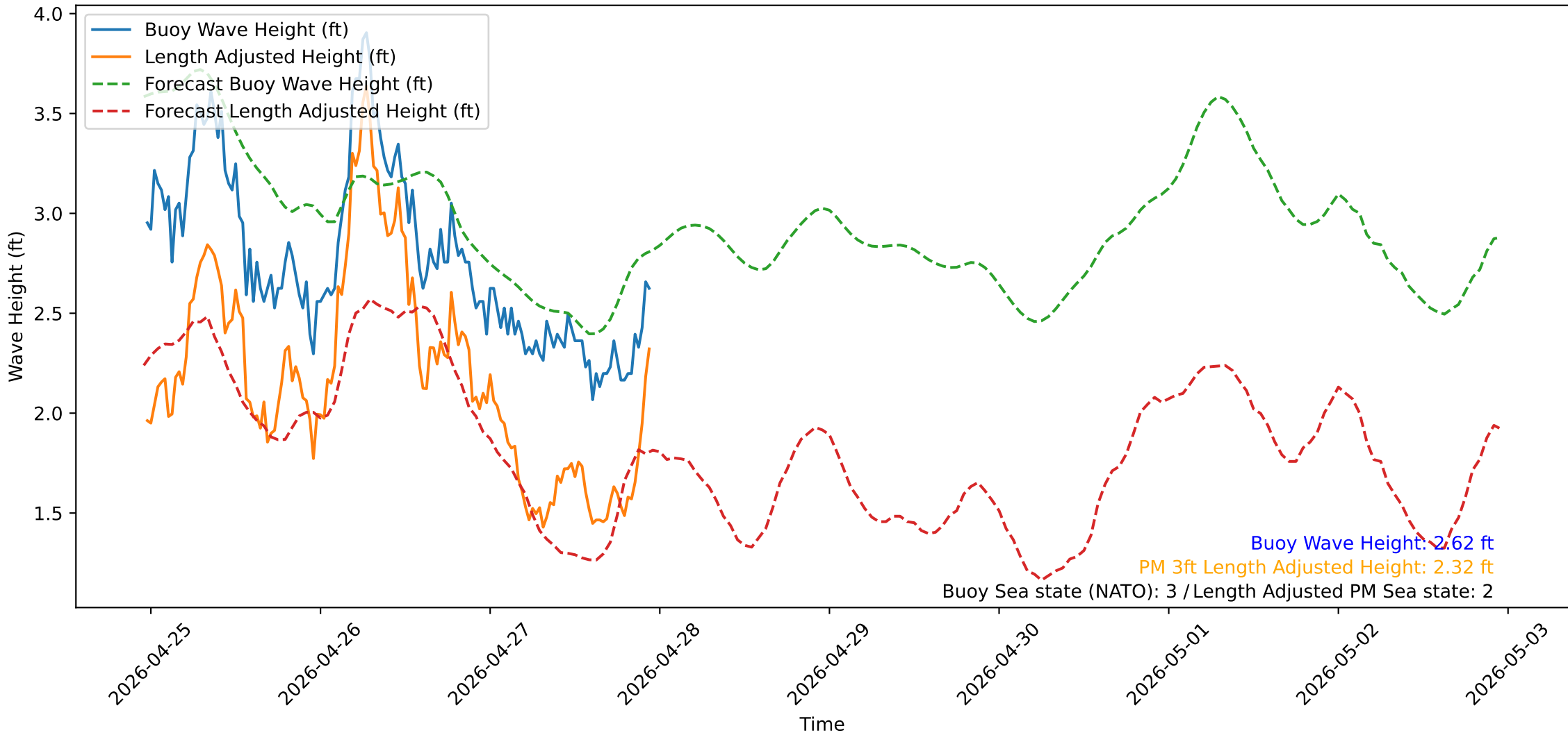
Wave Heights over Time for Oceanside Harbor at 2026-04-27 23:20:31
