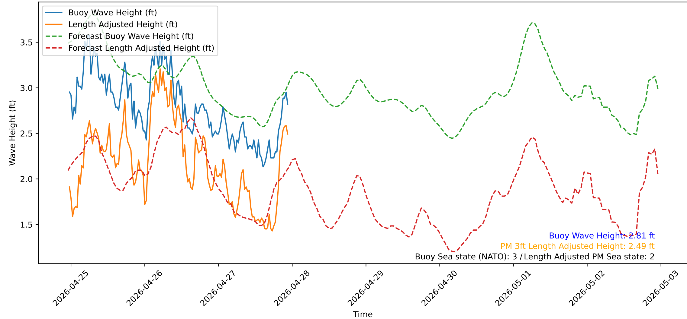
Wave Heights over Time for Green Beach at 2026-04-27 23:21:15
