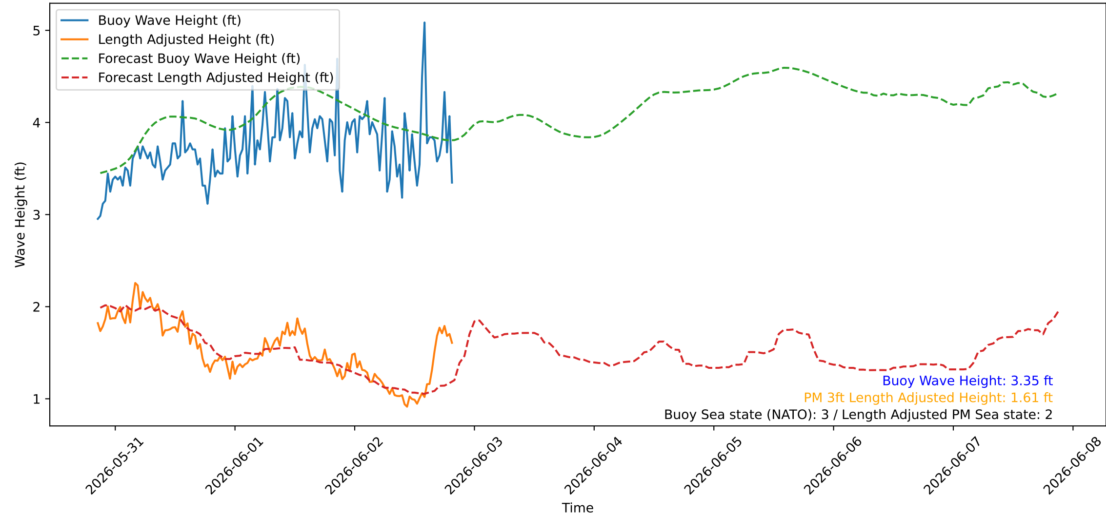
Wave Heights over Time for Oceanside Harbor at 2026-06-02 20:30:26
