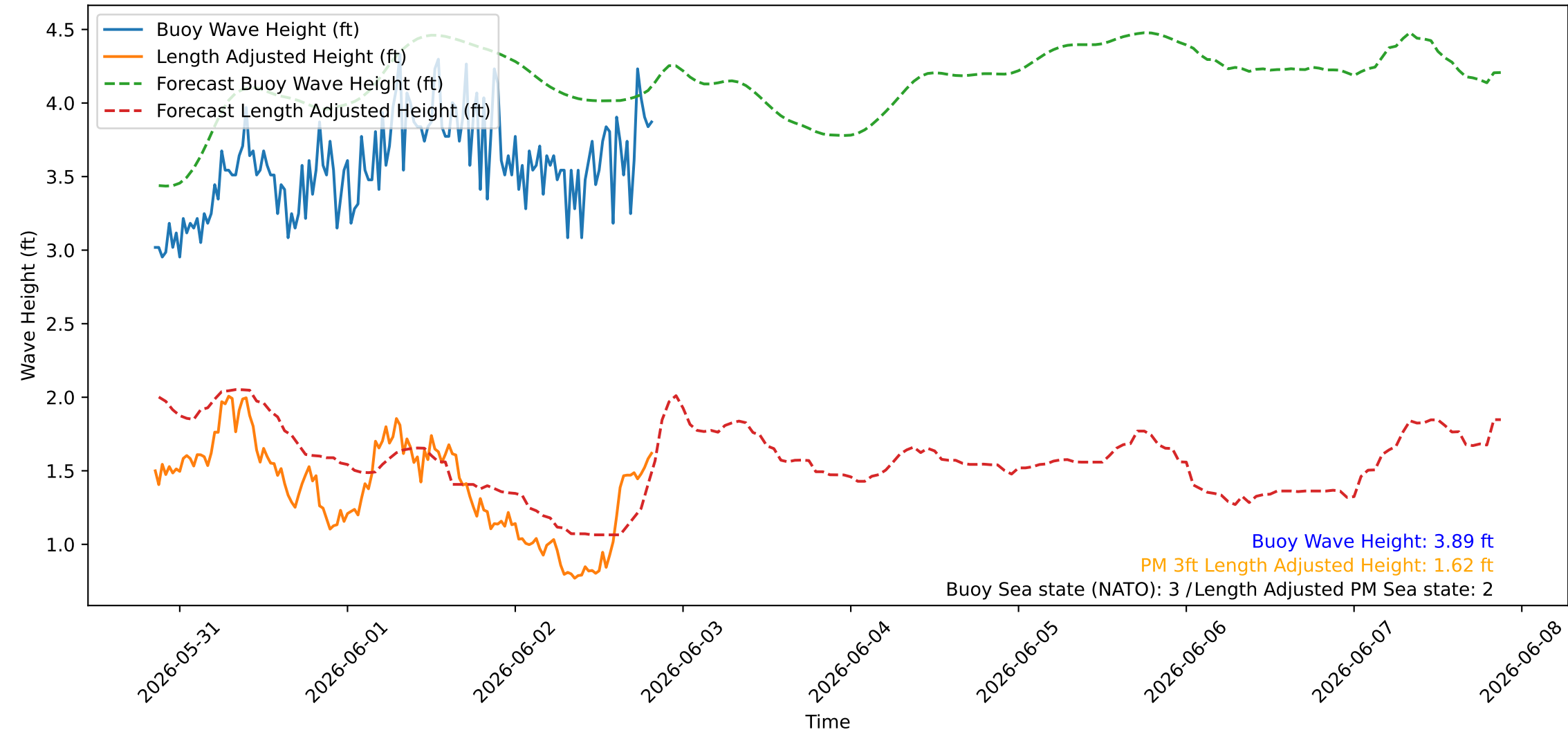
Wave Heights over Time for Green Beach at 2026-06-02 20:31:08
