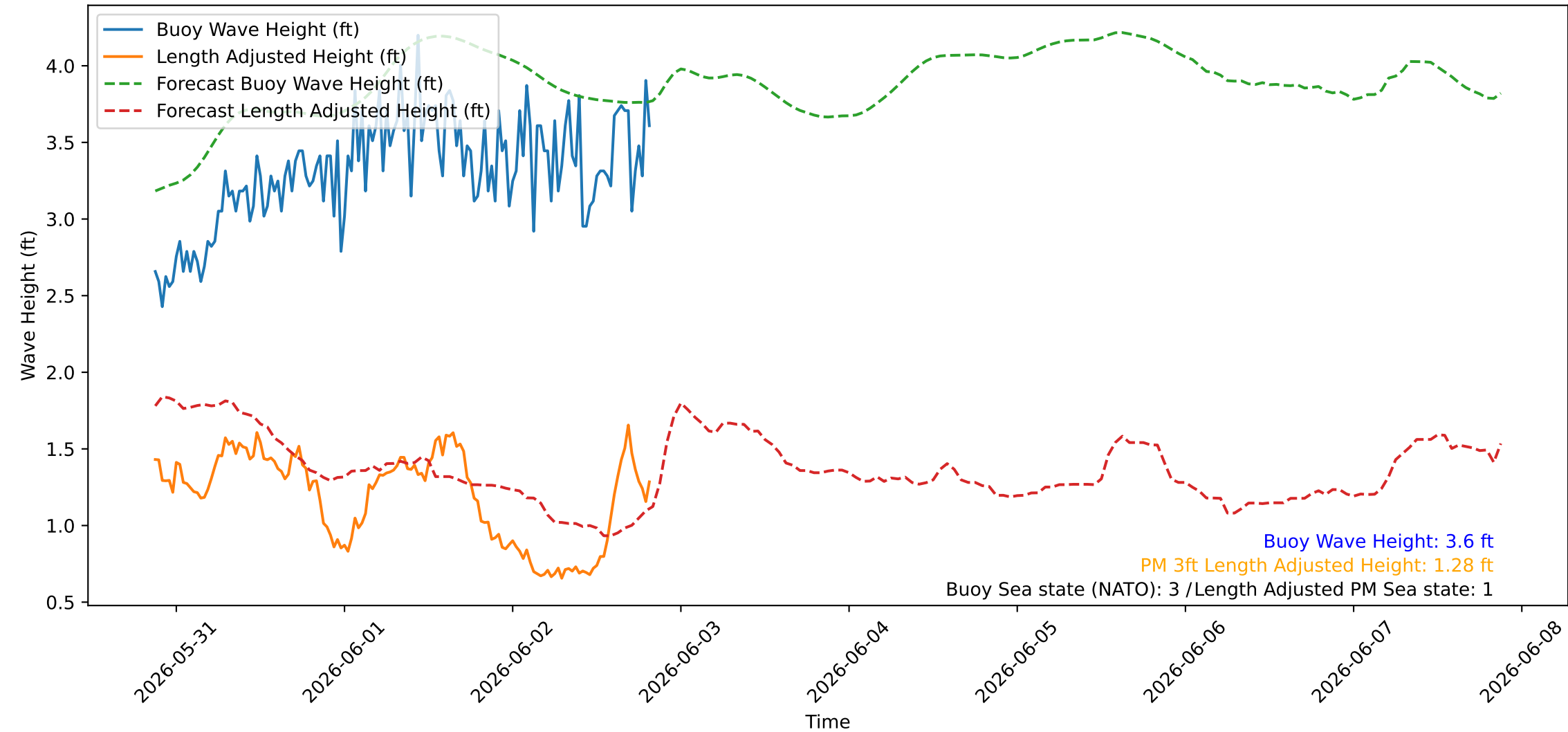
Wave Heights over Time for Red Beach at 2026-06-02 20:30:45
