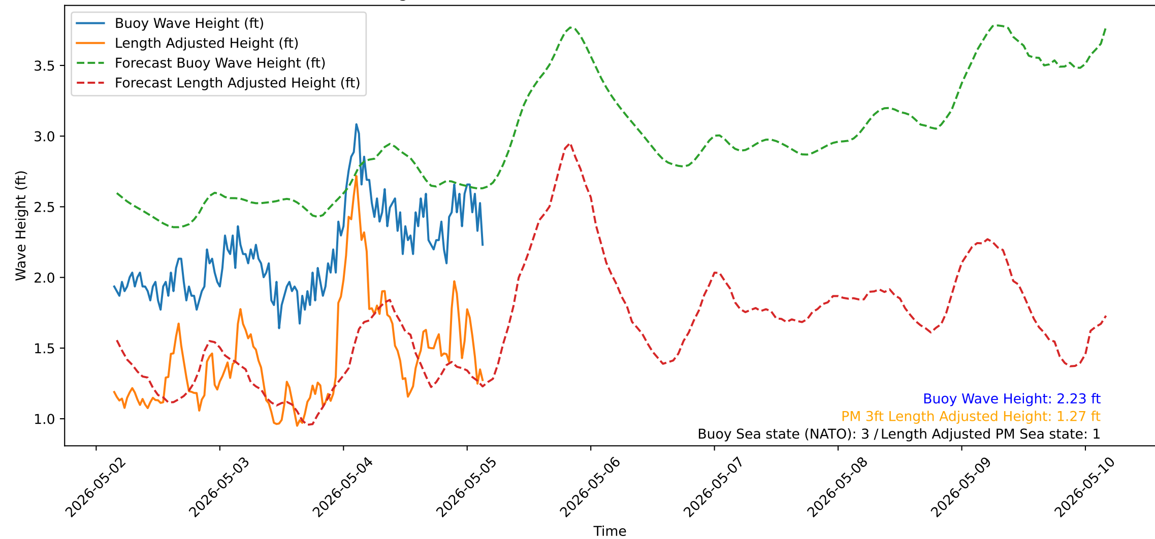
Wave Heights over Time for Oceanside Harbor at 2026-05-05 03:40:31
