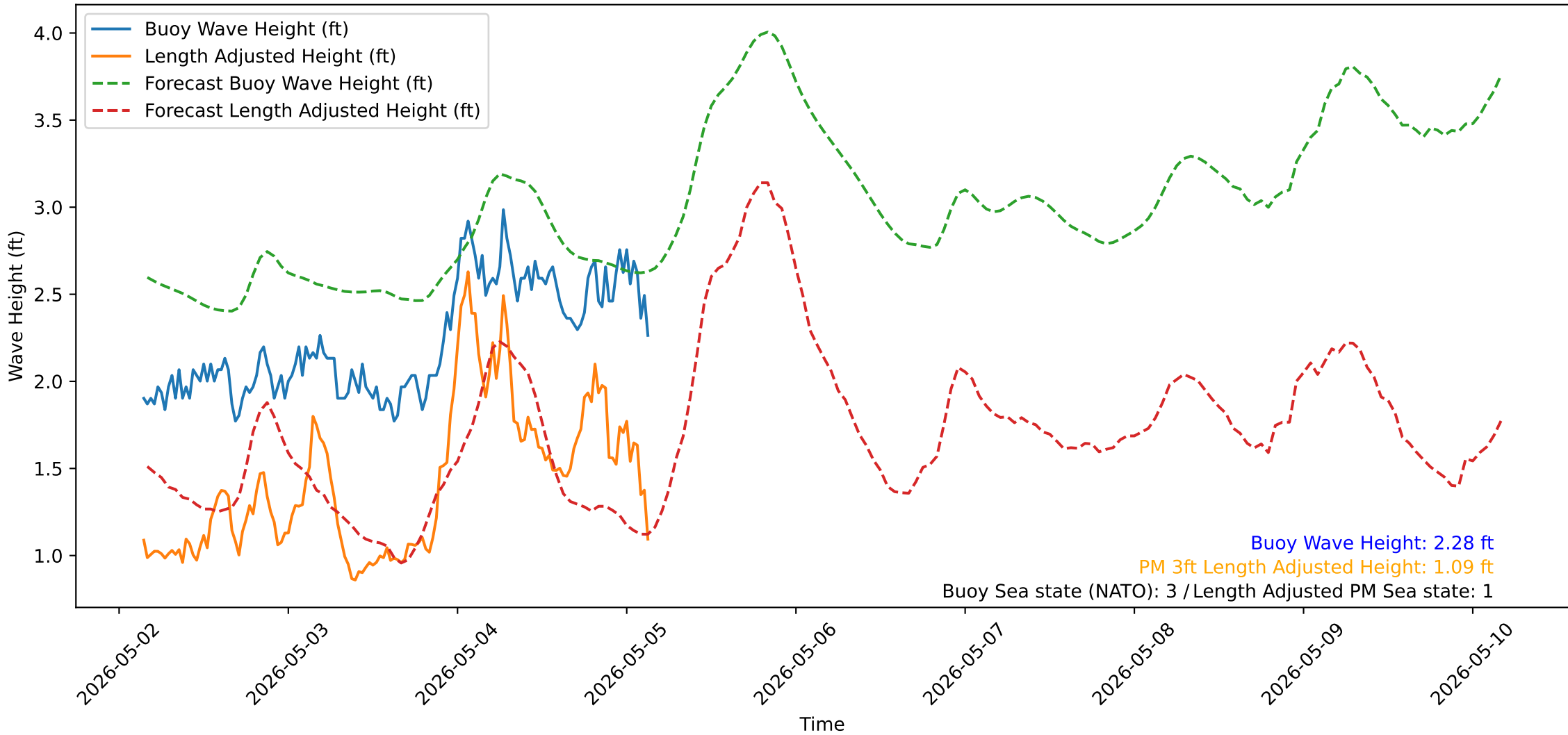
Wave Heights over Time for Green Beach at 2026-05-05 03:41:13
