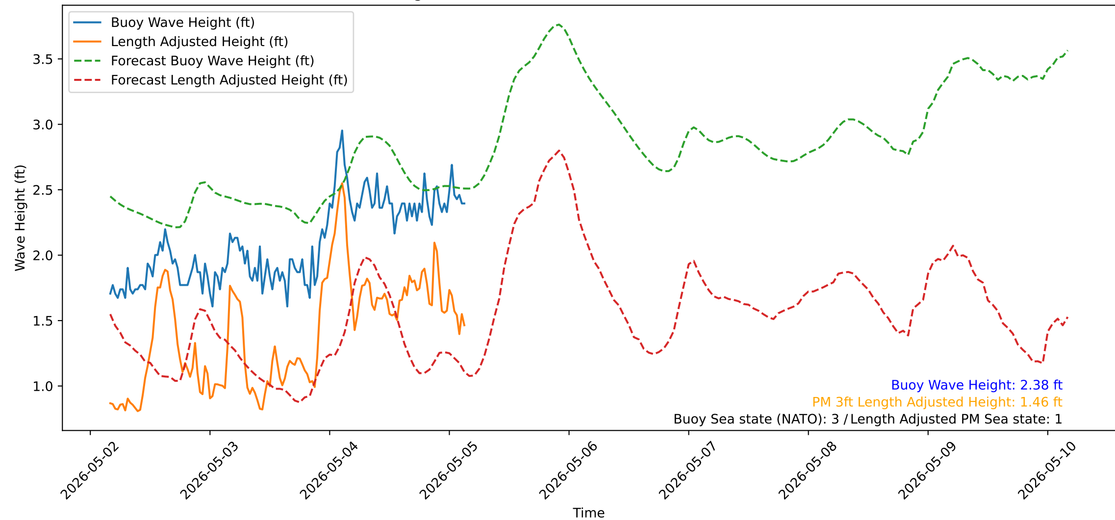
Wave Heights over Time for Red Beach at 2026-05-05 03:40:50
