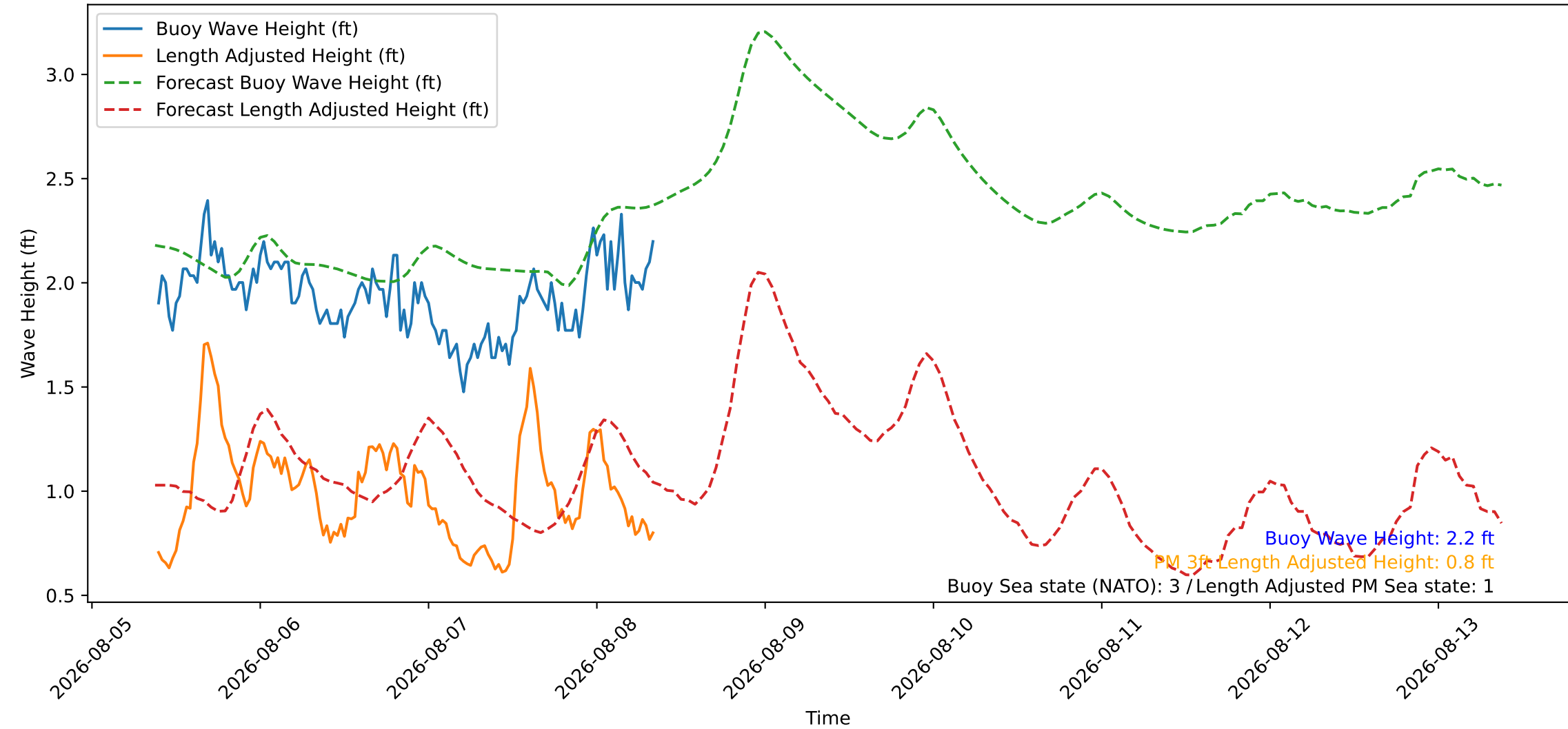
Wave Heights over Time for Red Beach at 2026-08-08 09:00:45
