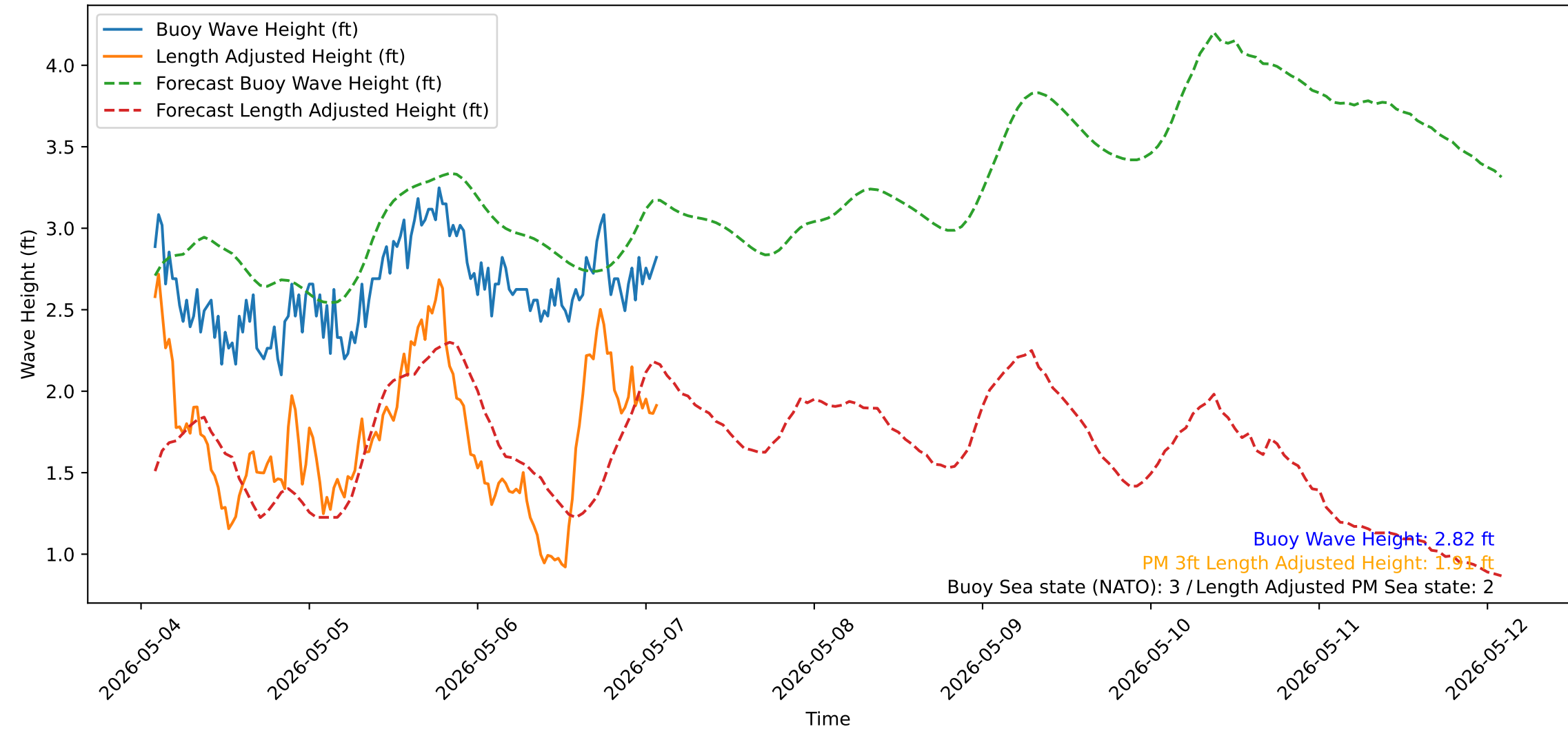
Wave Heights over Time for Oceanside Harbor at 2026-05-07 02:10:32
