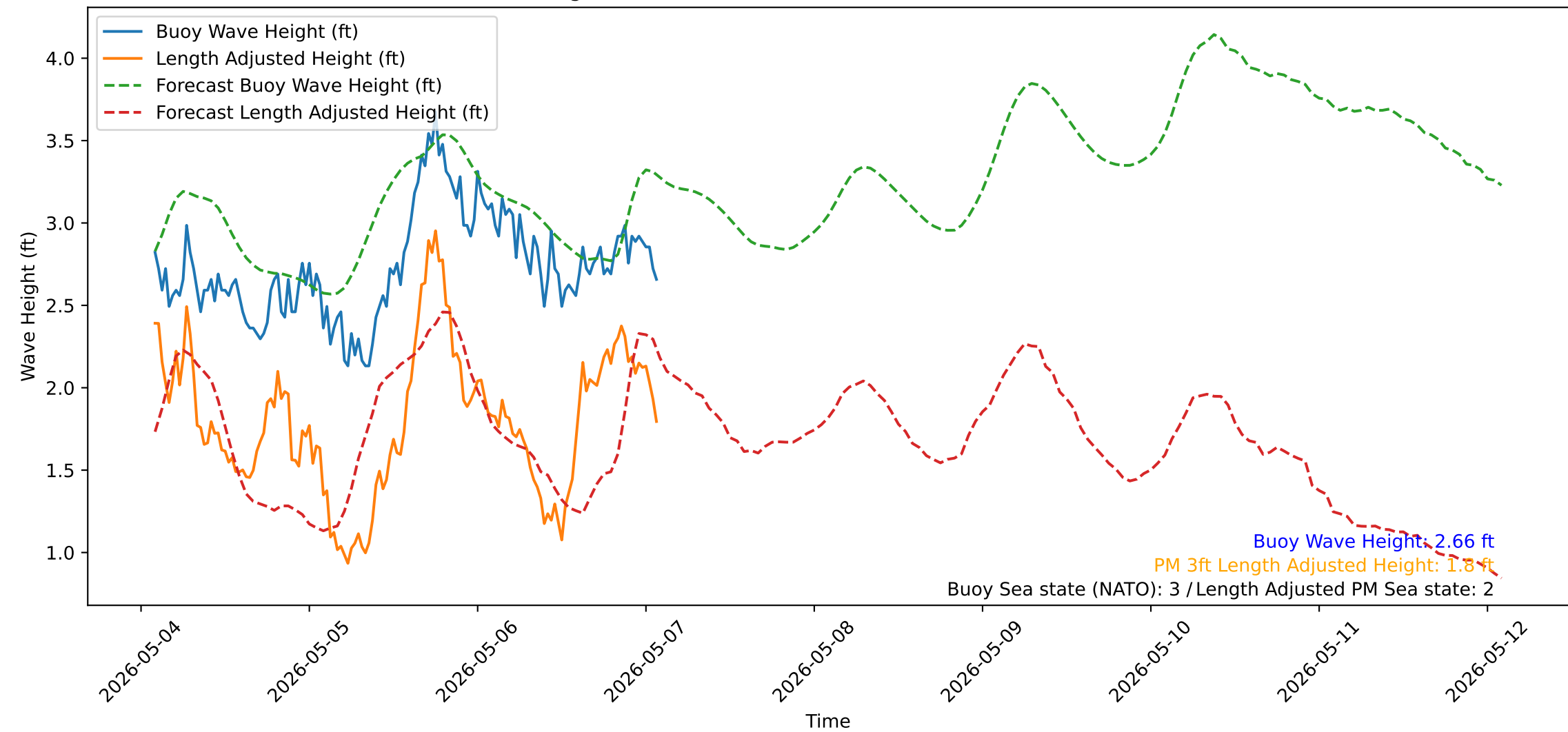
Wave Heights over Time for Green Beach at 2026-05-07 02:11:14
