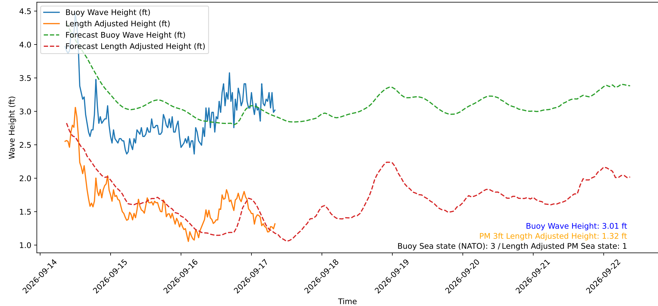
Wave Heights over Time for Oceanside Harbor at 2026-09-17 08:40:30
