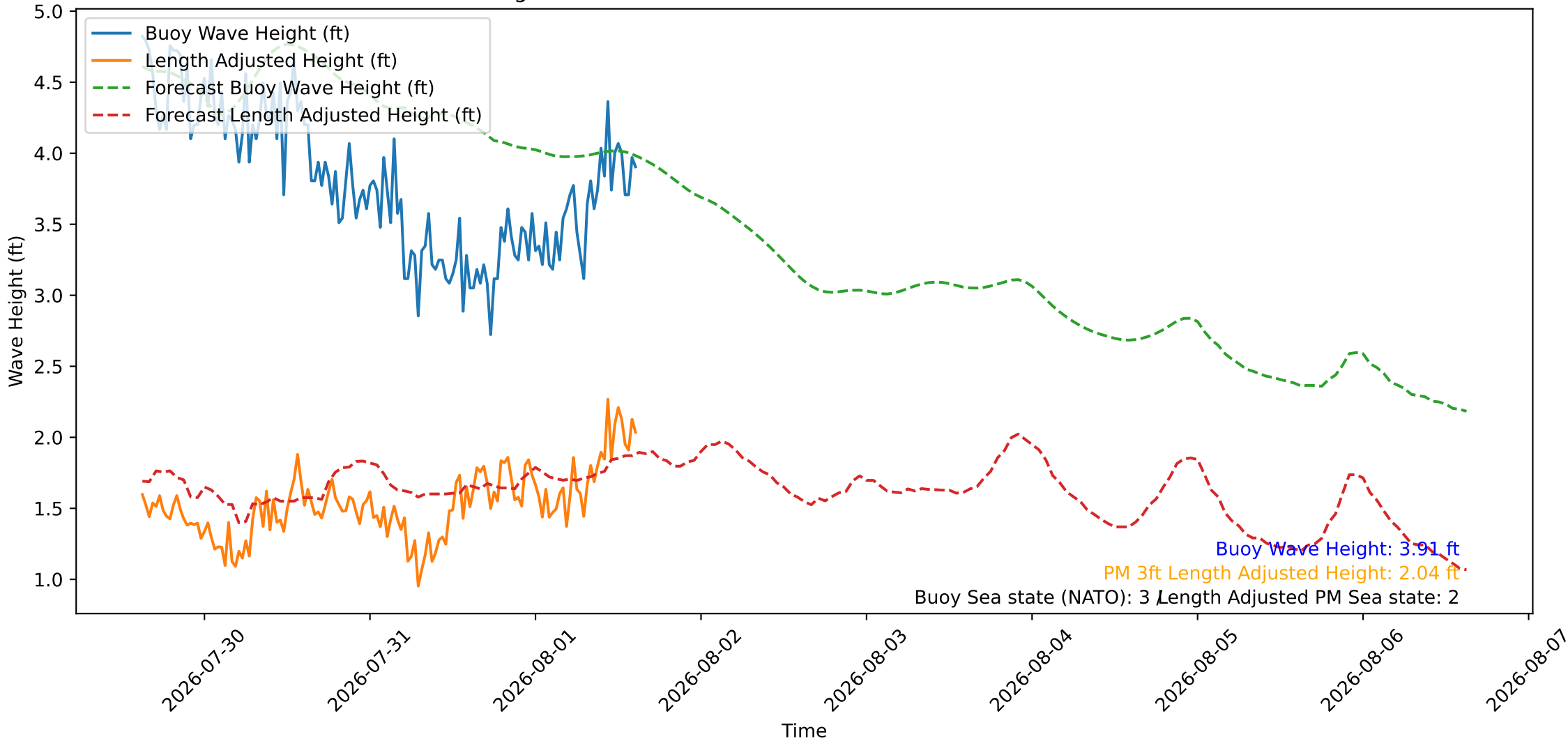
Wave Heights over Time for Oceanside Harbor at 2026-08-01 15:10:27
