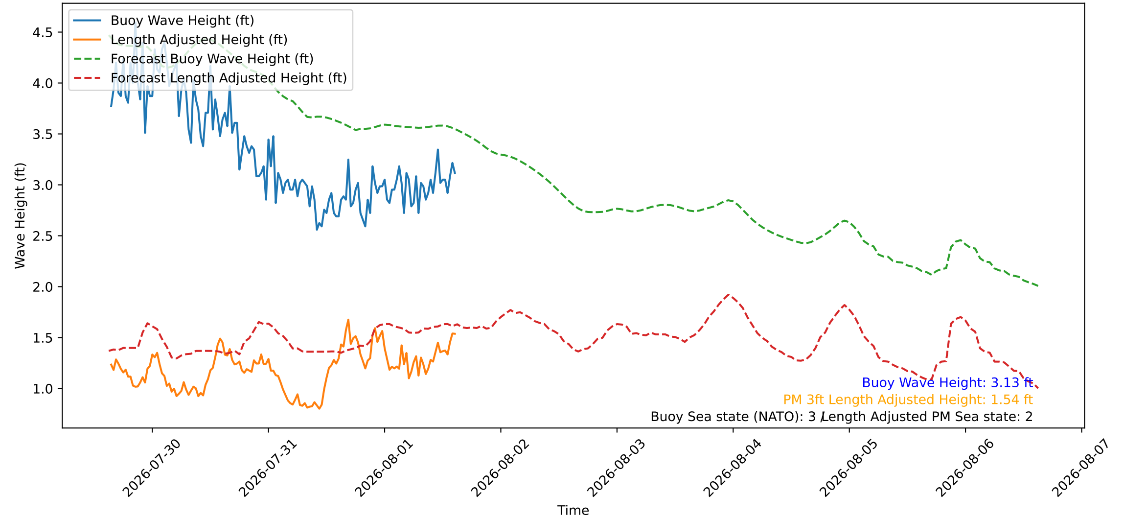
Wave Heights over Time for Red Beach at 2026-08-01 15:10:46
