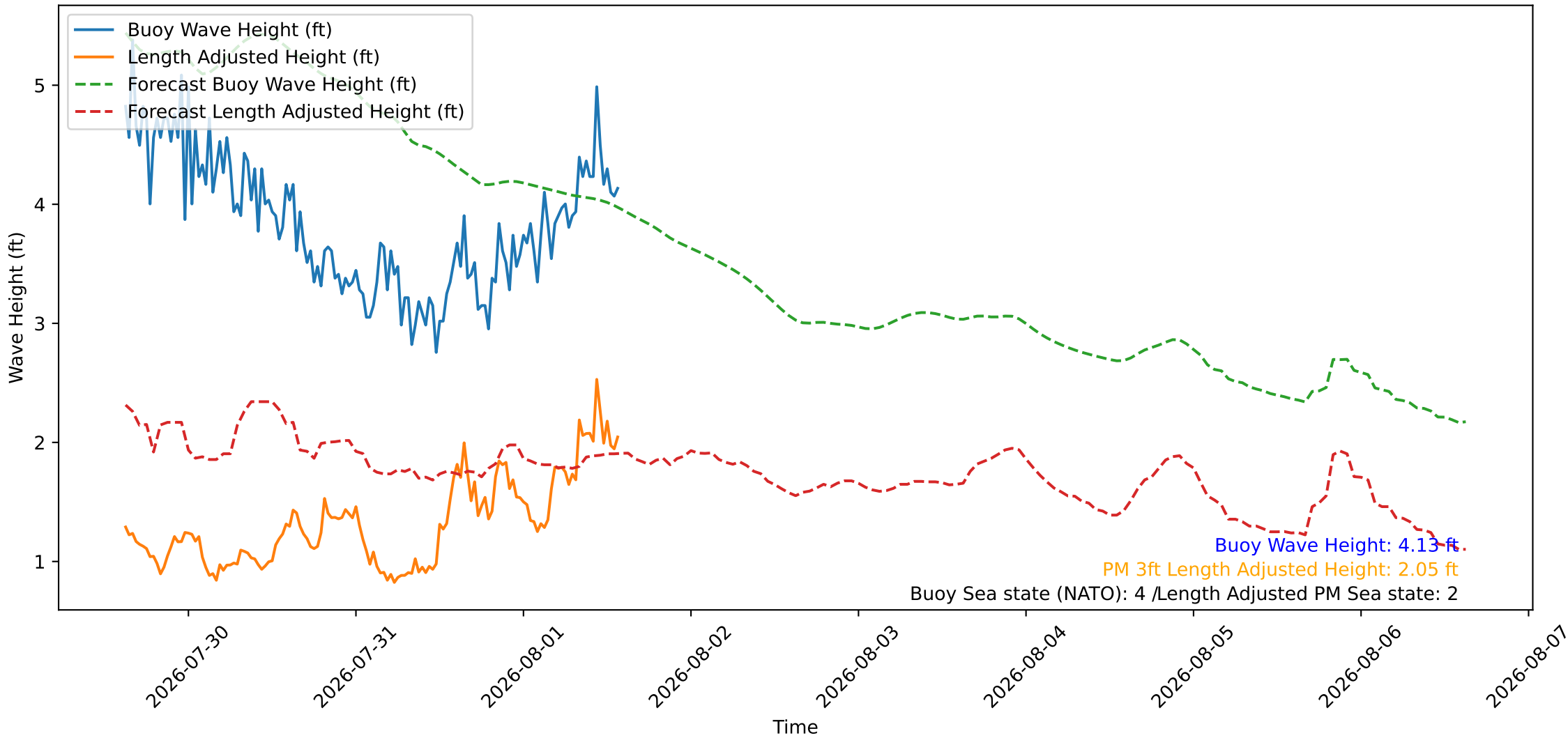
Wave Heights over Time for Green Beach at 2026-08-01 15:11:09
