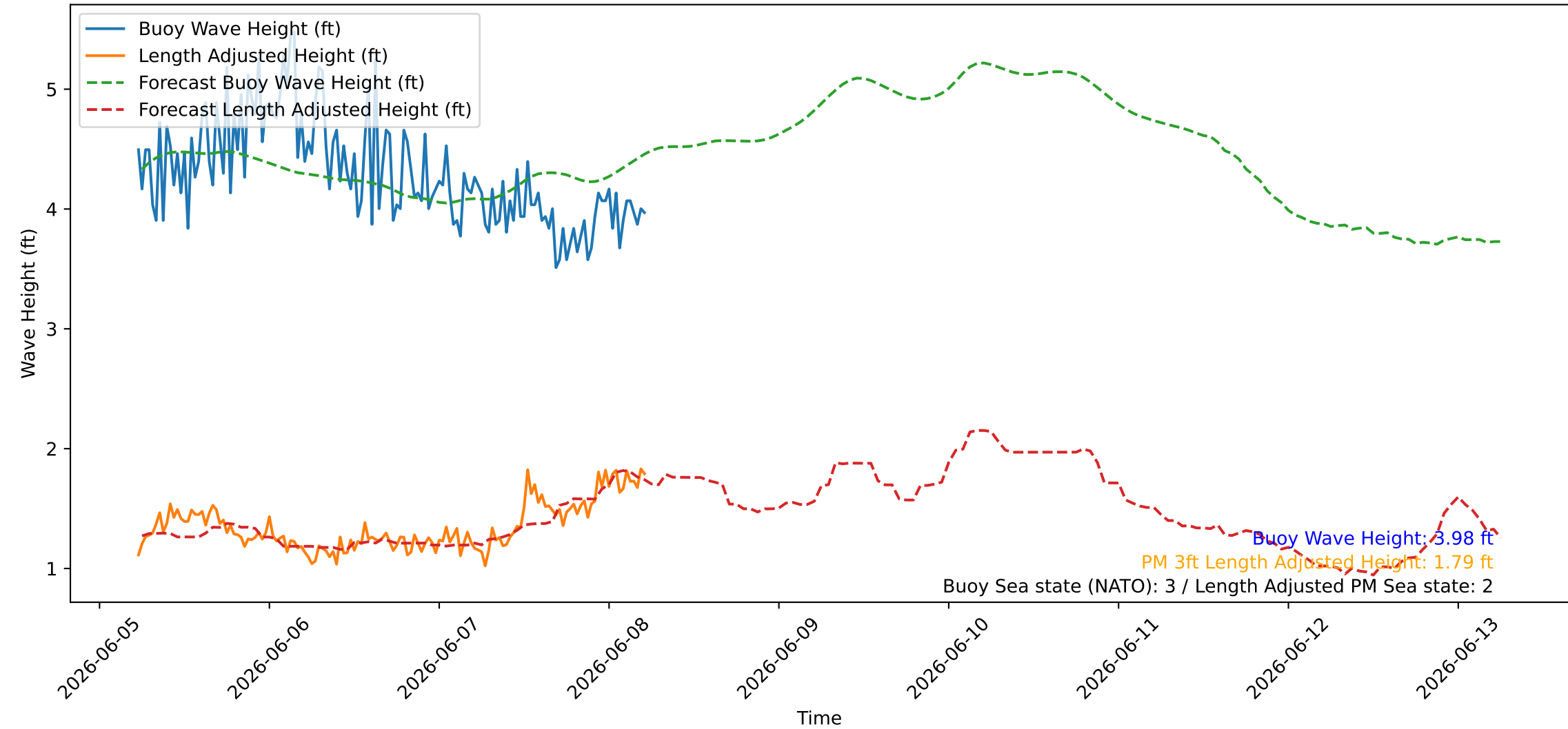
Wave Heights over Time for Oceanside Harbor at 2026-06-08 05:40:26
