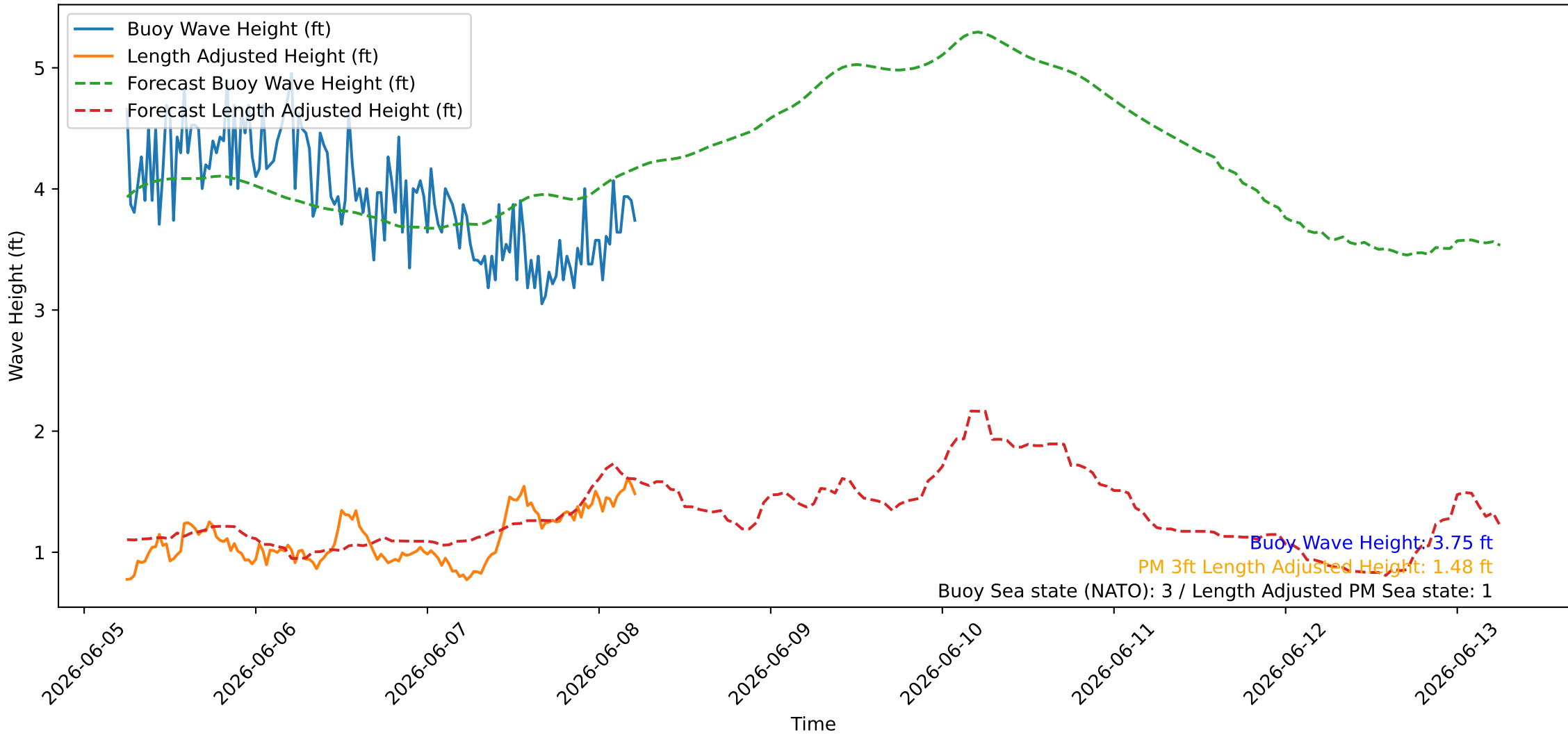
Wave Heights over Time for Red Beach at 2026-06-08 05:40:45
