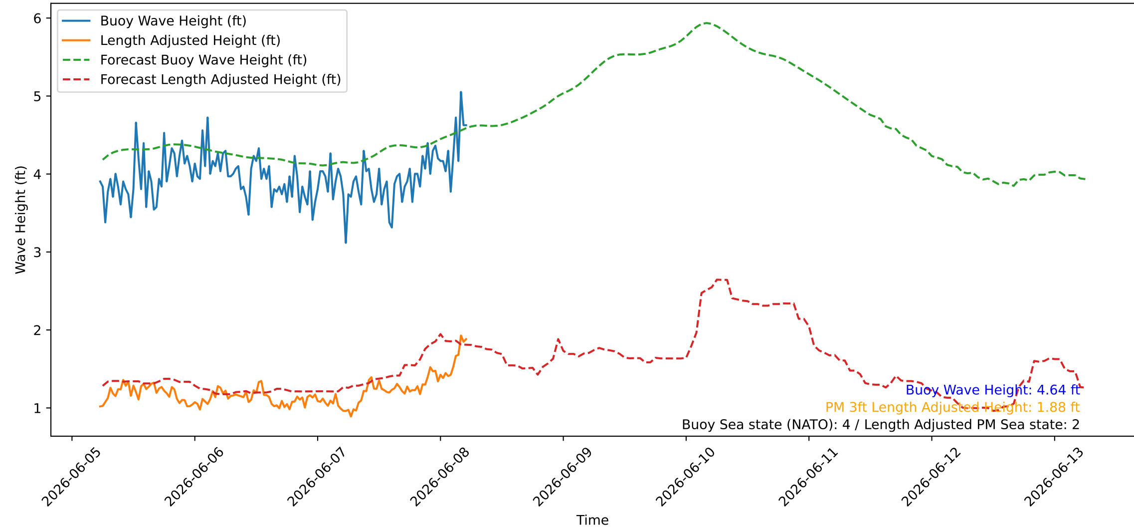
Wave Heights over Time for Green Beach at 2026-06-08 05:41:07
