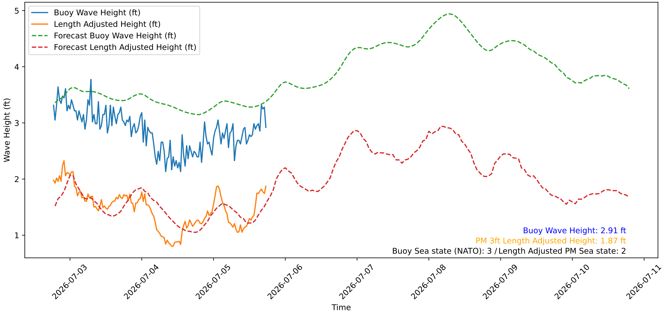
Wave Heights over Time for Oceanside Harbor at 2026-07-05 18:30:27
