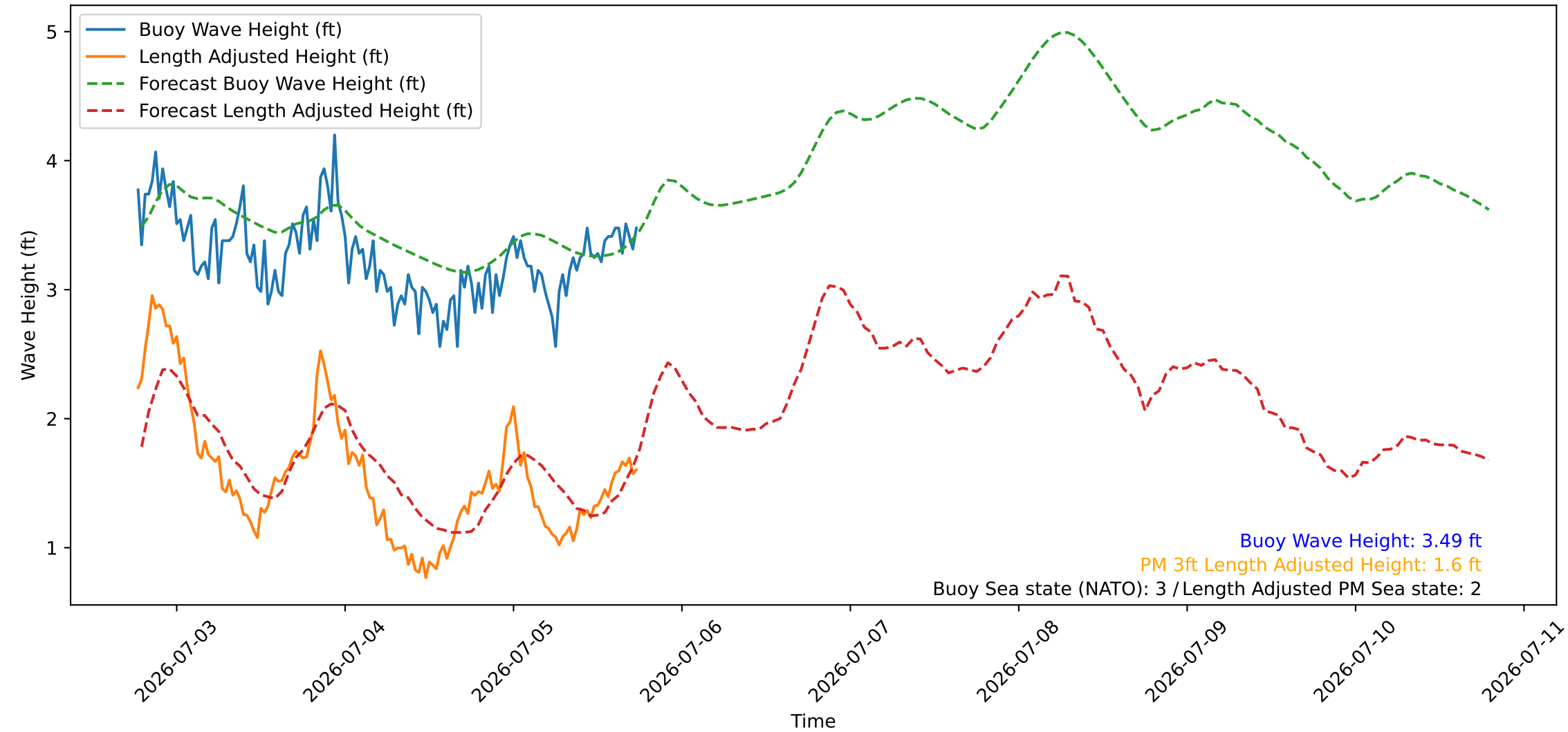
Wave Heights over Time for Green Beach at 2026-07-05 18:31:08
