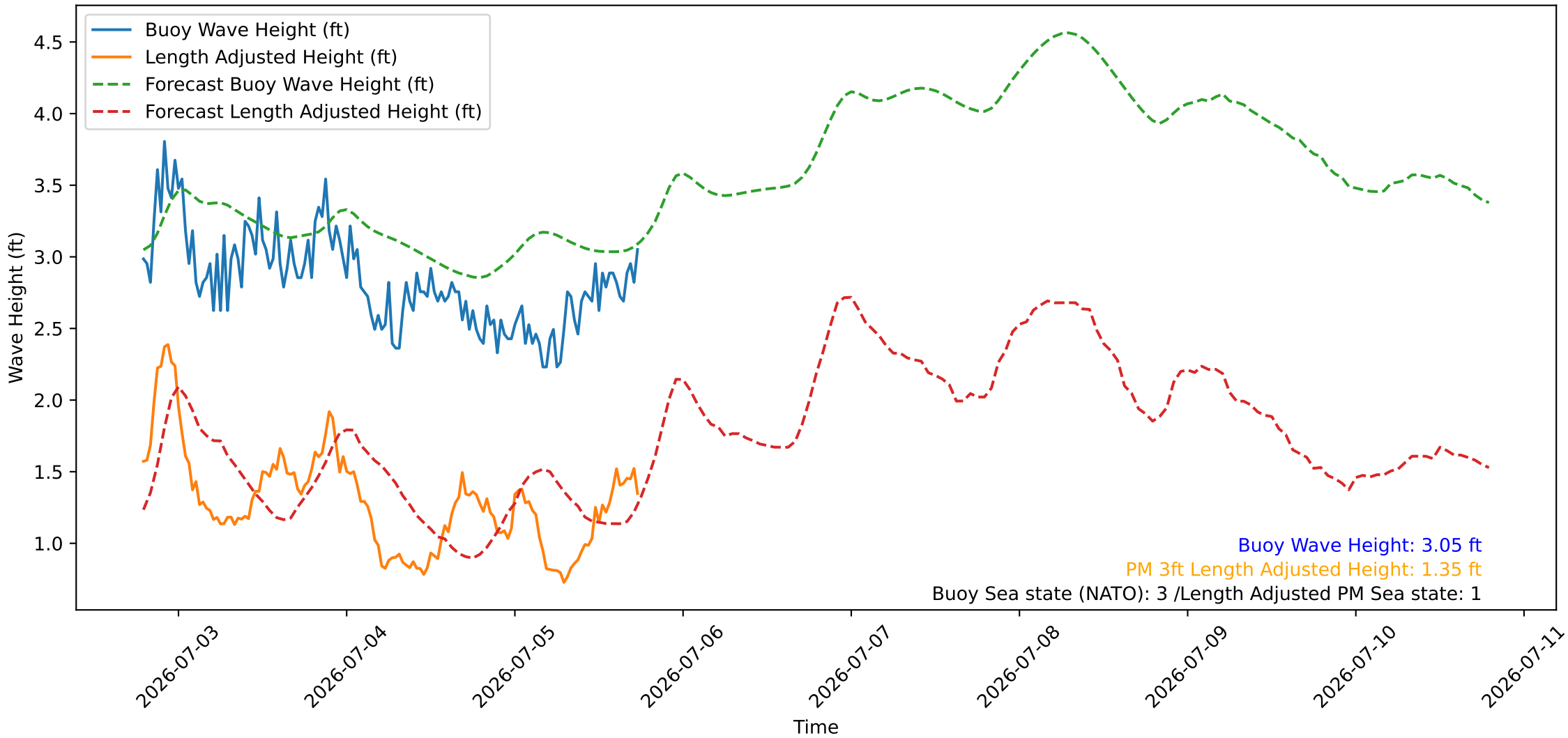
Wave Heights over Time for Red Beach at 2026-07-05 18:30:46
