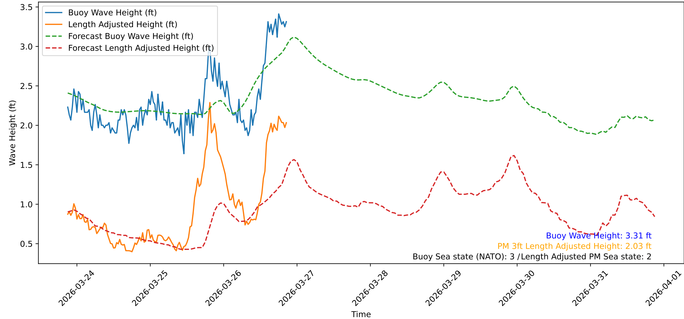
Wave Heights over Time for Green Beach at 2026-03-26 21:11:10
