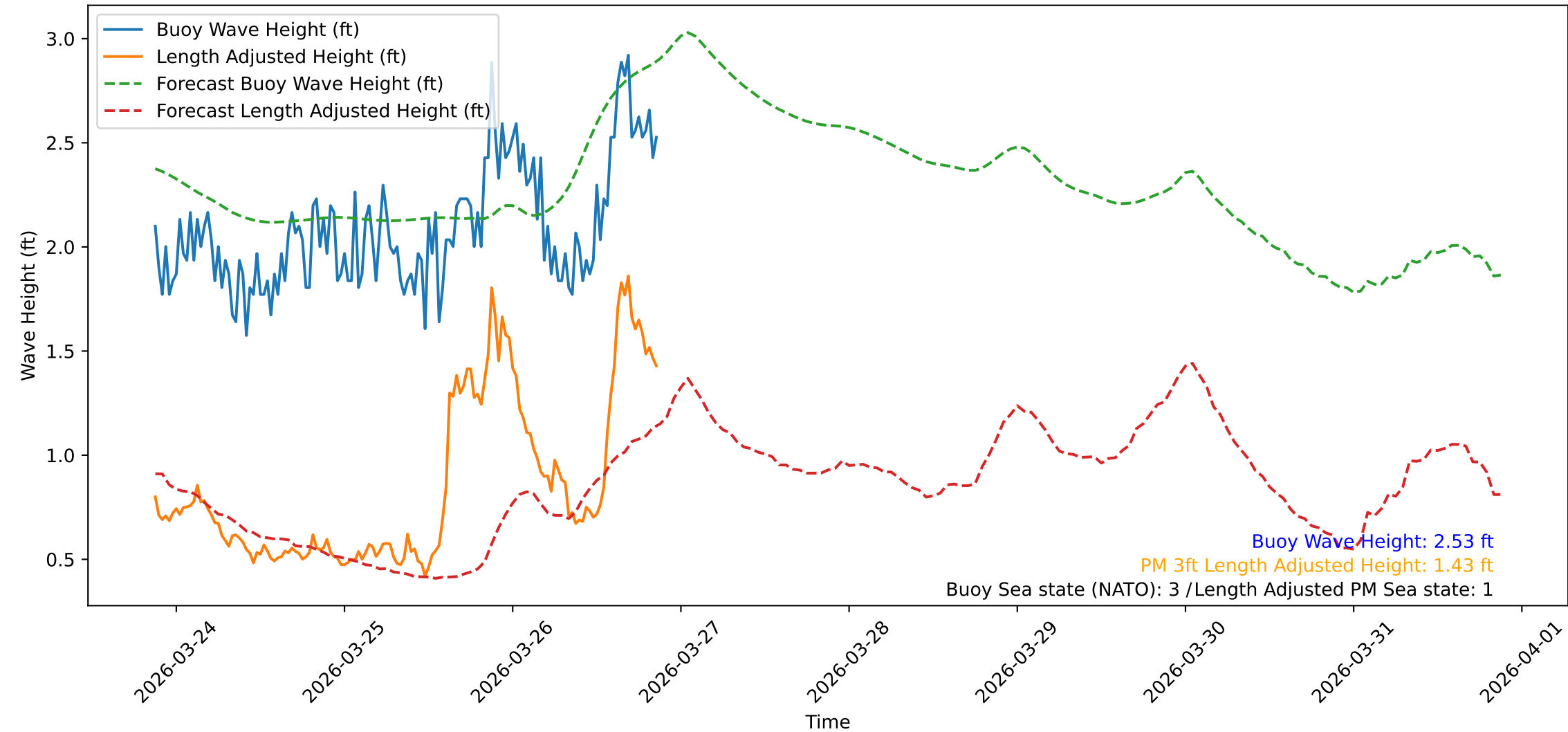
Wave Heights over Time for Oceanside Harbor at 2026-03-26 21:10:32
