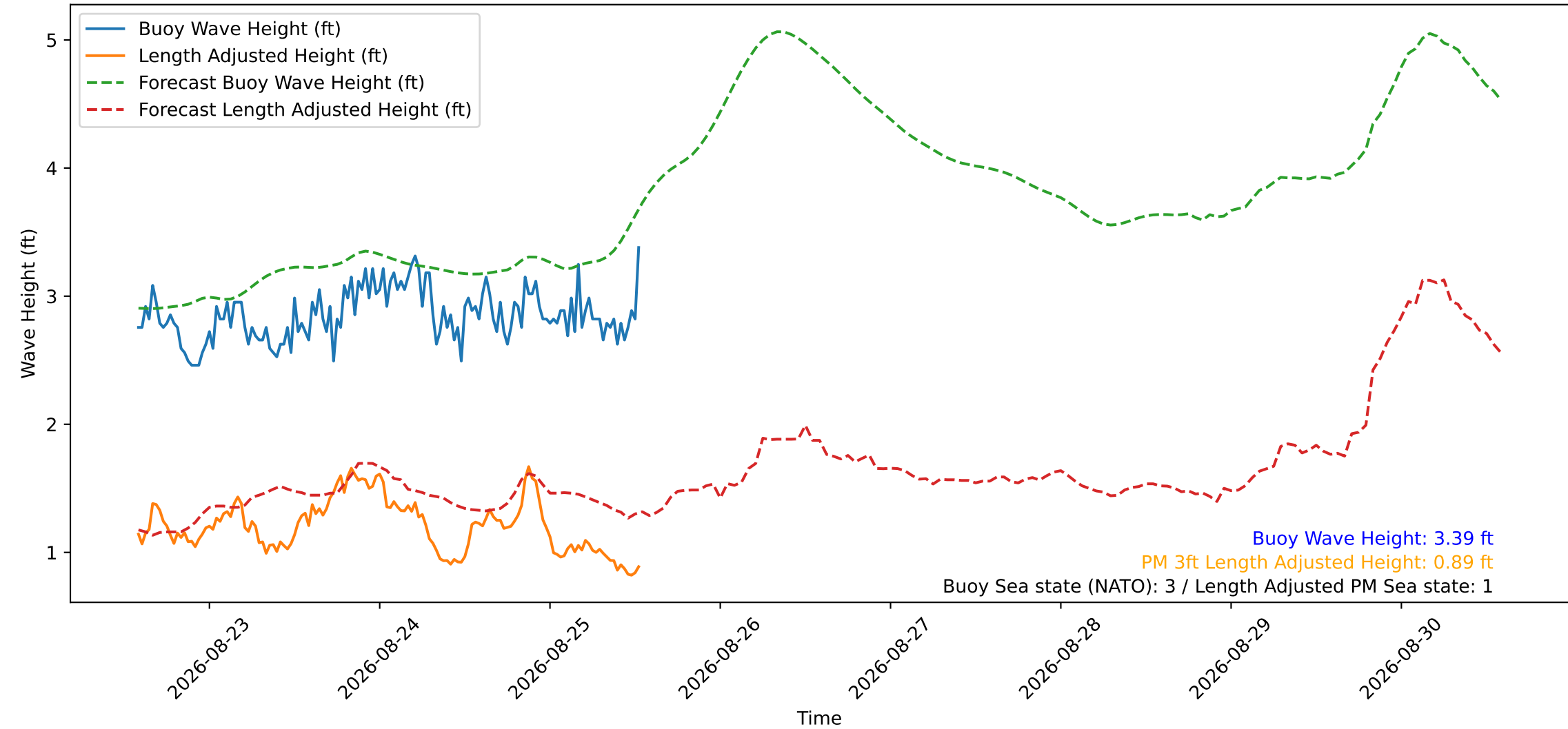
Wave Heights over Time for Green Beach at 2026-08-25 13:31:13
