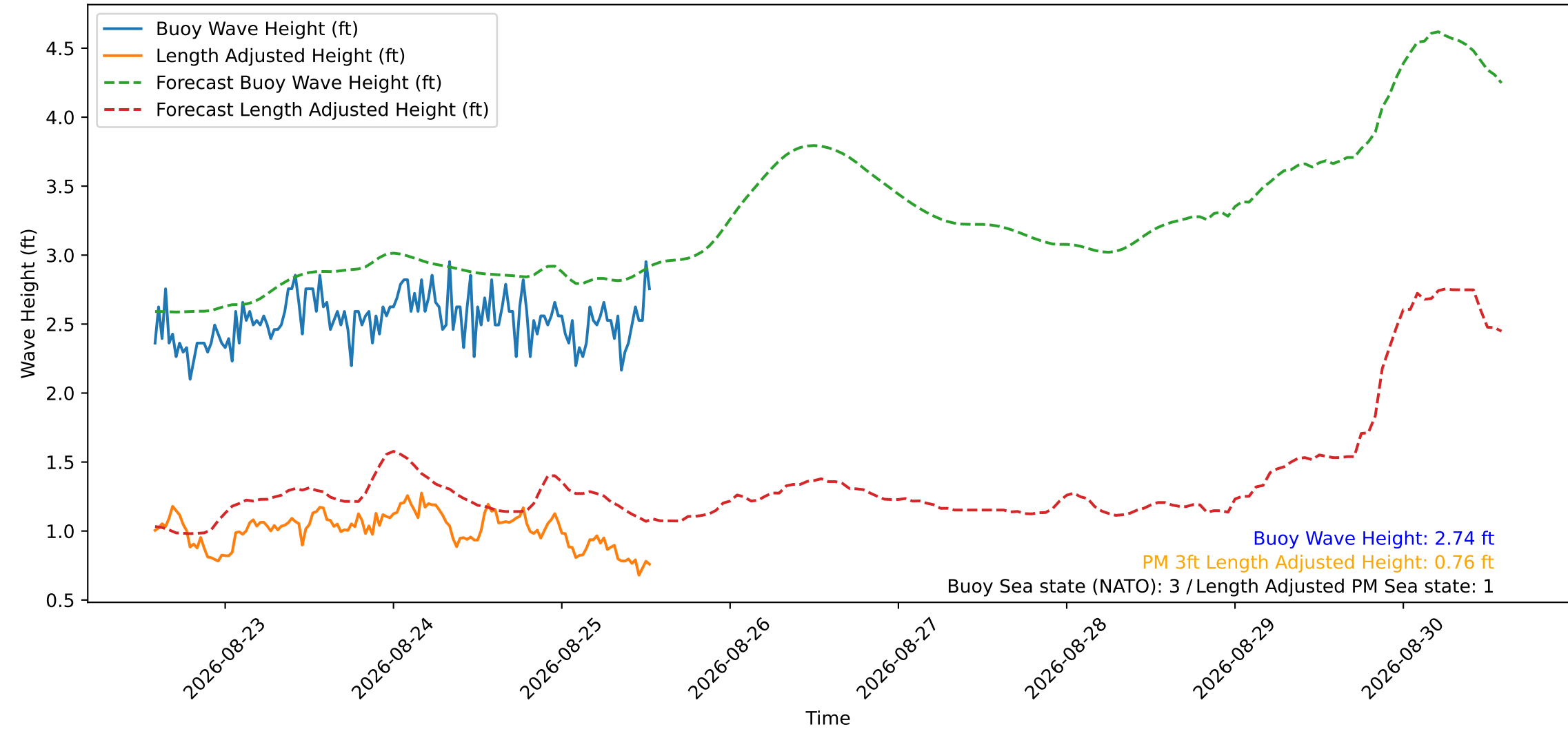
Wave Heights over Time for Red Beach at 2026-08-25 13:30:50
