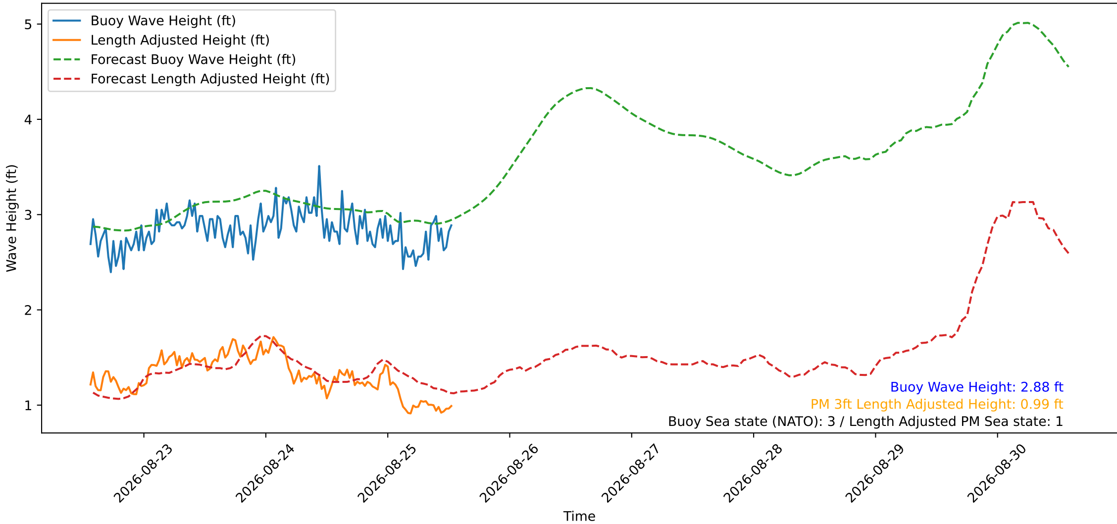
Wave Heights over Time for Oceanside Harbor at 2026-08-25 13:30:30
