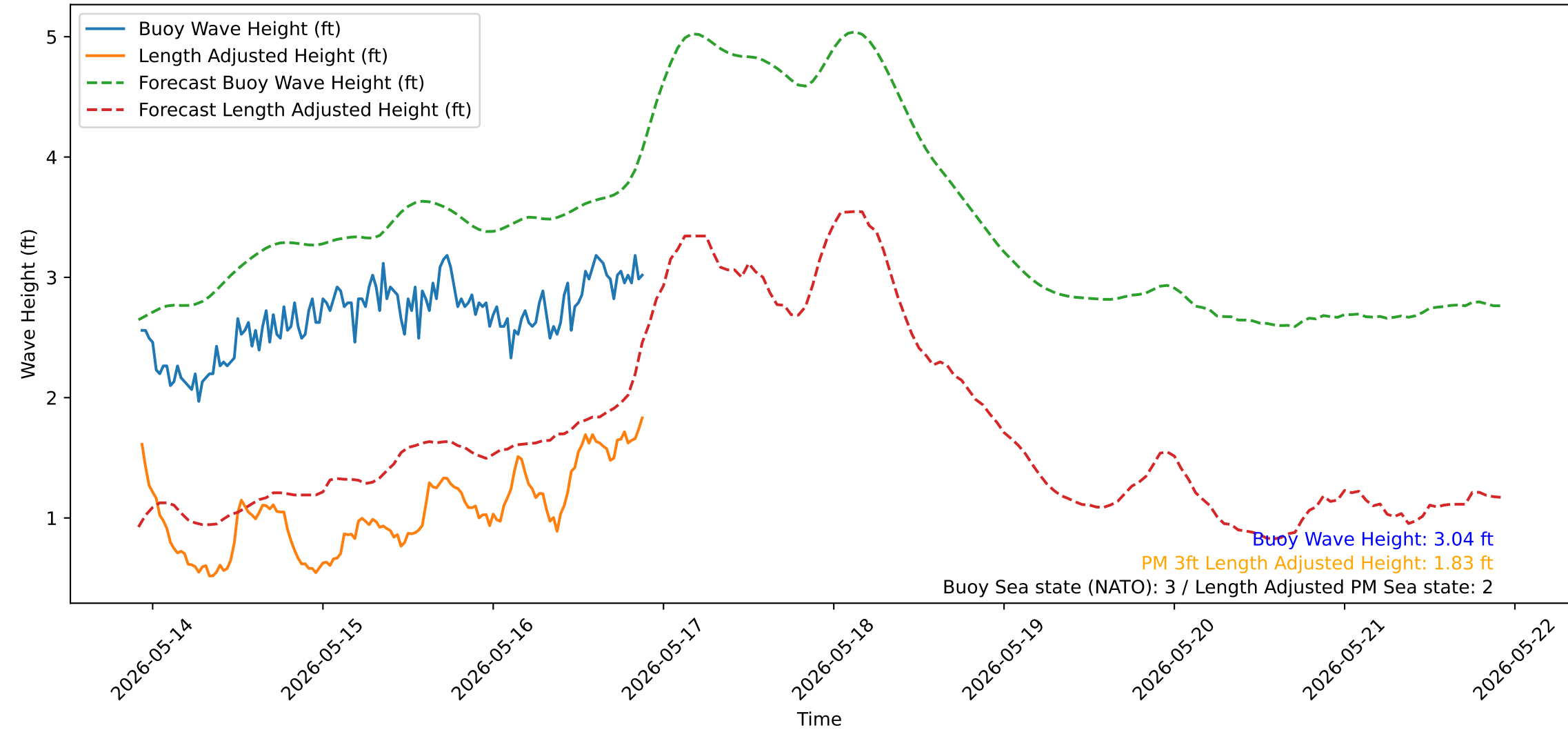
Wave Heights over Time for Red Beach at 2026-05-16 22:10:51
