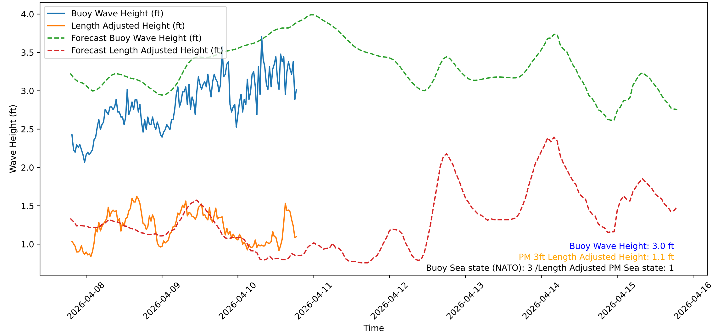
Wave Heights over Time for Red Beach at 2026-04-10 19:10:51
