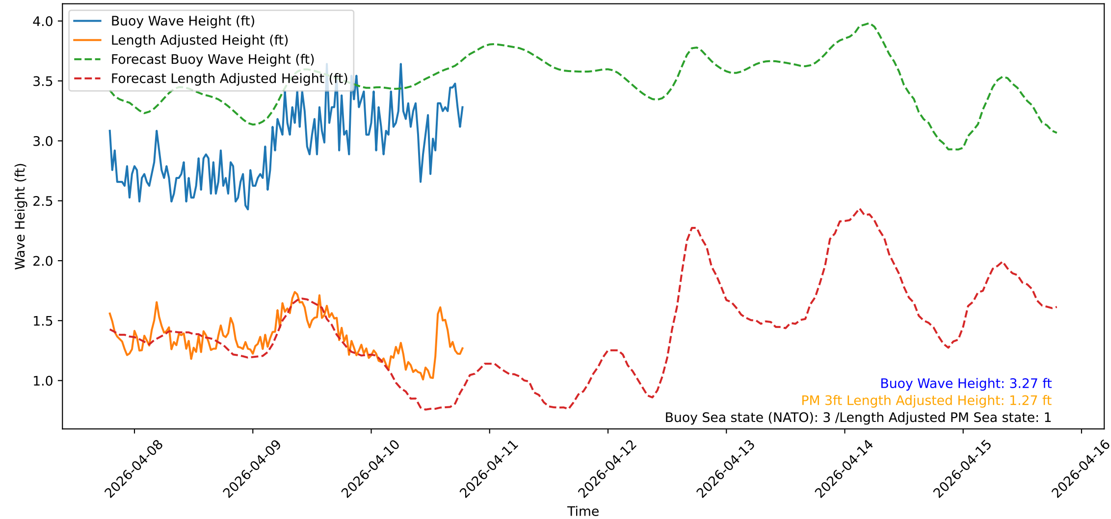
Wave Heights over Time for Oceanside Harbor at 2026-04-10 19:10:32
