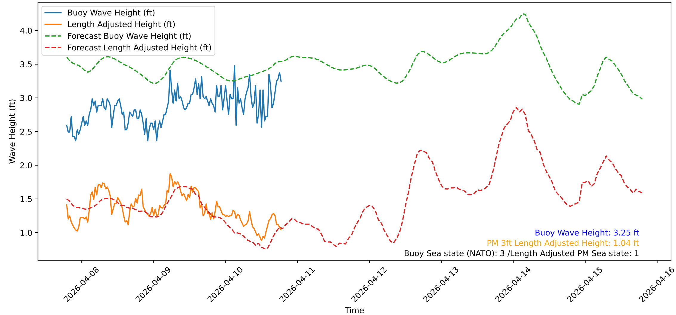
Wave Heights over Time for Green Beach at 2026-04-10 19:11:13
