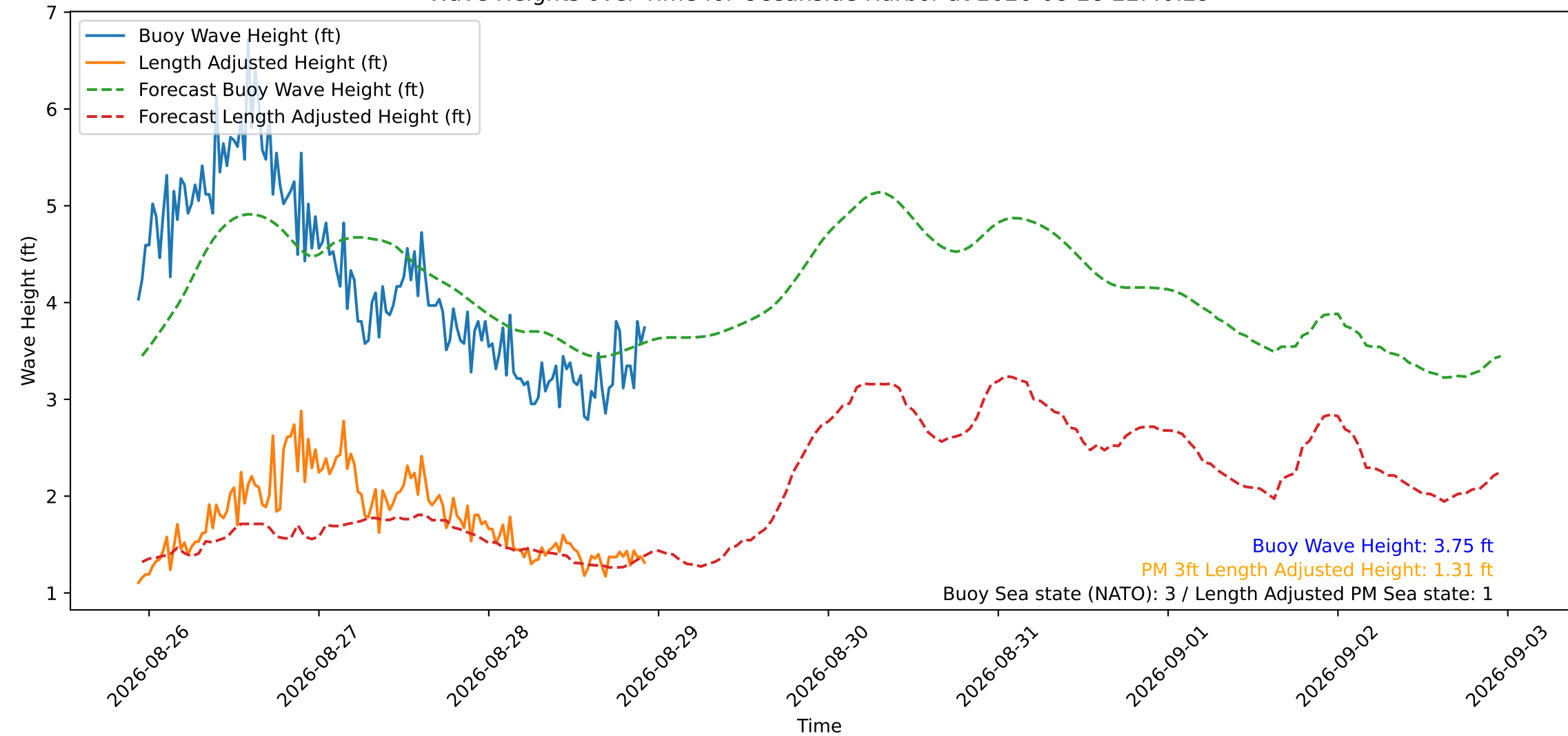
Wave Heights over Time for Oceanside Harbor at 2026-08-28 22:40:29
