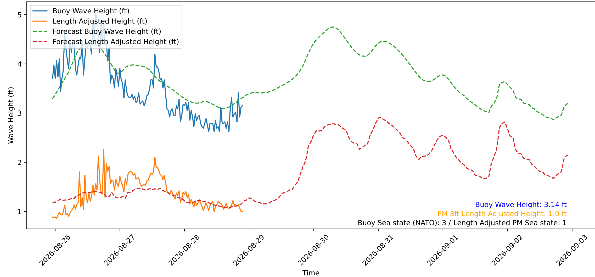
Wave Heights over Time for Red Beach at 2026-08-28 22:40:49
