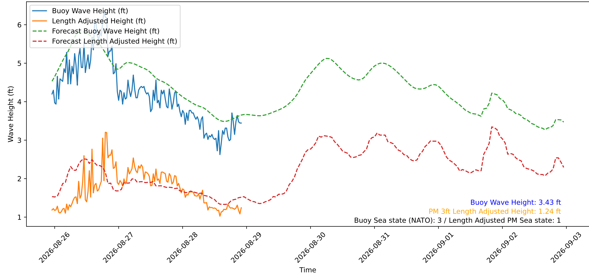
Wave Heights over Time for Green Beach at 2026-08-28 22:41:12
