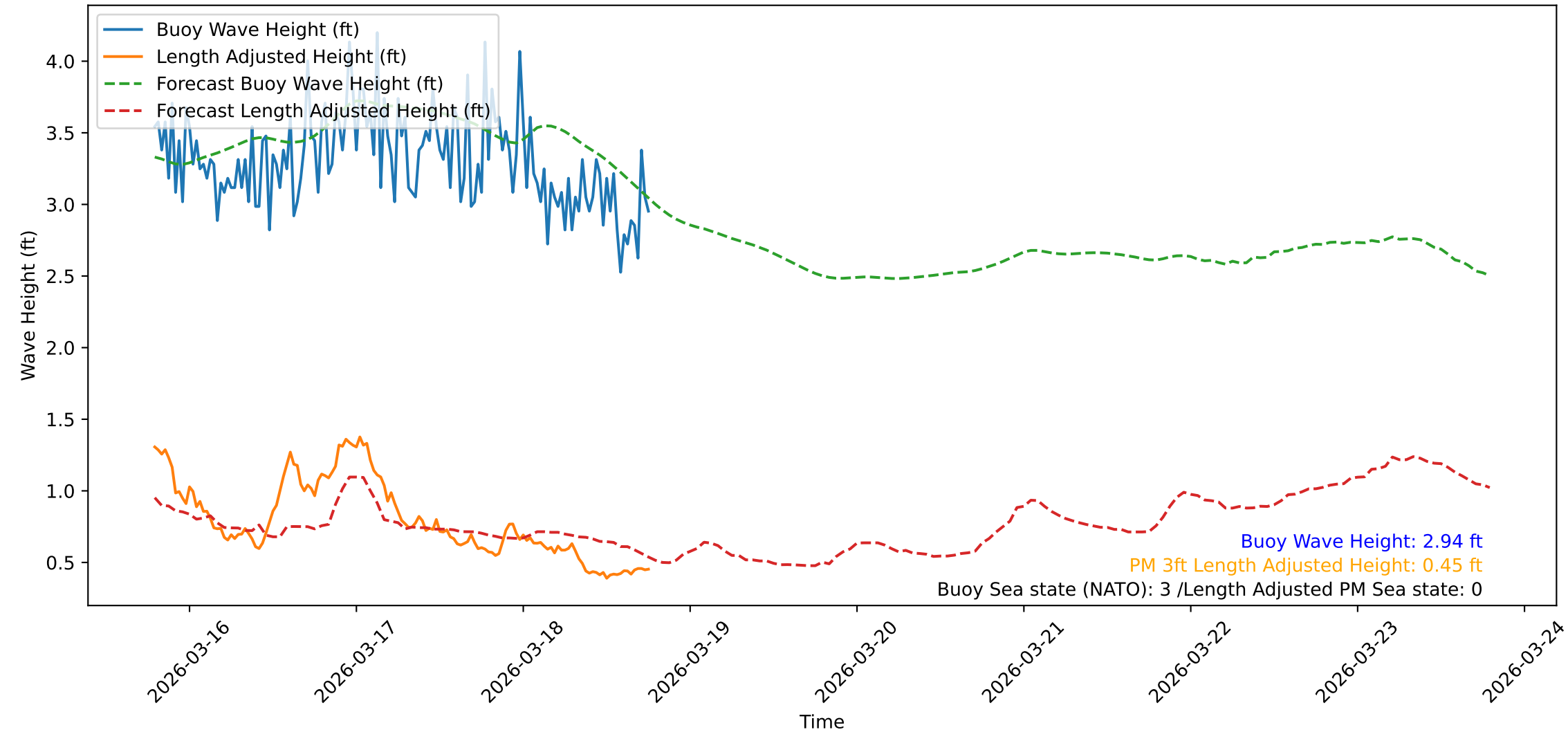
Wave Heights over Time for Green Beach at 2026-03-18 18:51:09
