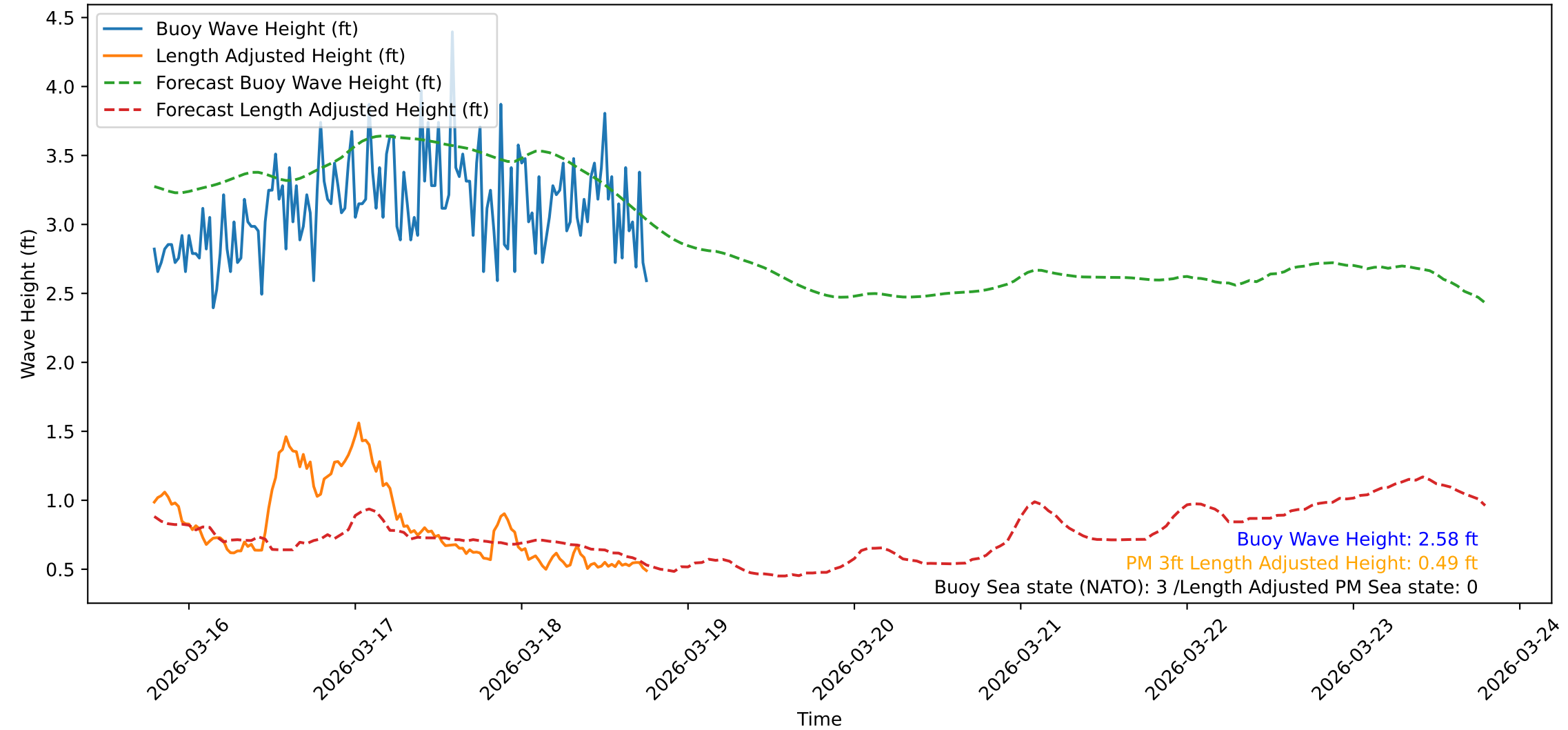
Wave Heights over Time for Oceanside Harbor at 2026-03-18 18:50:31
