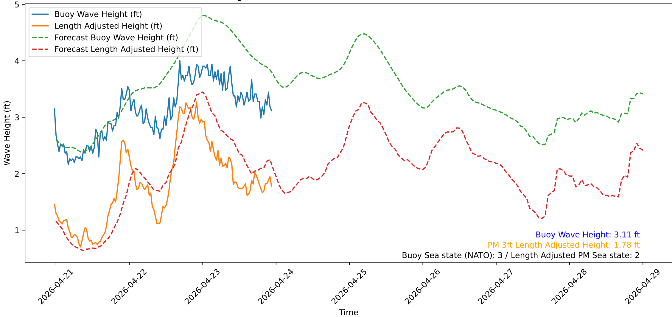
Wave Heights over Time for Green Beach at 2026-04-23 23:31:12
