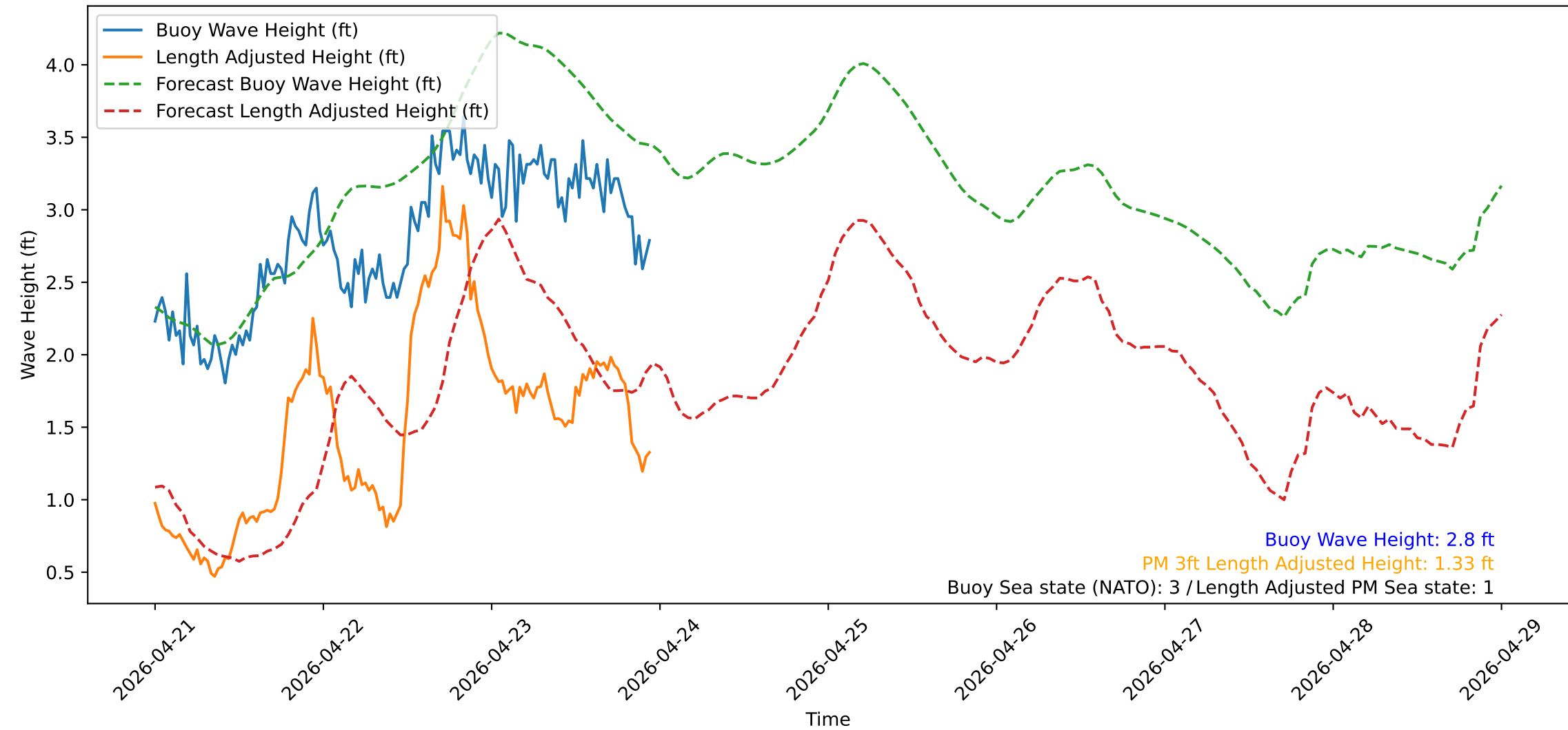
Wave Heights over Time for Red Beach at 2026-04-23 23:30:50
