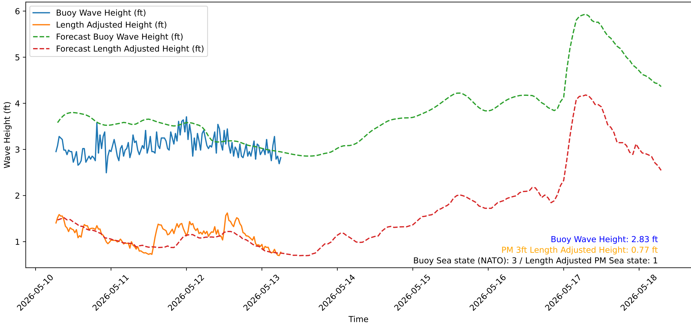
Wave Heights over Time for Oceanside Harbor at 2026-05-13 06:40:31
