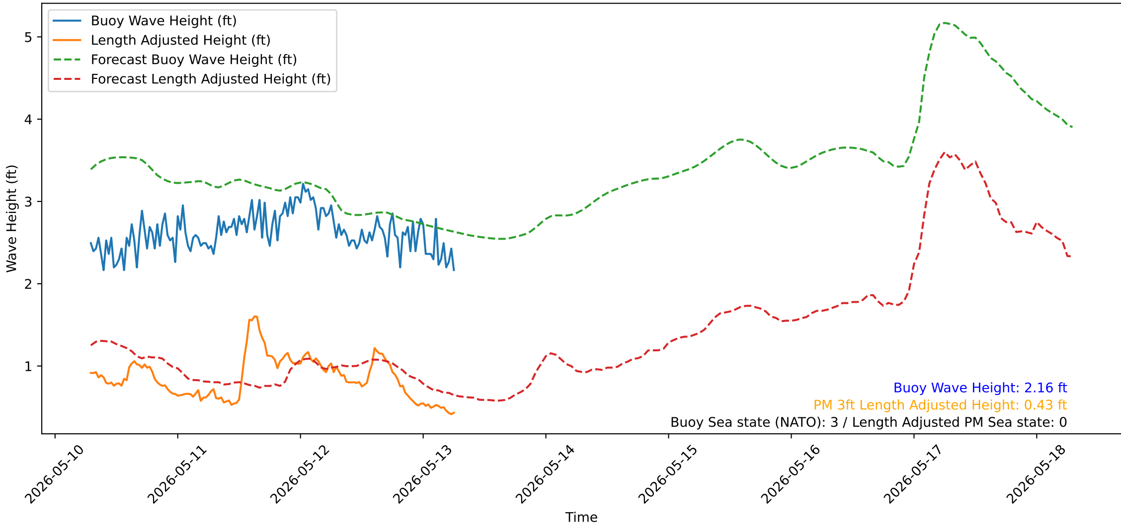
Wave Heights over Time for Red Beach at 2026-05-13 06:40:50
