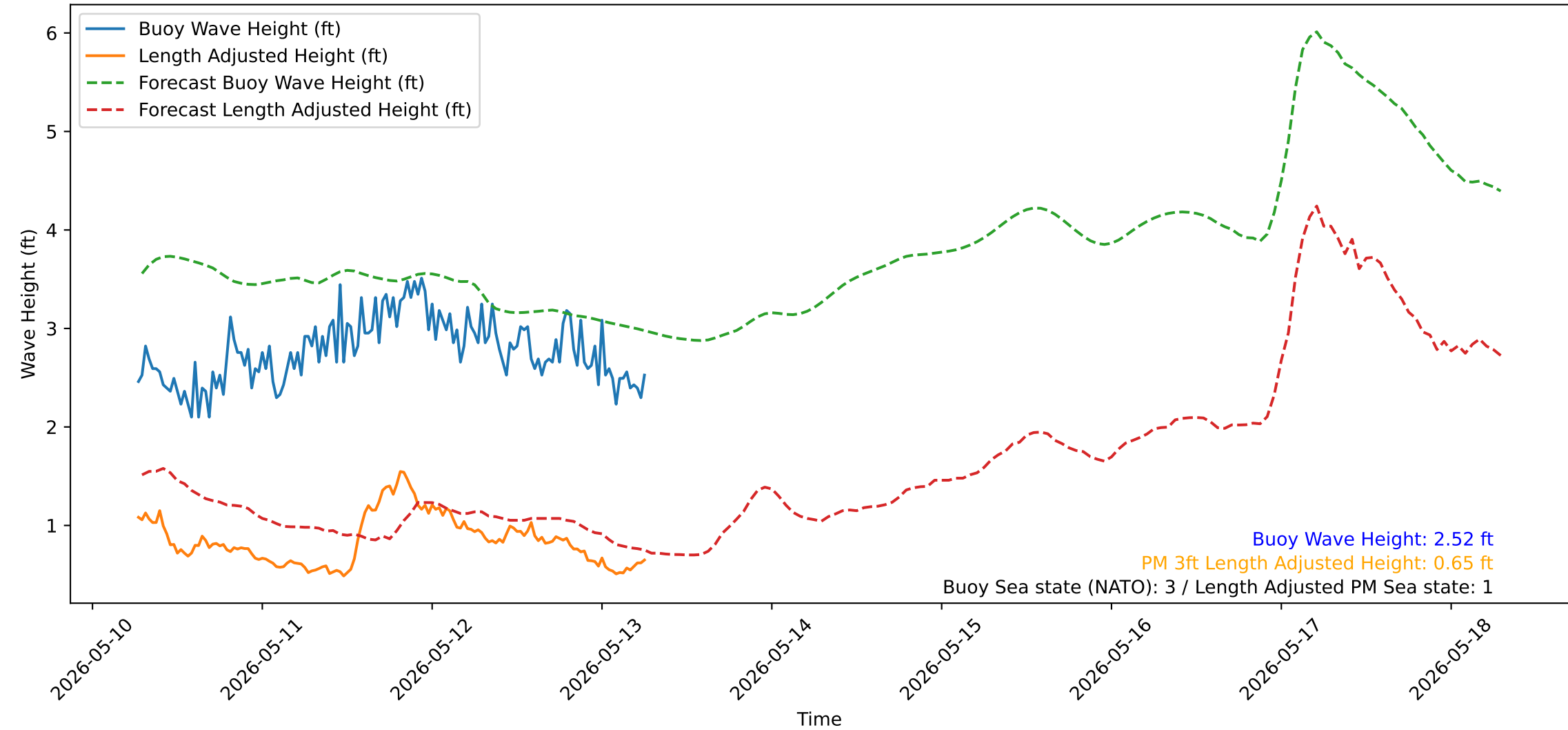
Wave Heights over Time for Green Beach at 2026-05-13 06:41:14
