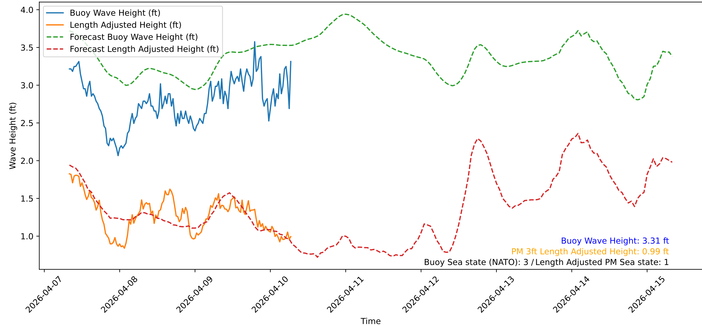
Wave Heights over Time for Red Beach at 2026-04-10 07:30:50
