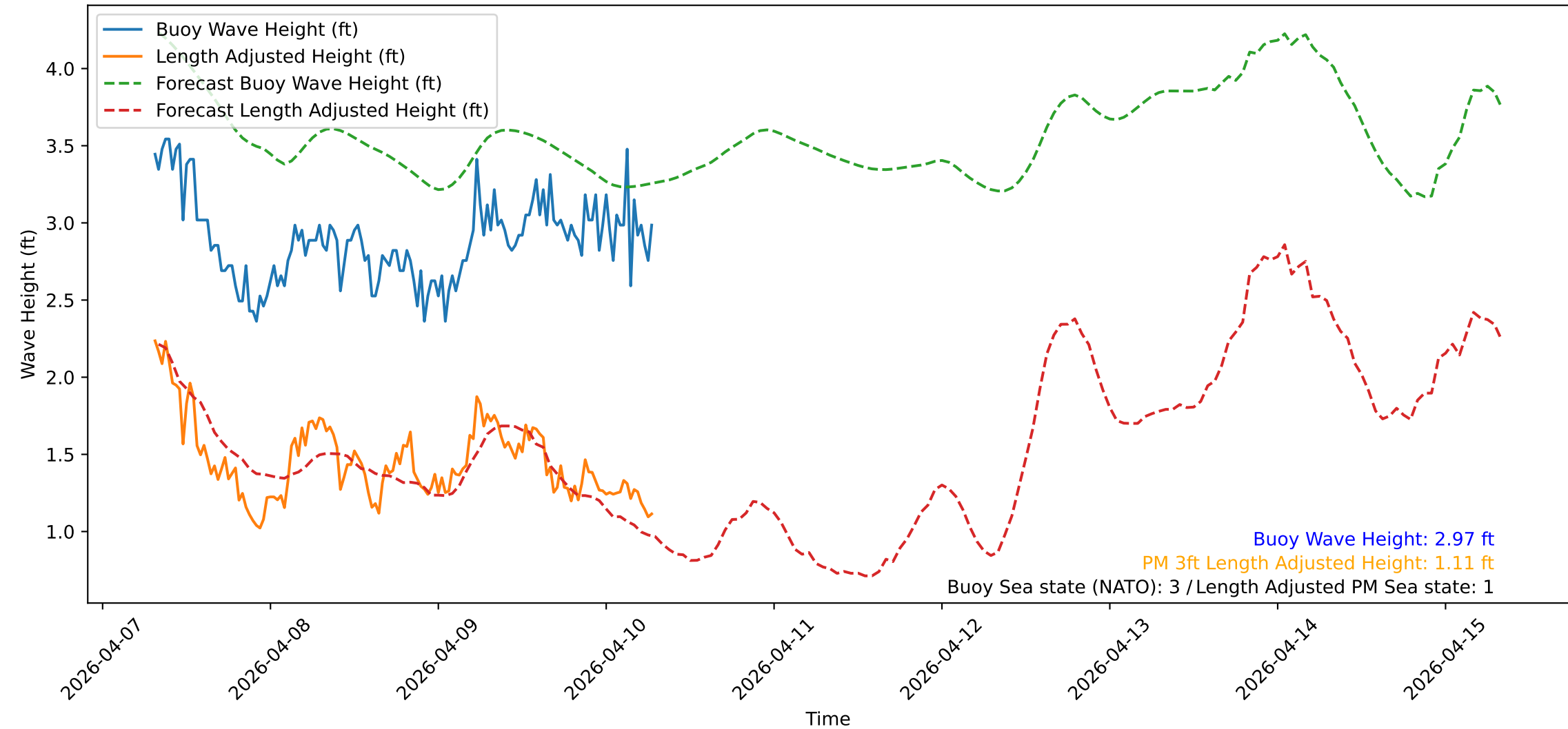
Wave Heights over Time for Green Beach at 2026-04-10 07:31:13
