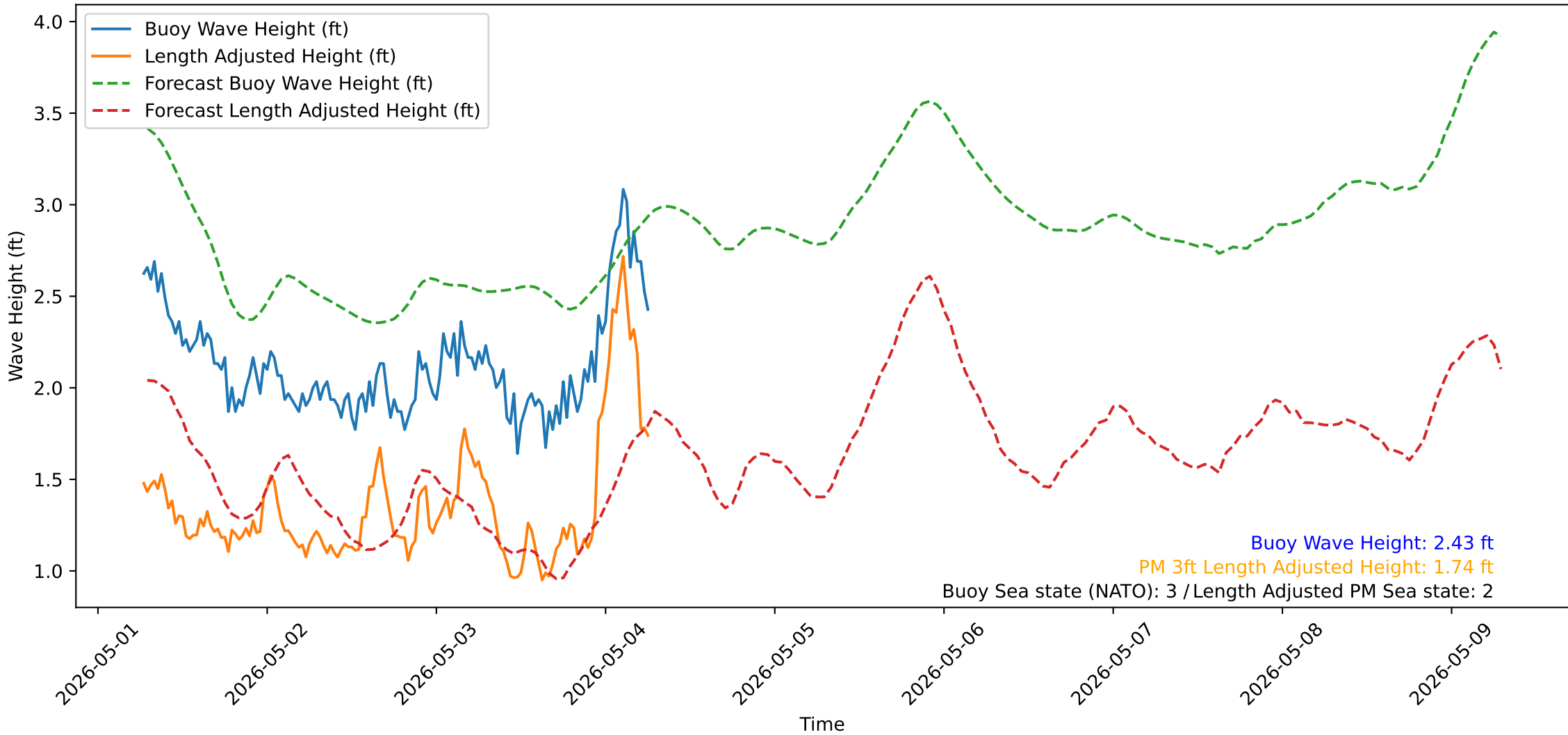
Wave Heights over Time for Oceanside Harbor at 2026-05-04 06:40:32
