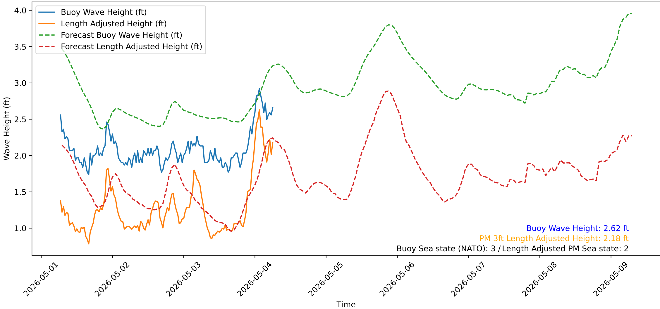
Wave Heights over Time for Green Beach at 2026-05-04 06:41:14
