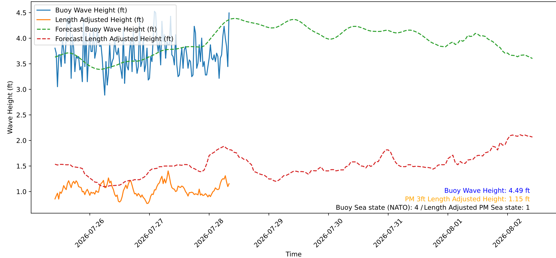
Wave Heights over Time for Red Beach at 2026-07-28 09:30:48
