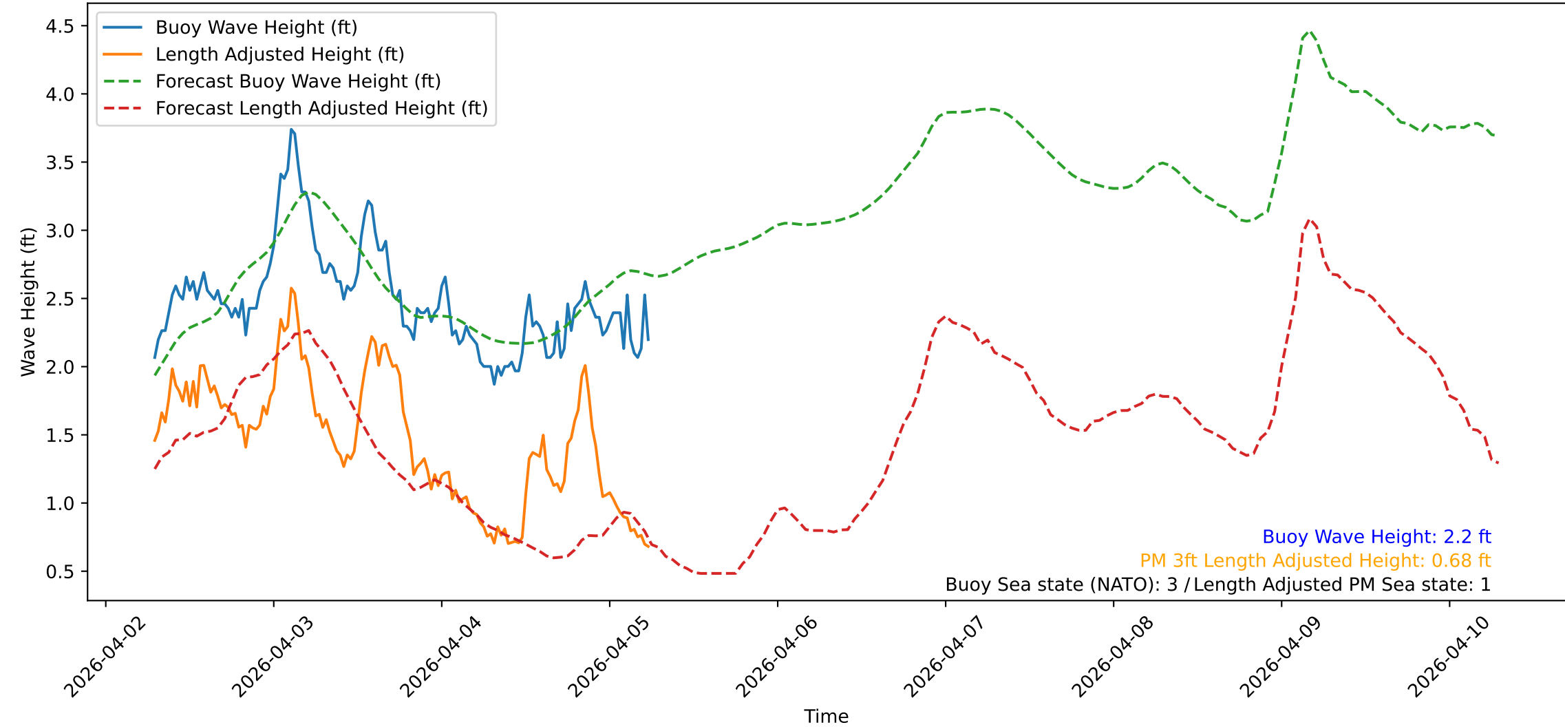
Wave Heights over Time for Red Beach at 2026-04-05 06:30:47
