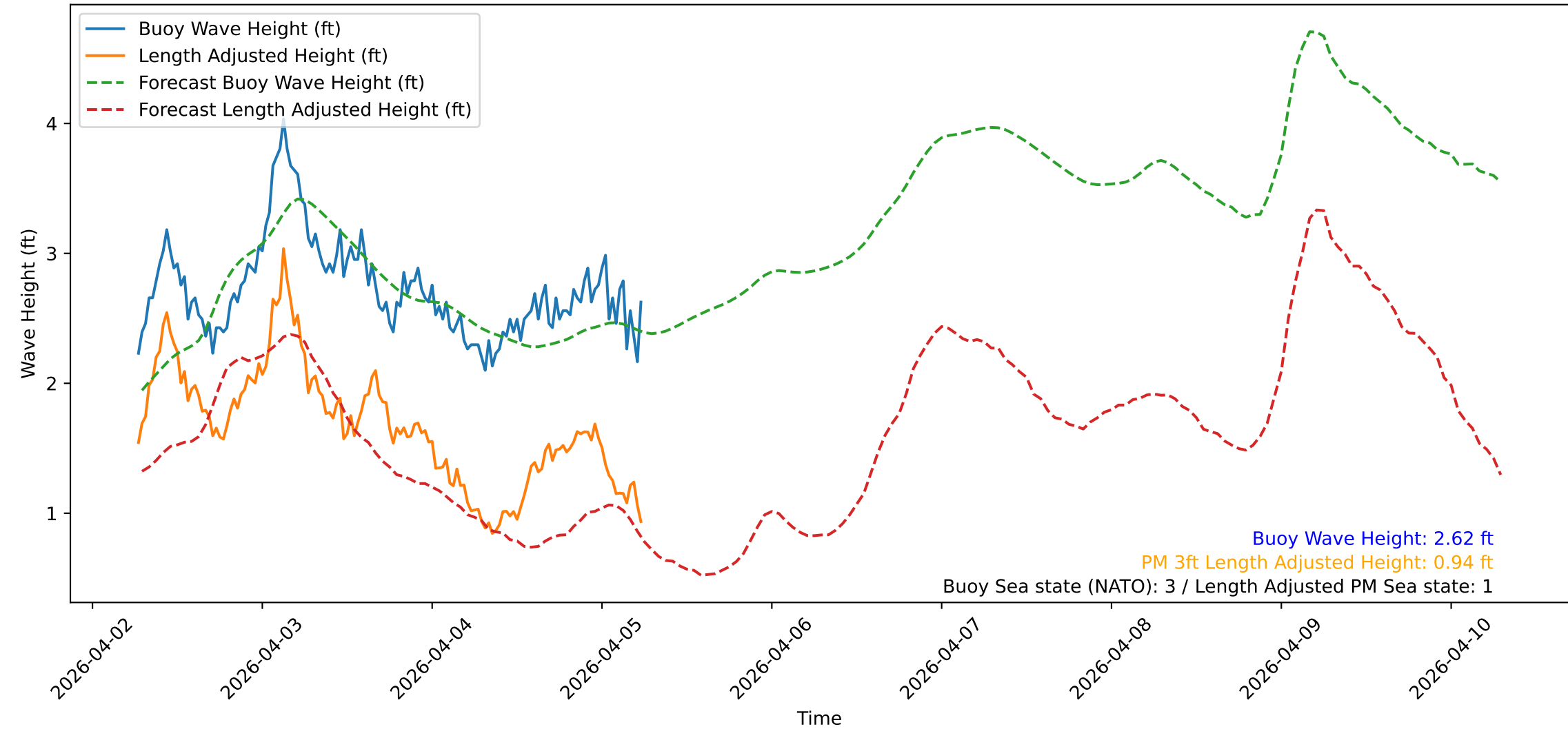
Wave Heights over Time for Oceanside Harbor at 2026-04-05 06:30:32
