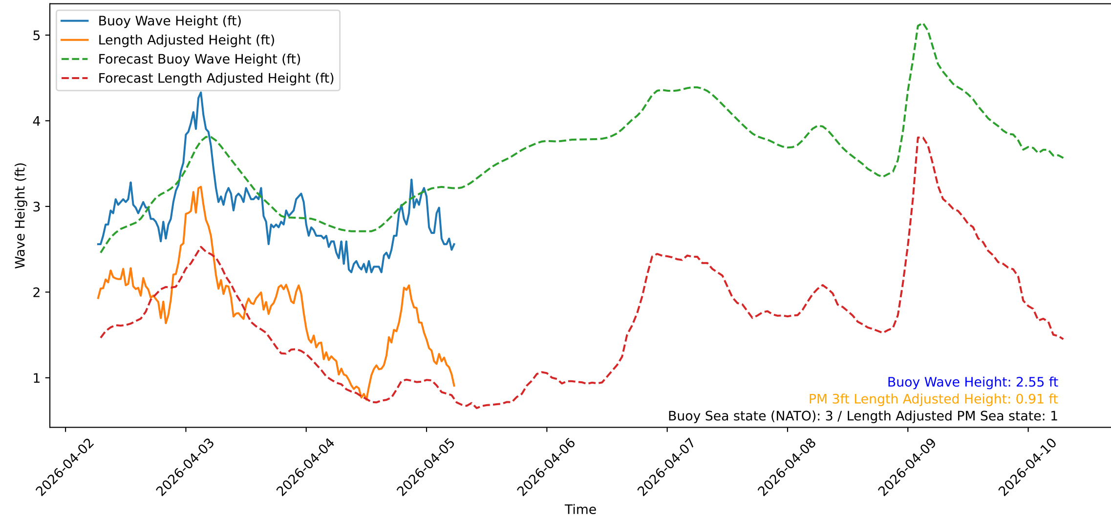
Wave Heights over Time for Green Beach at 2026-04-05 06:31:10
